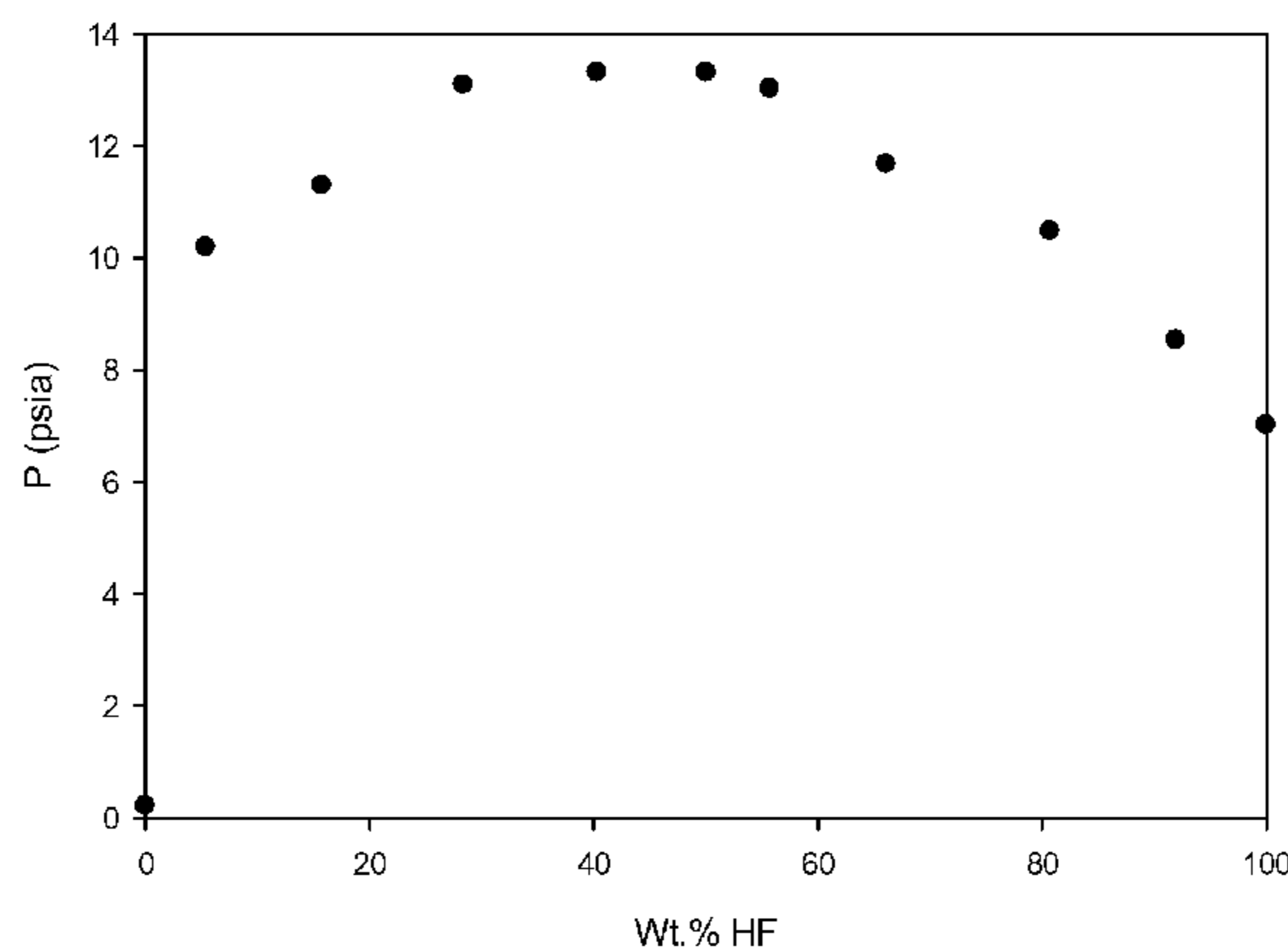
P-T-X 1230zd/HF at 0 C
