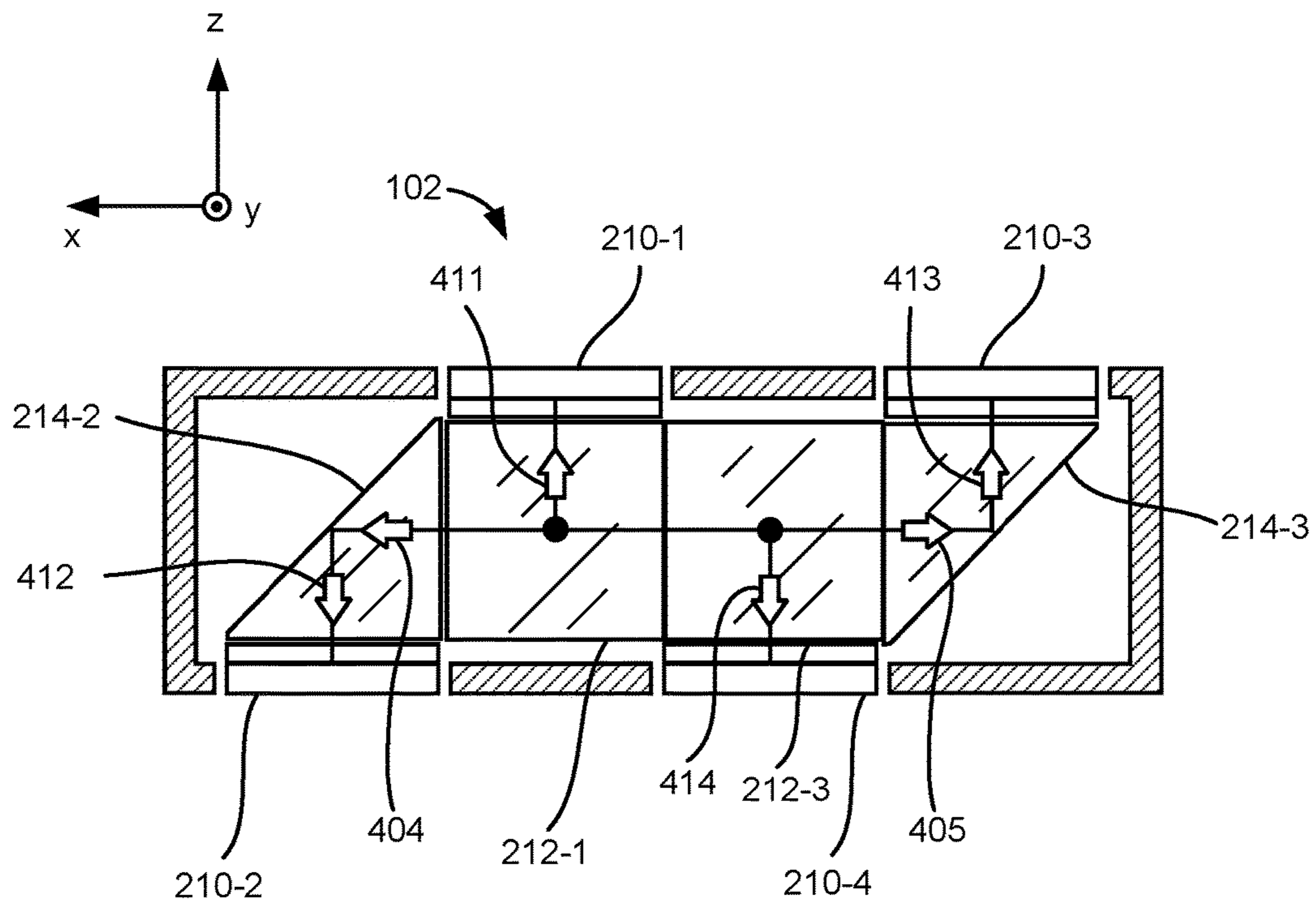
FRONT VIEW
