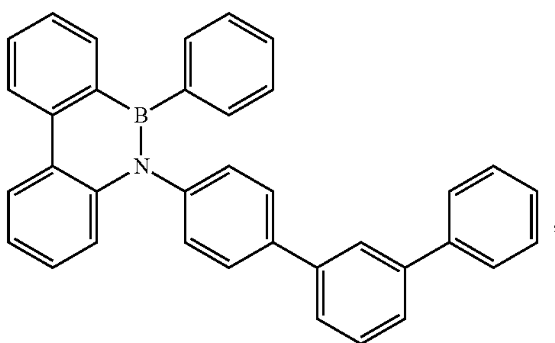
Compound B-60
