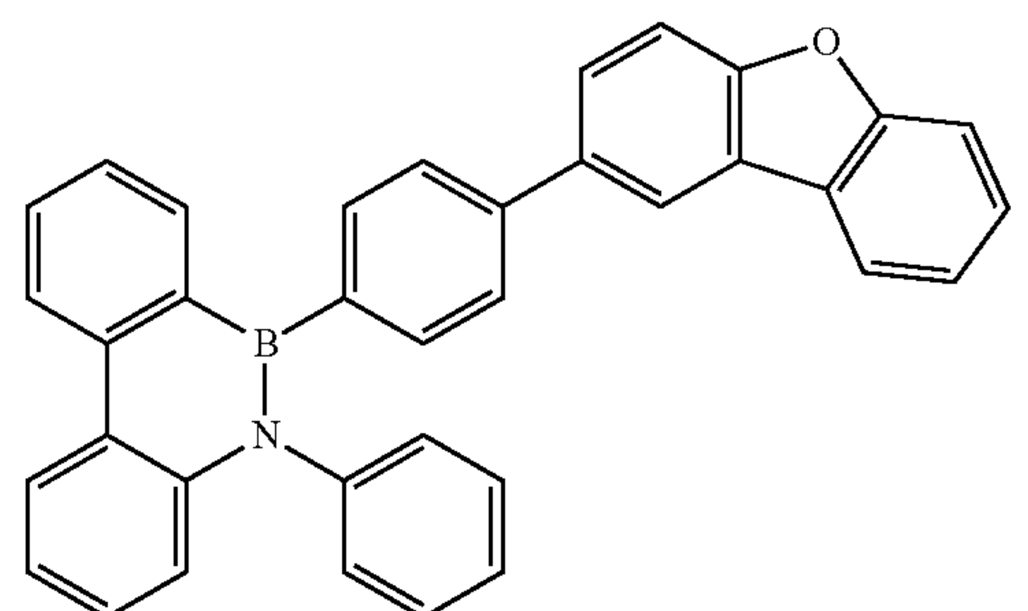
Compound B-47
