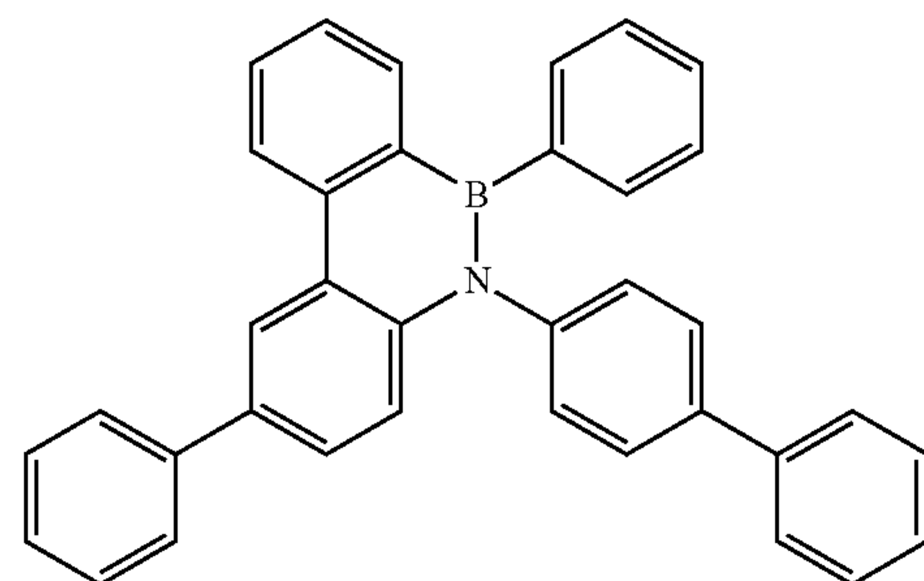
Compound B-17
