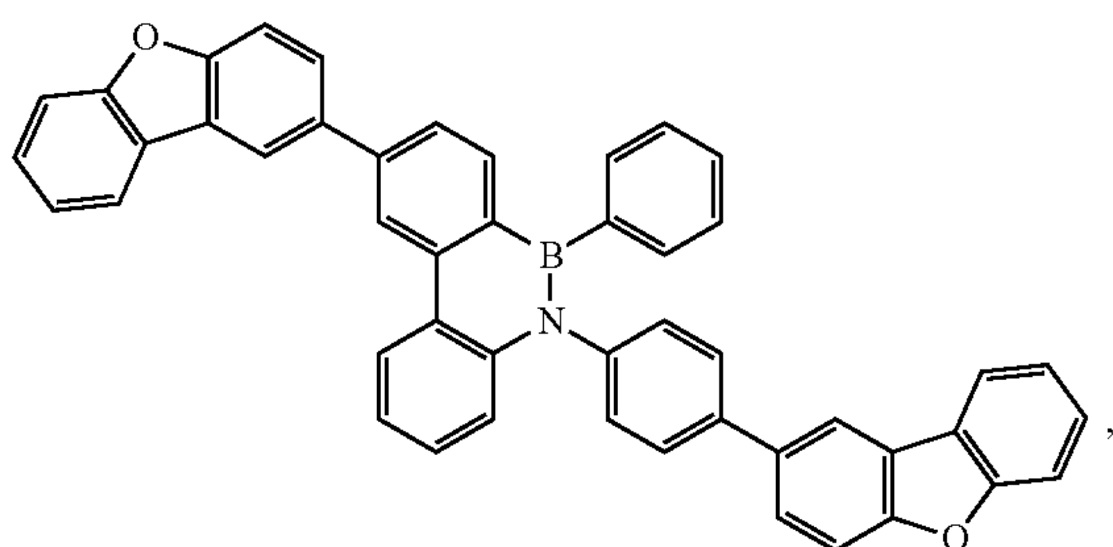
Compound B-52
