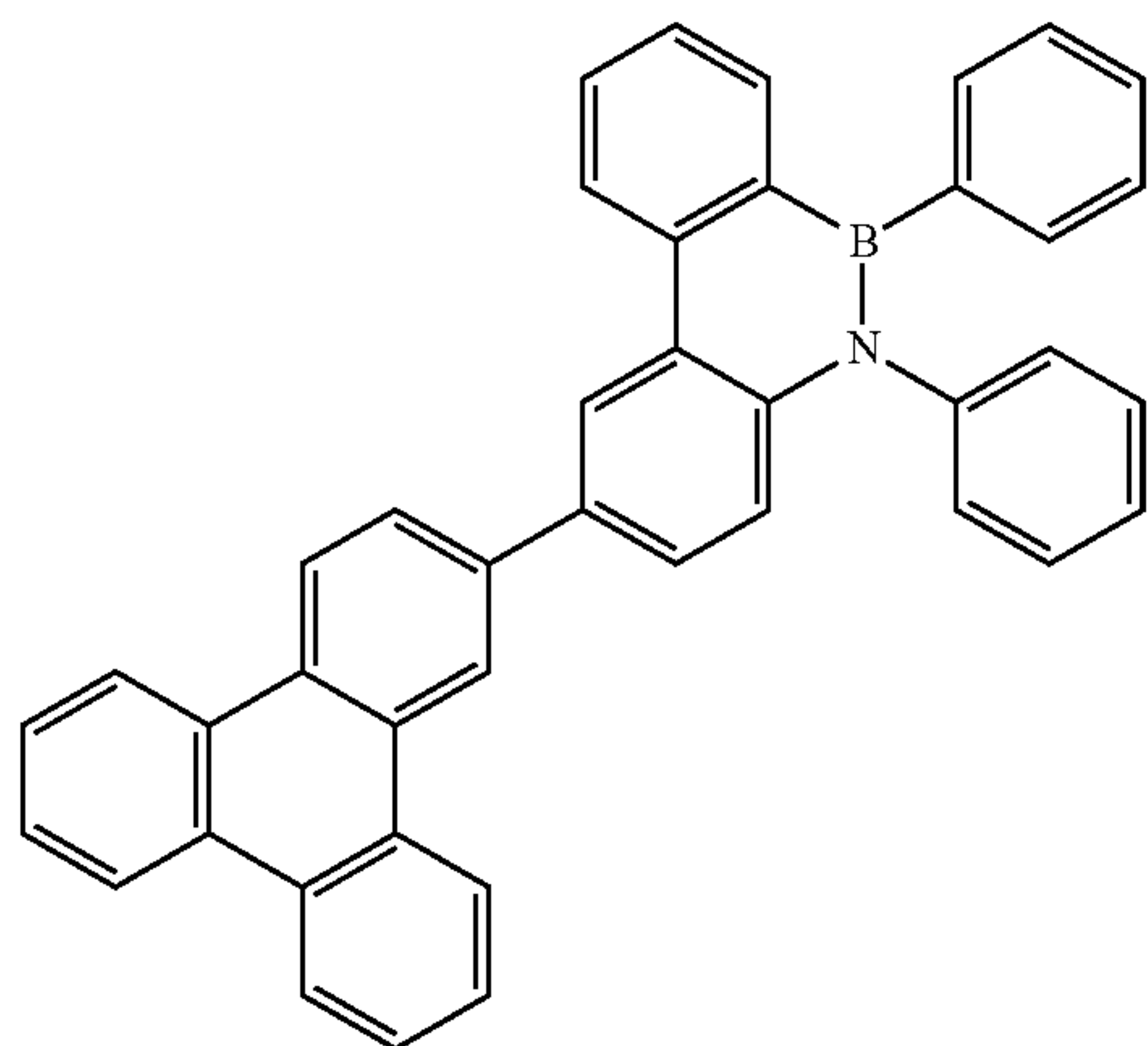
Compound B-64
