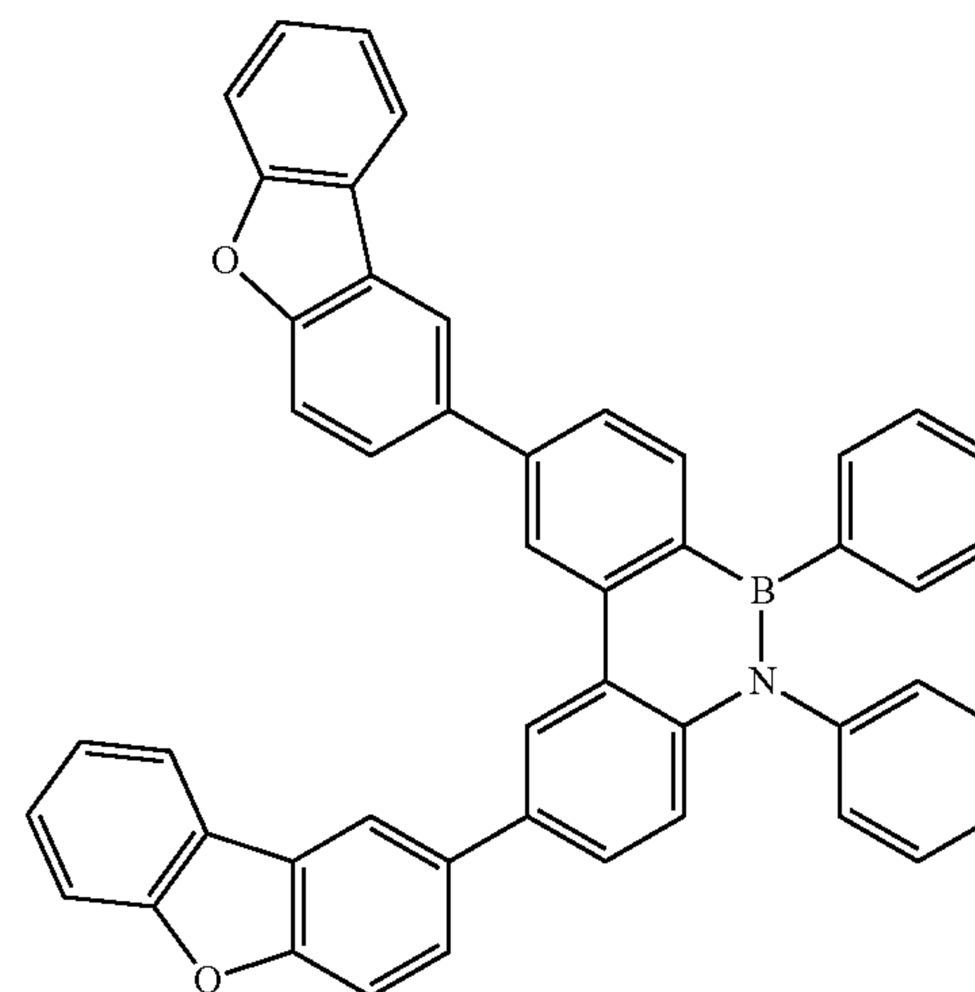
Compound B-51
