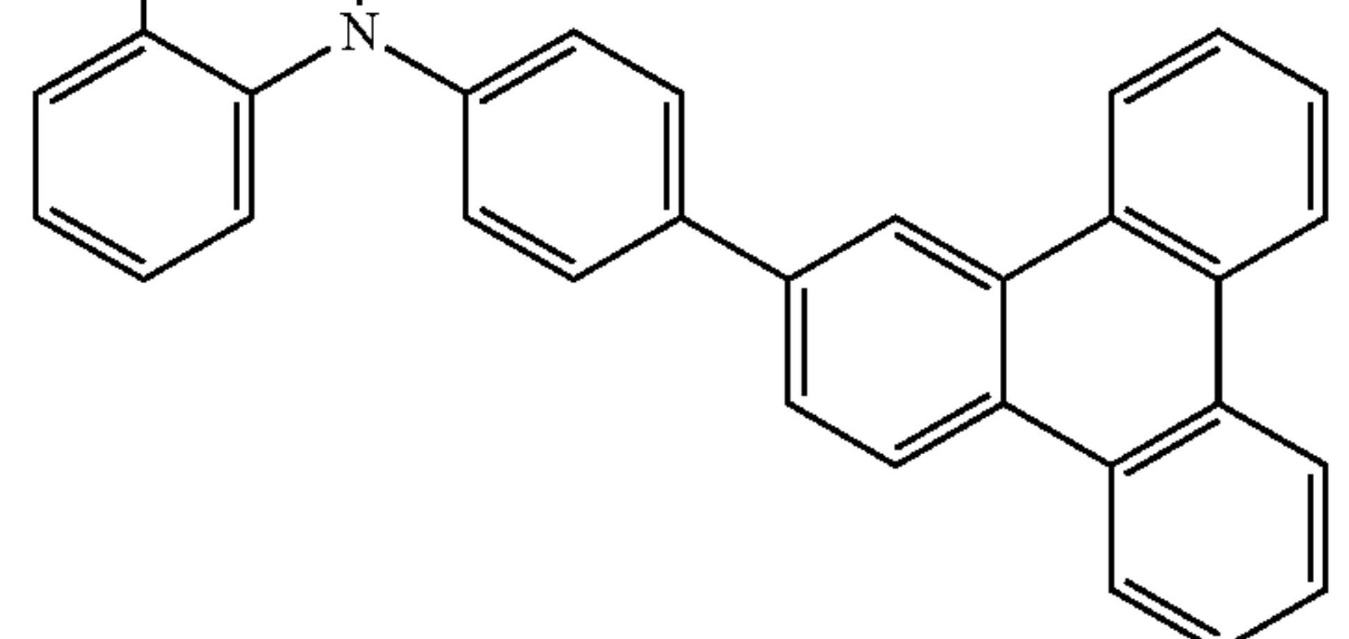
Compound B-78
