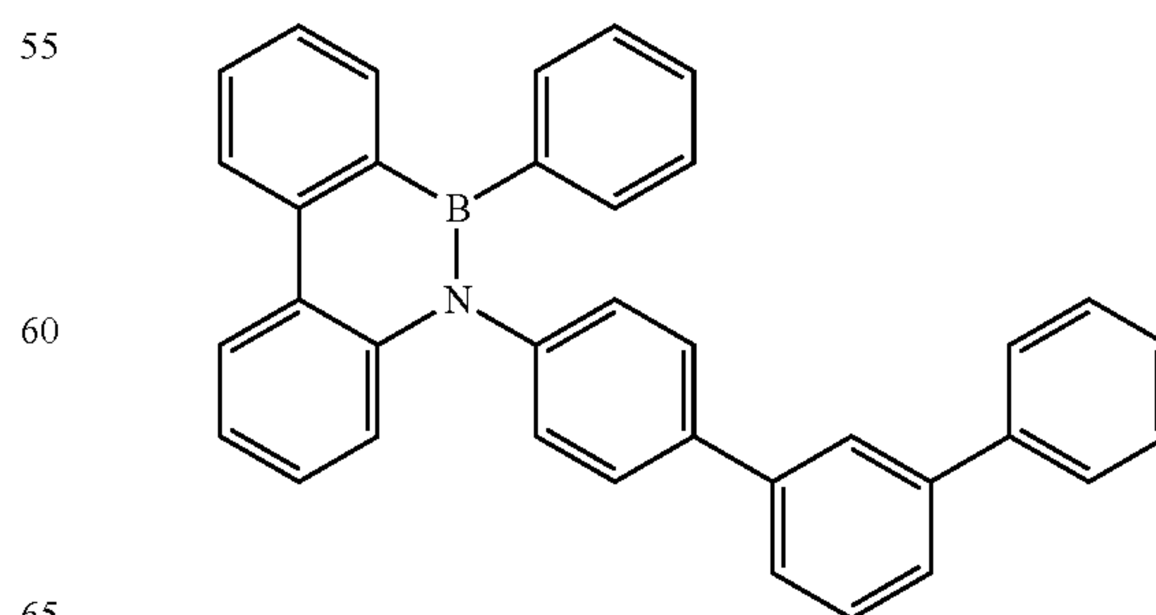
Compound B-60
