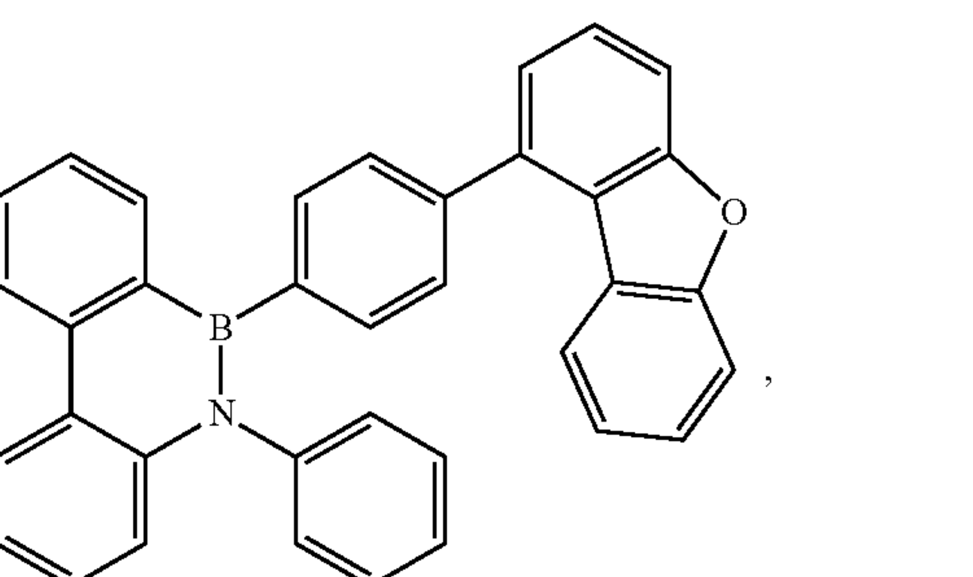
Compound B-50
