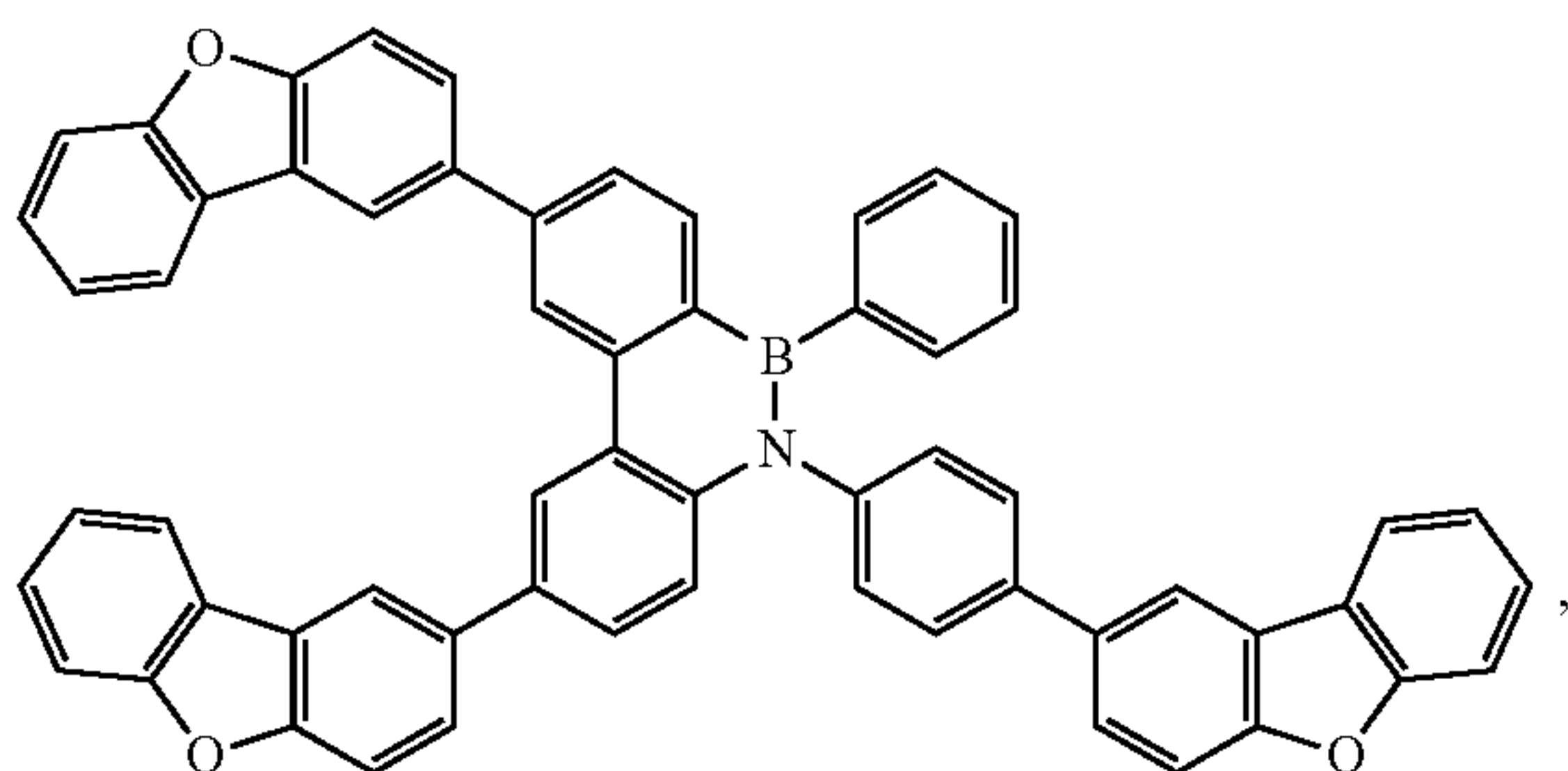
Compound B-53
