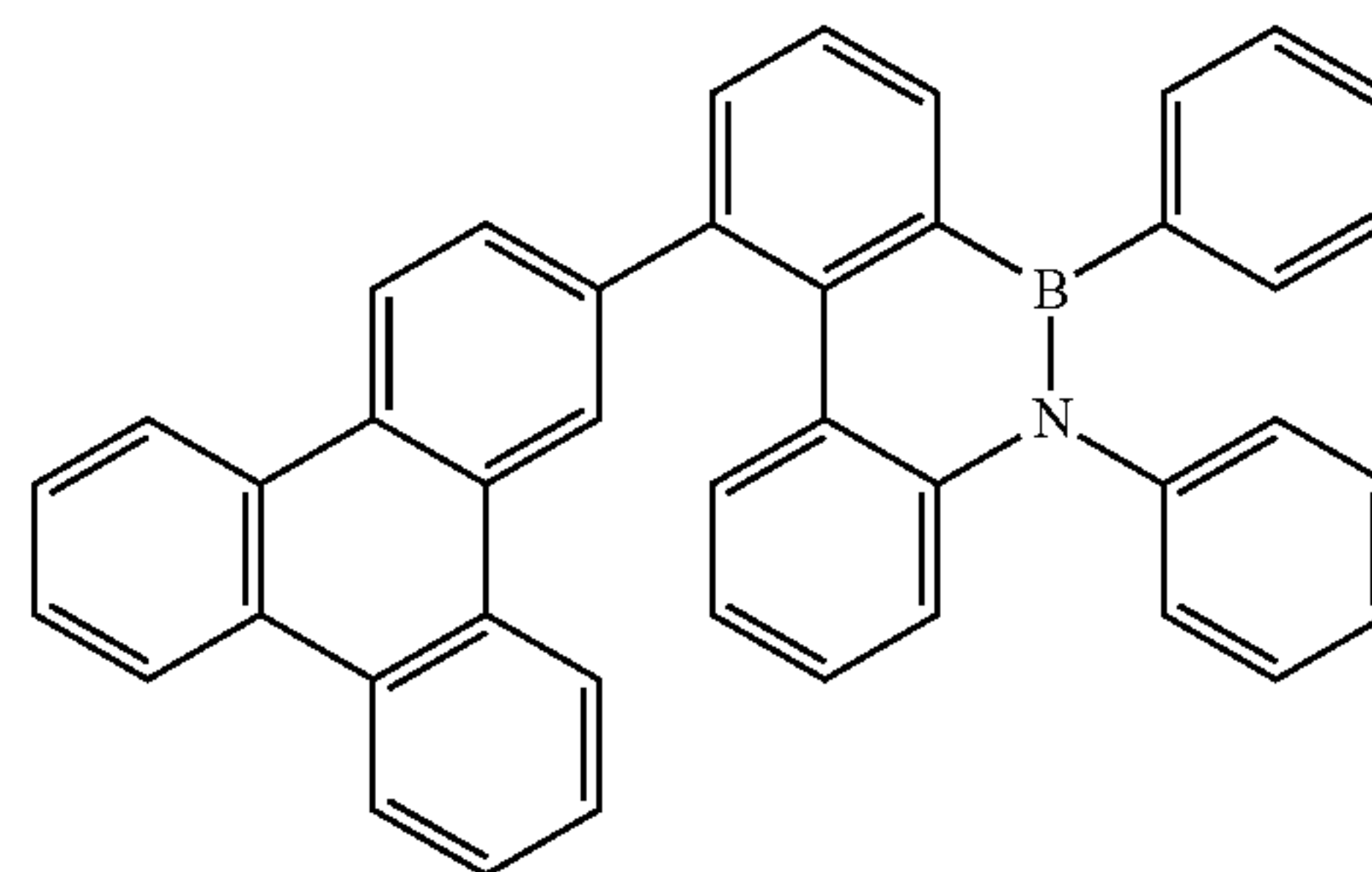
Compound B-67
