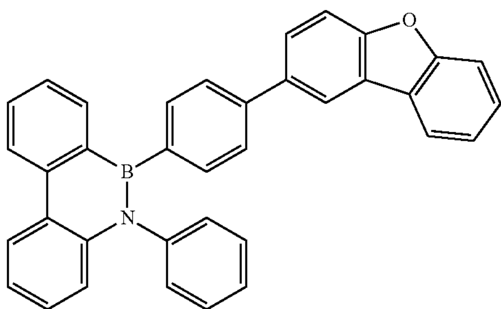
Compound B-47
