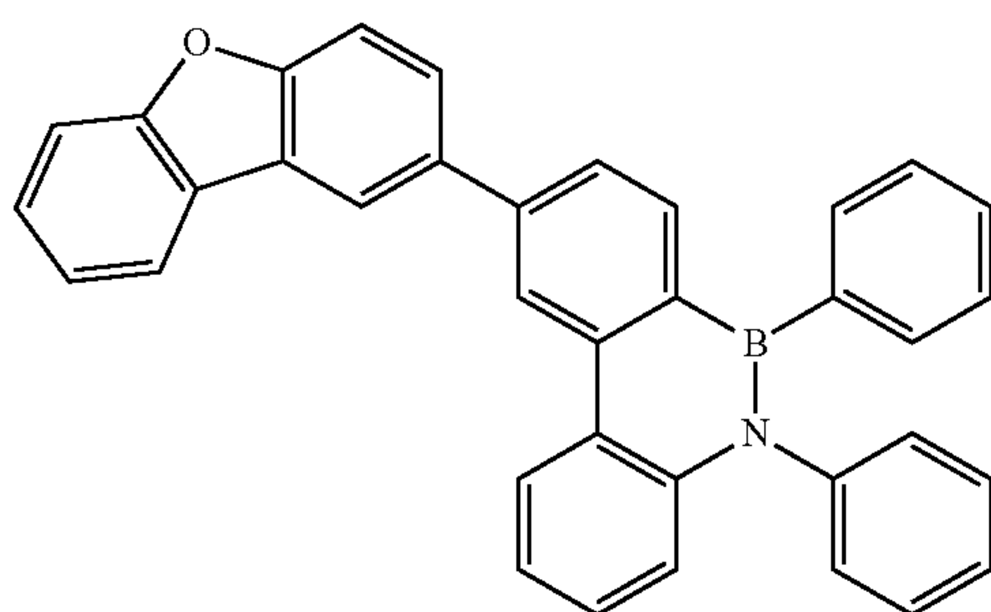
Compound B-45
