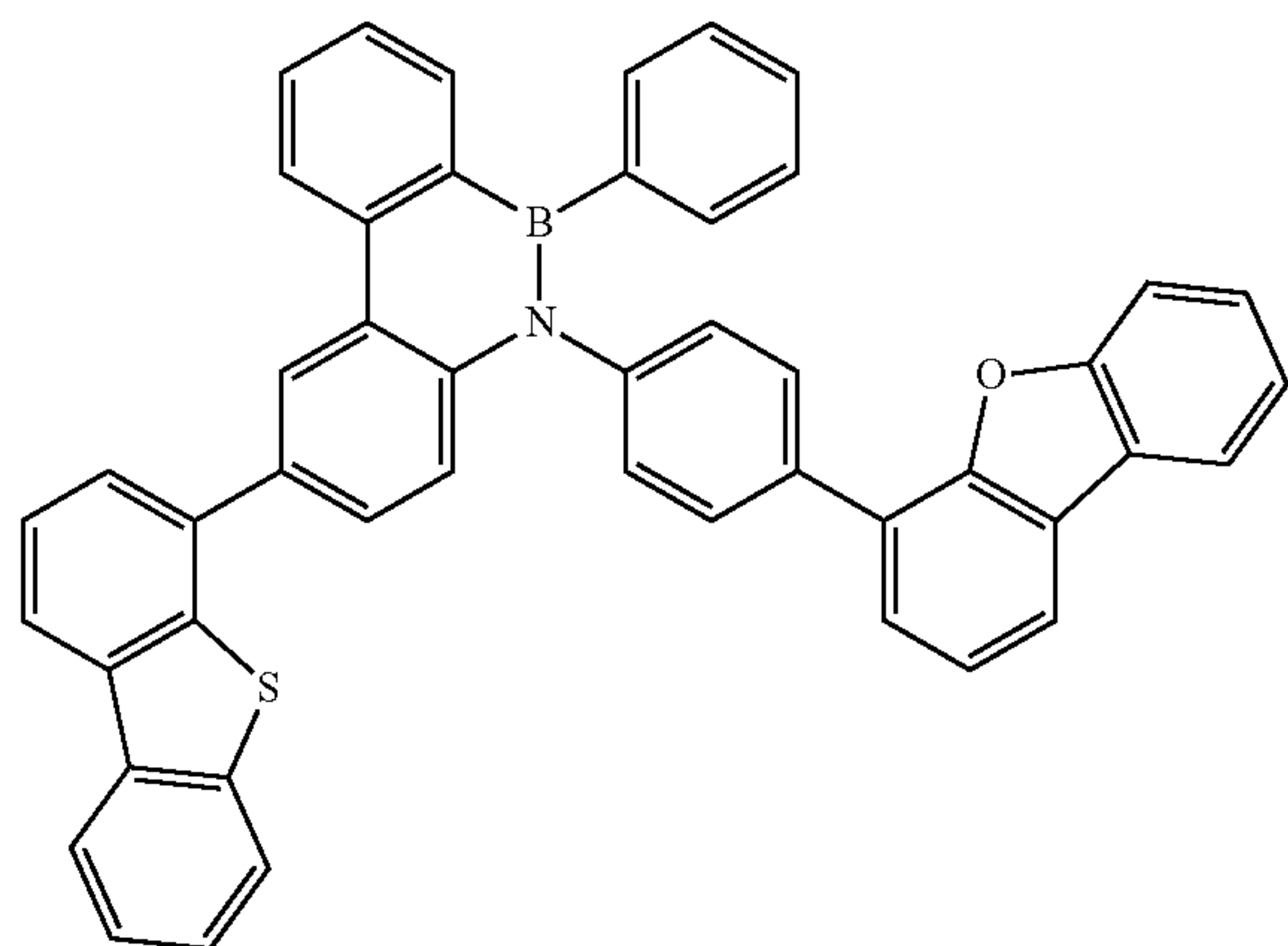
Compound B-41
