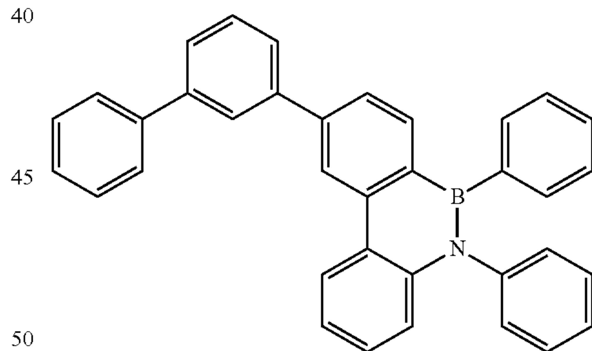
Compound B-55
