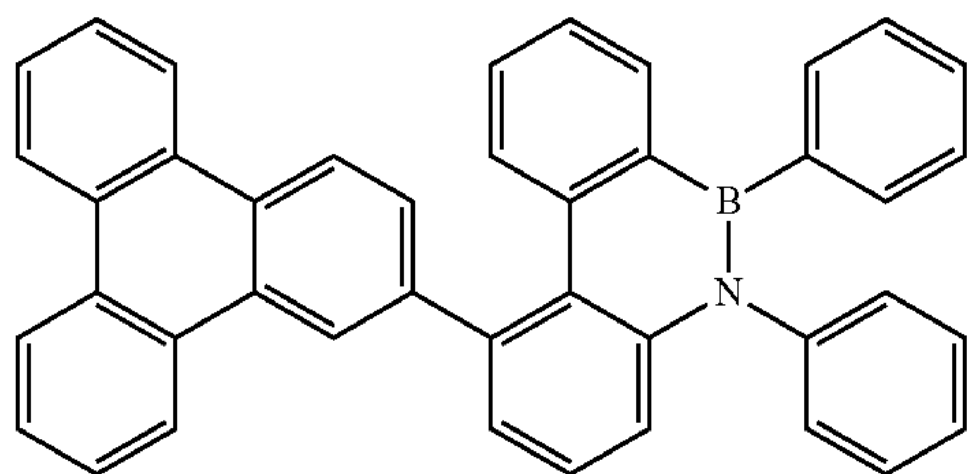
Compound B-63
