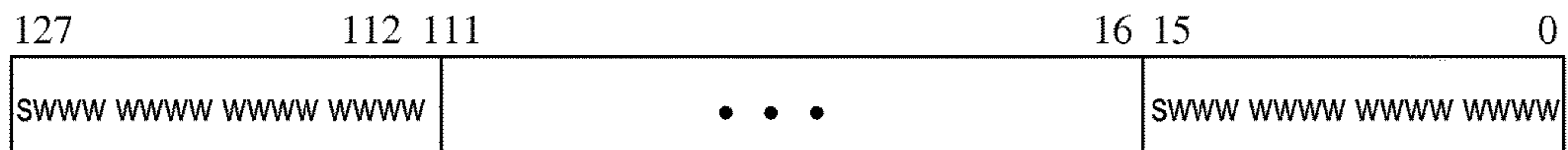
347 — SIGNED PACKED WORD REPRESENTATION
