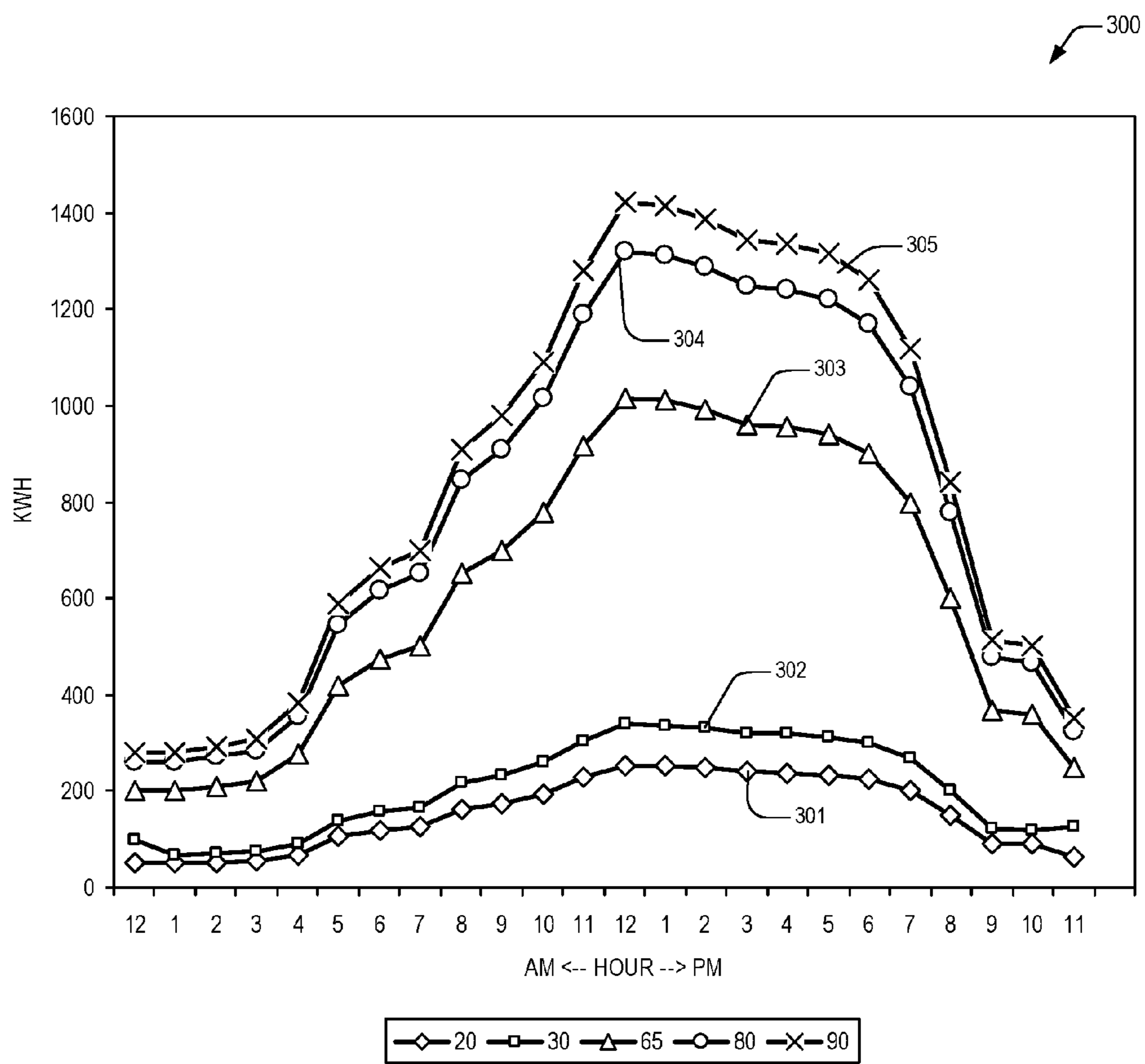
HOURLY FACILITY ENERGY CONSUMPTION PROFILES
