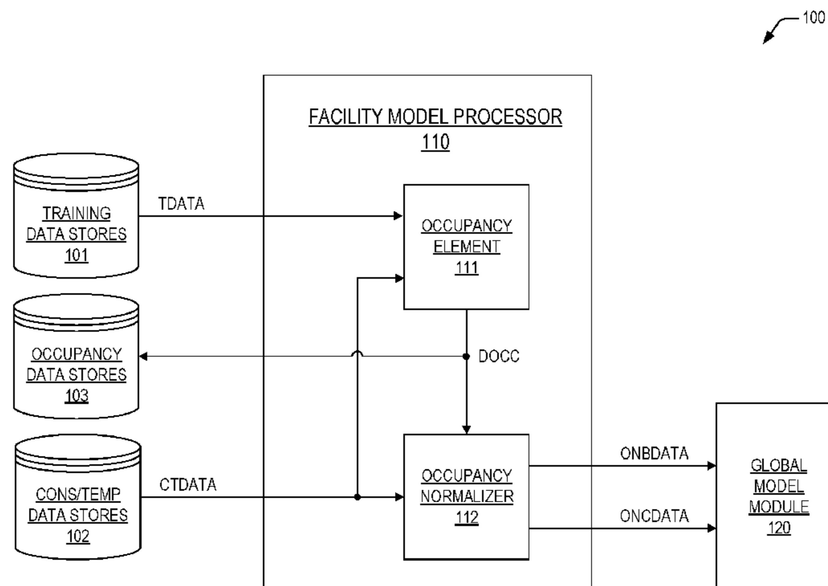
OCCUPANCY DETERMINATION SYSTEM
