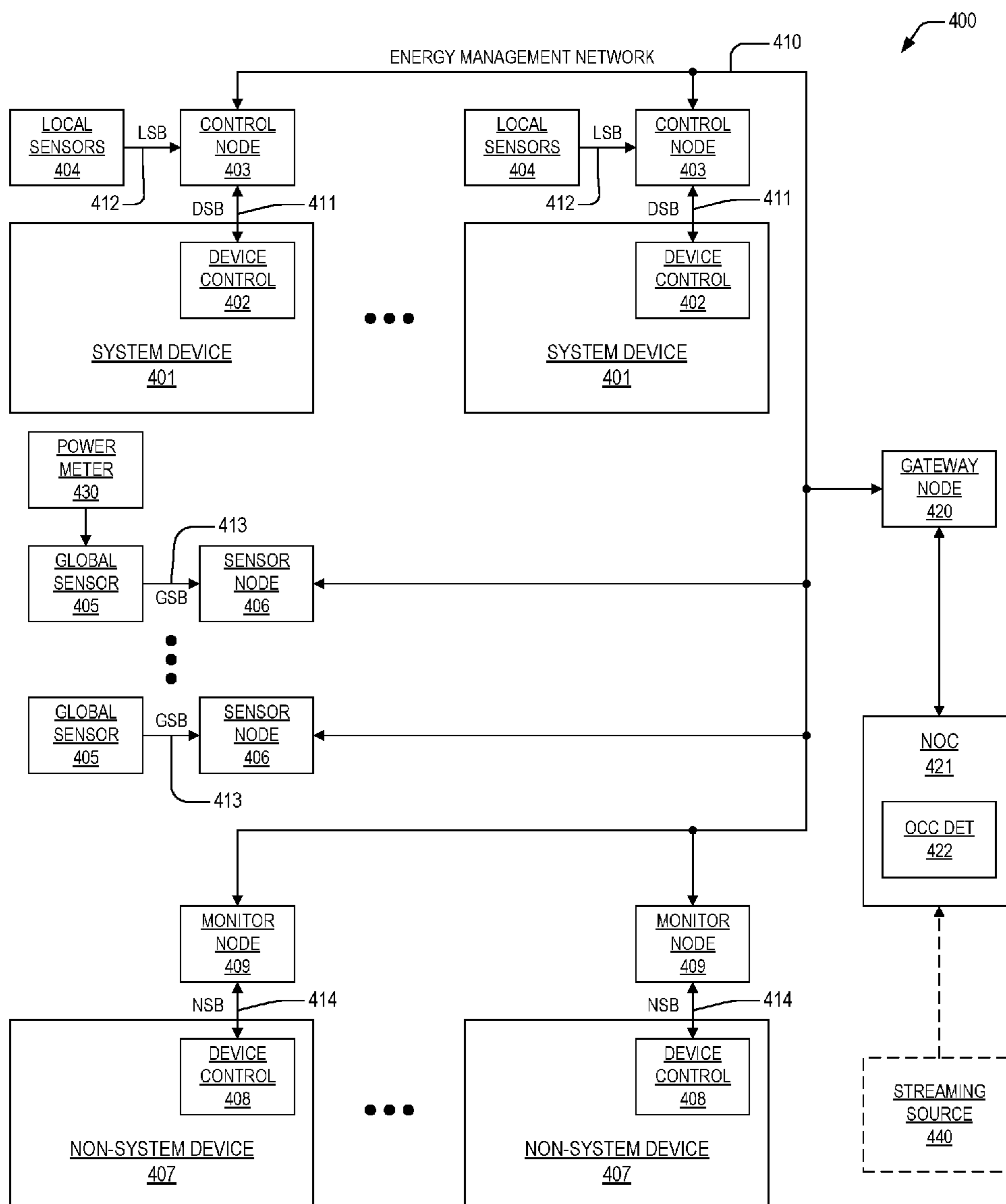
OCCUPANCY BASED ENERGY CONSUMPTION MANAGEMENT SYSTEM
