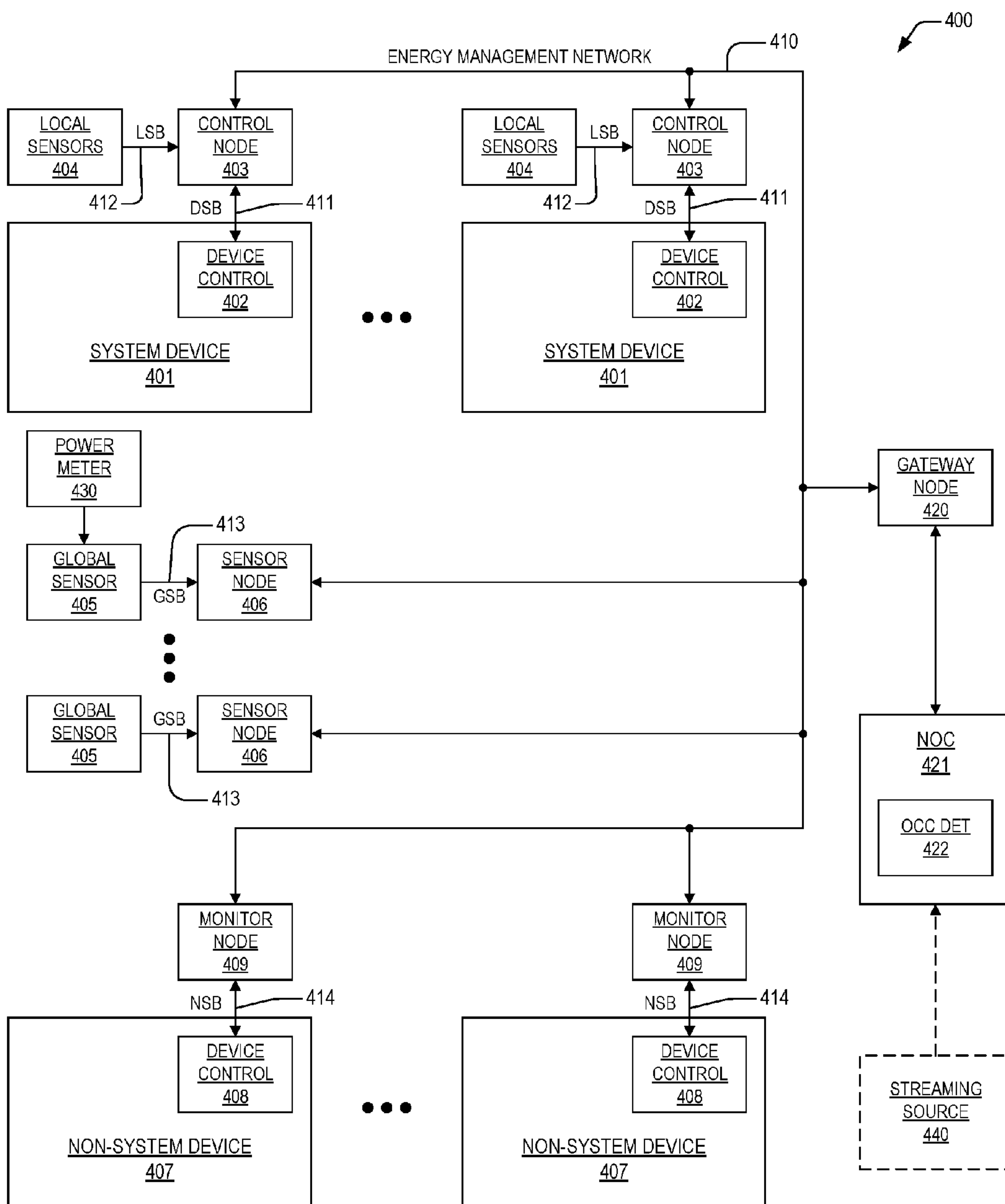
OCCUPANCY BASED ENERGY CONSUMPTION MANAGEMENT SYSTEM
