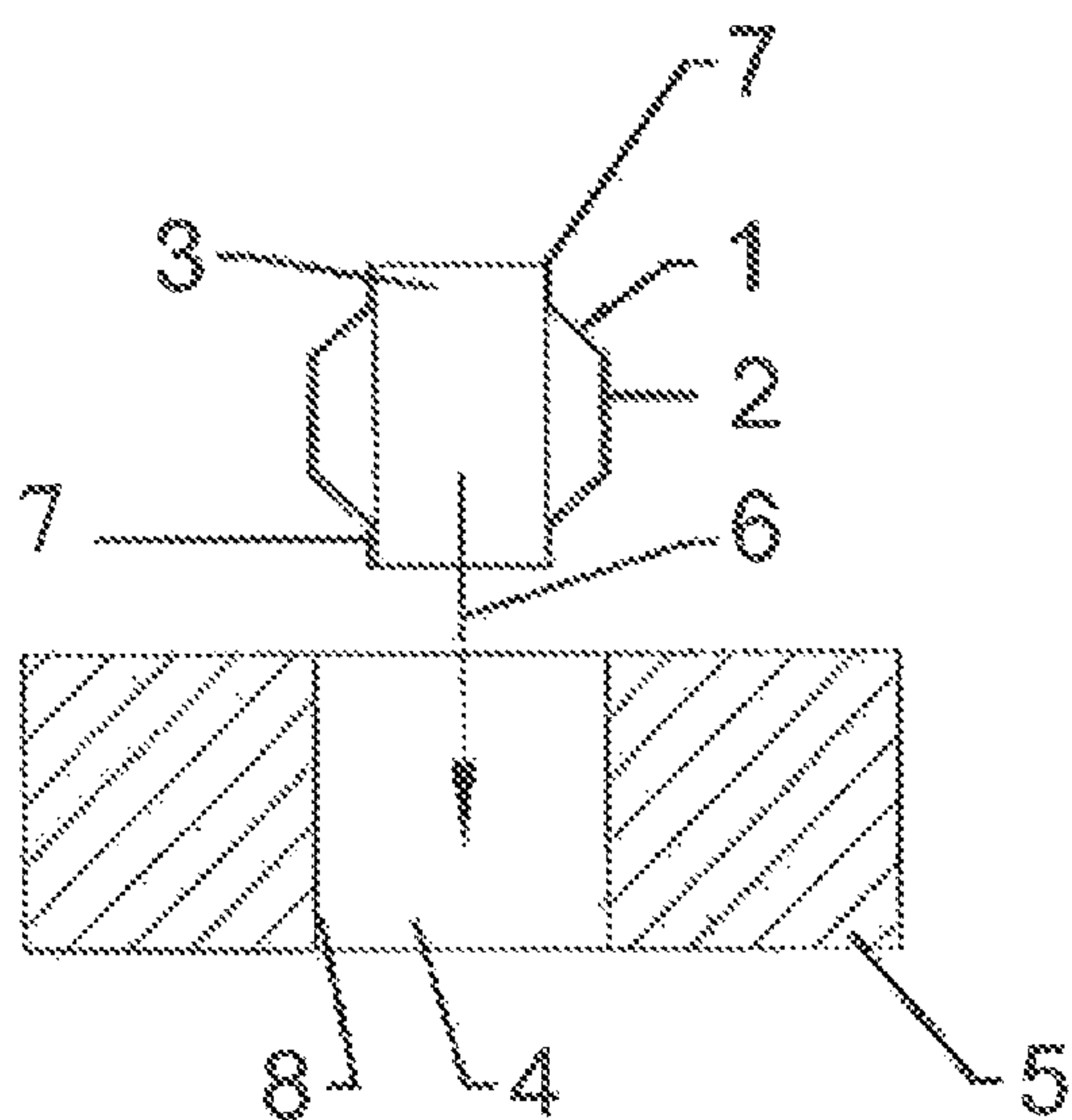
Fig.1 (Prior art)
