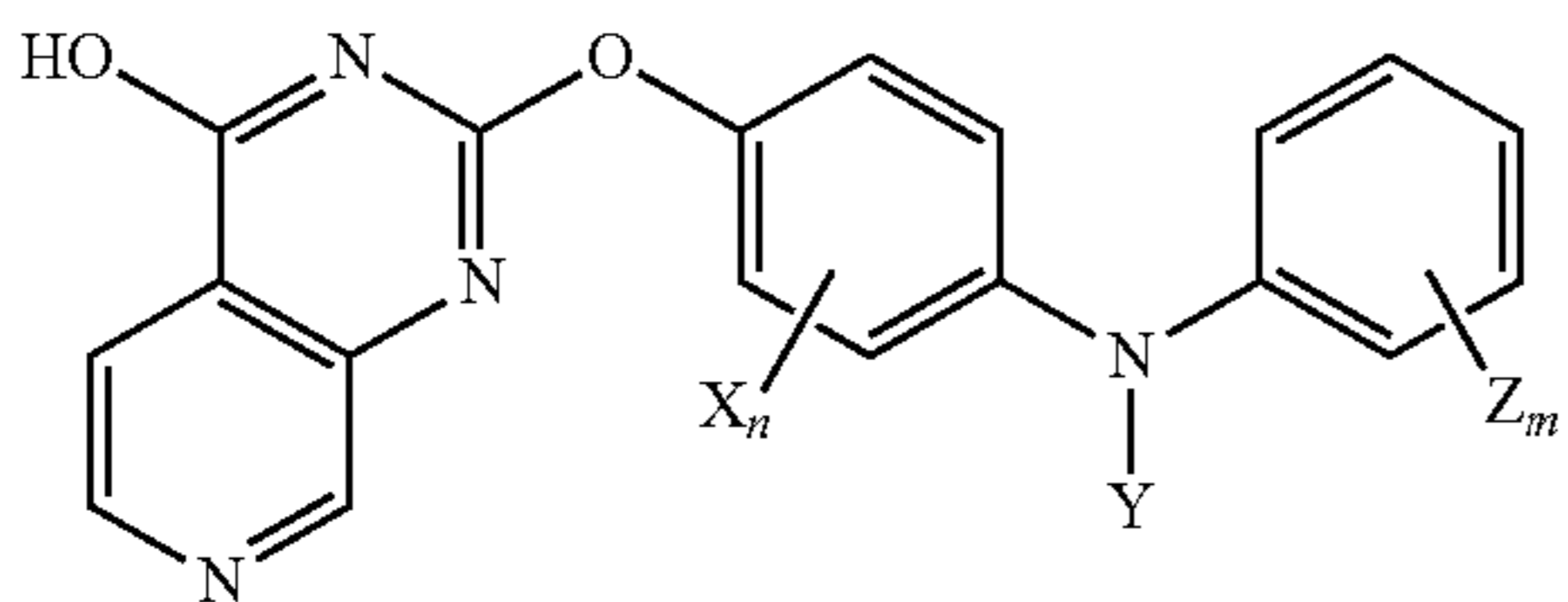
Formula (III)
