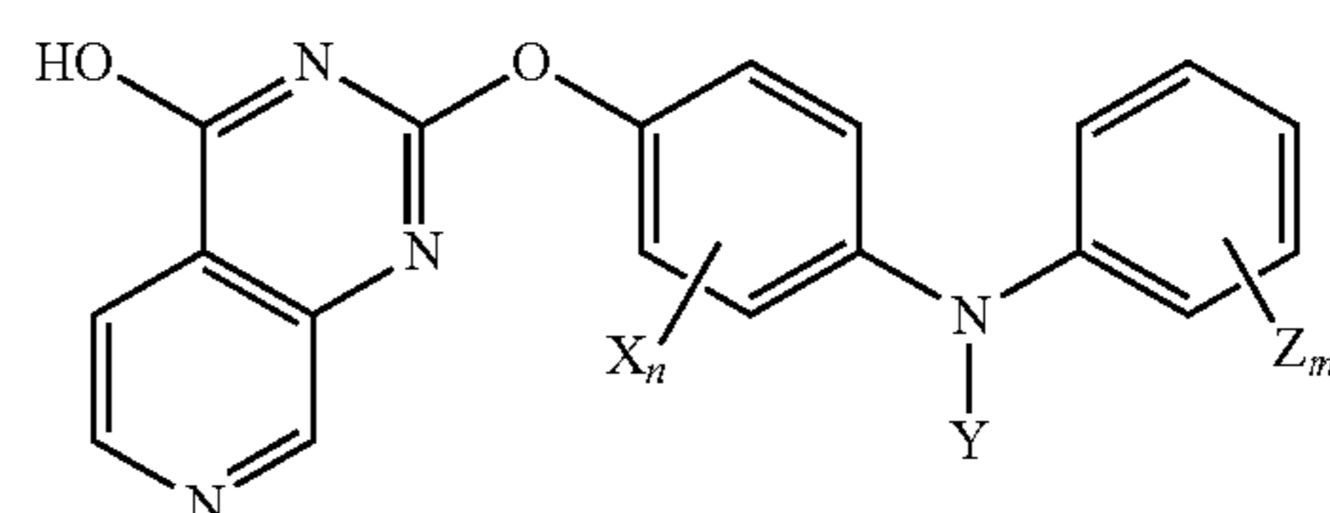
Formula (III)
