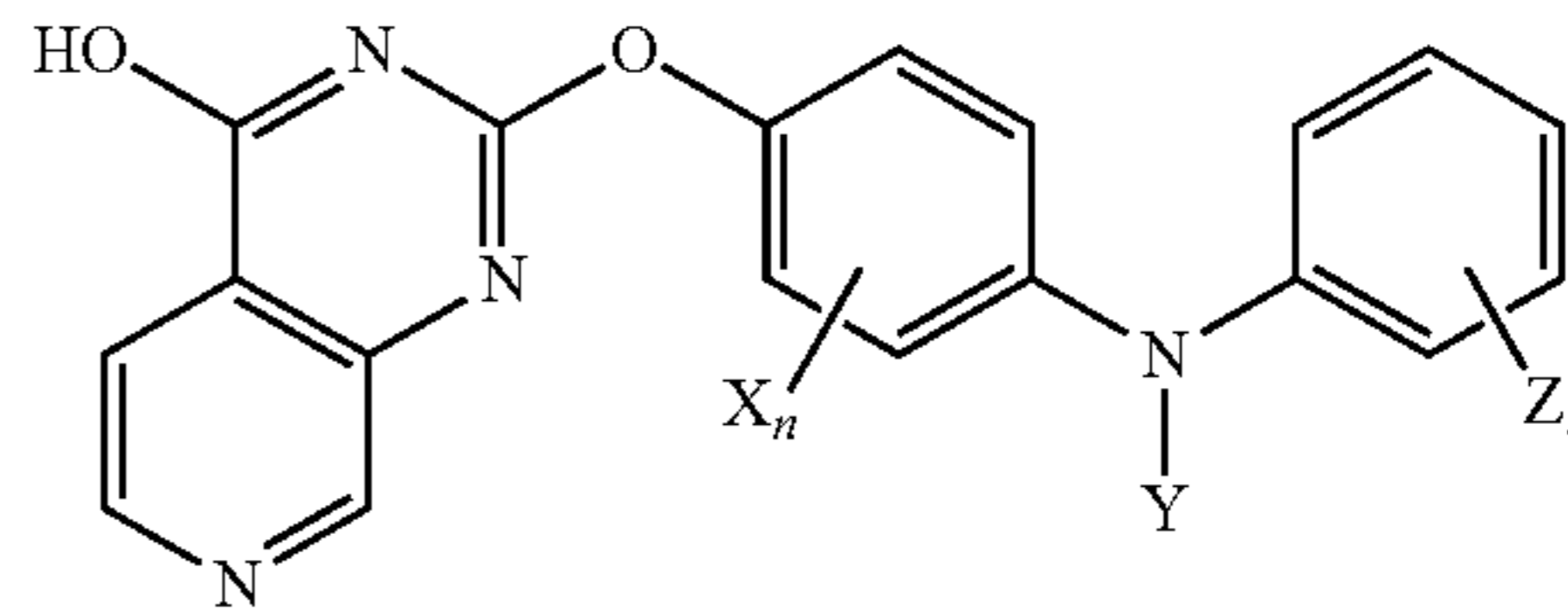
Formula (IIIa)
