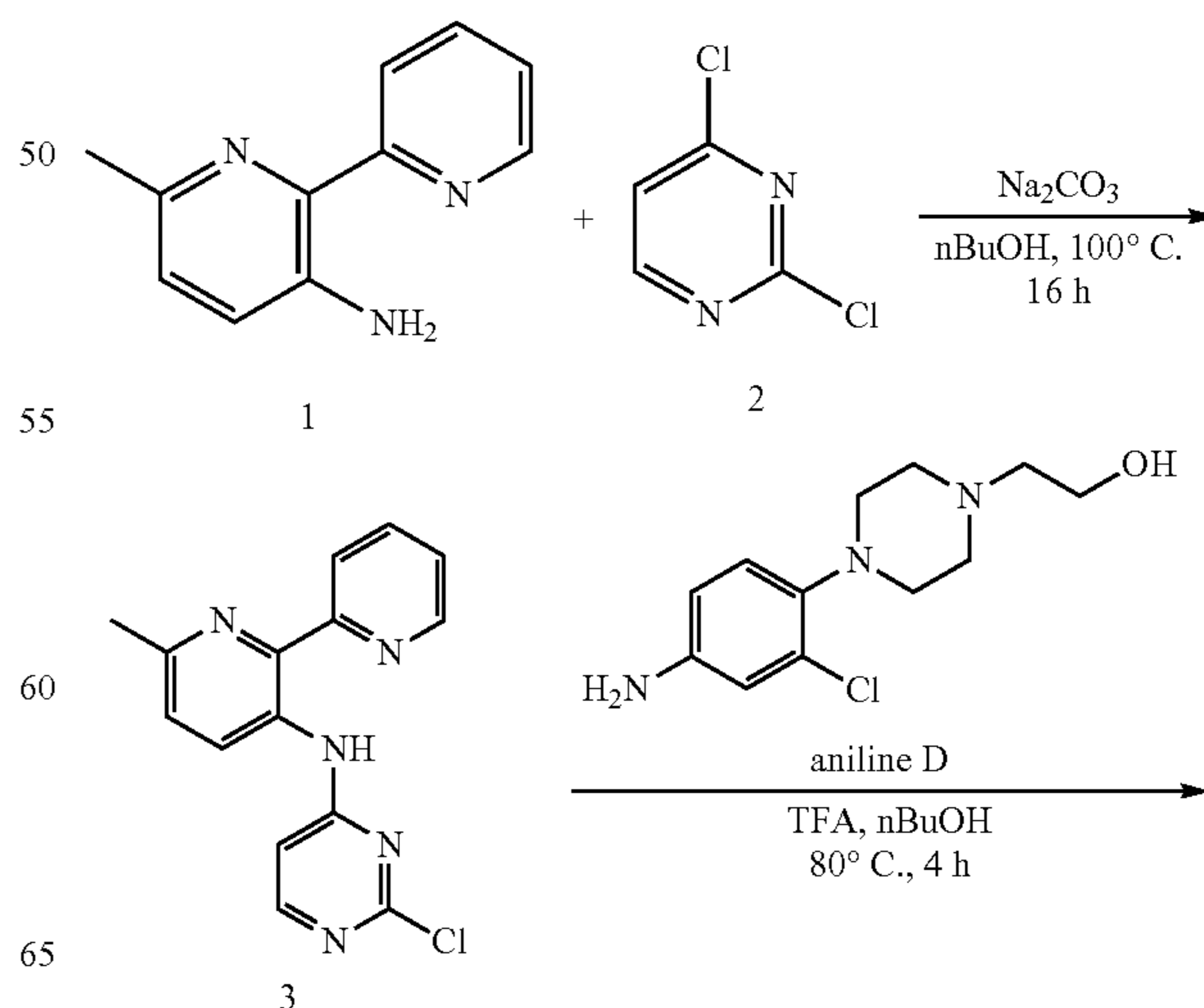
Scheme 13
