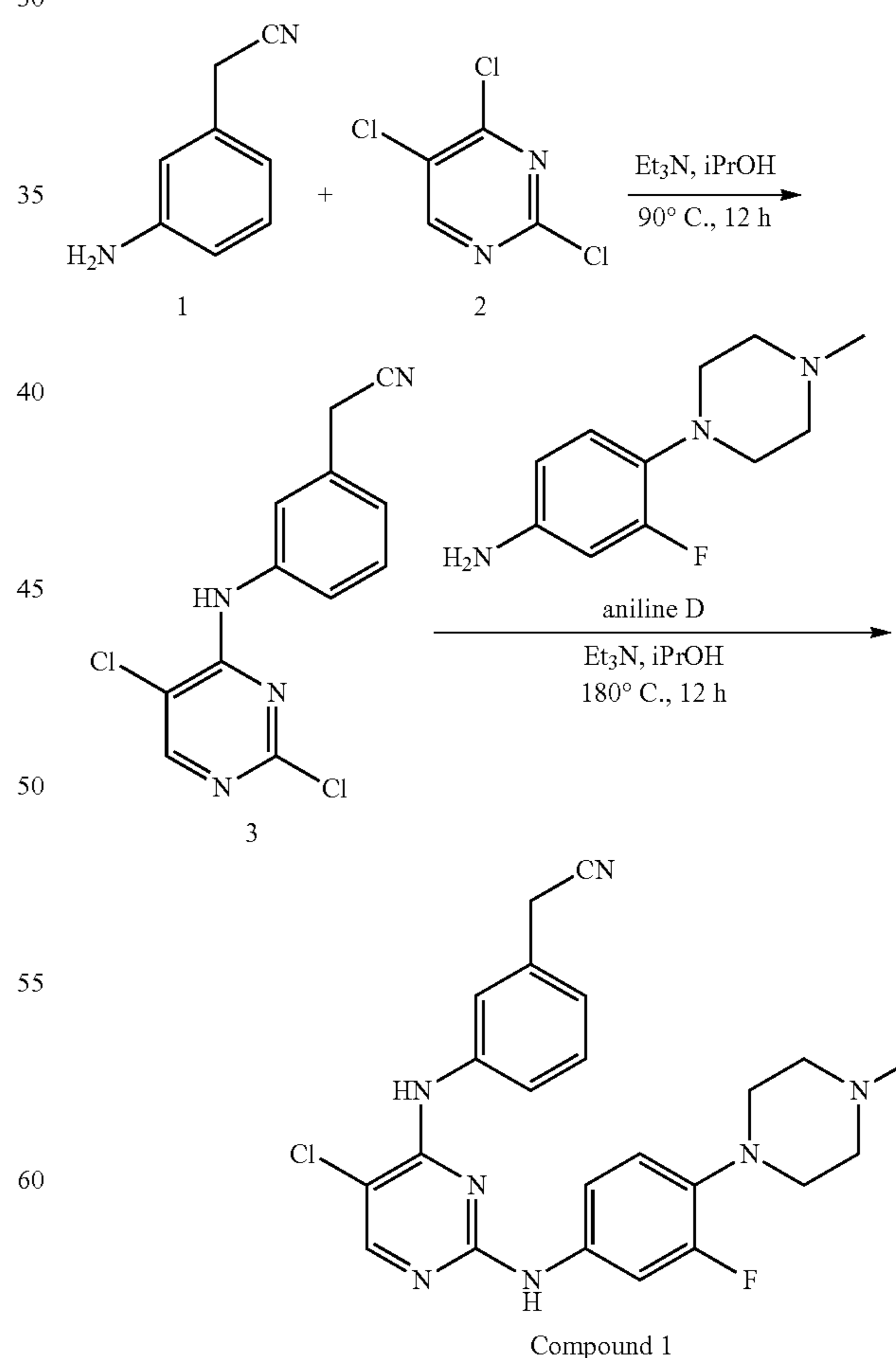
Scheme 3
