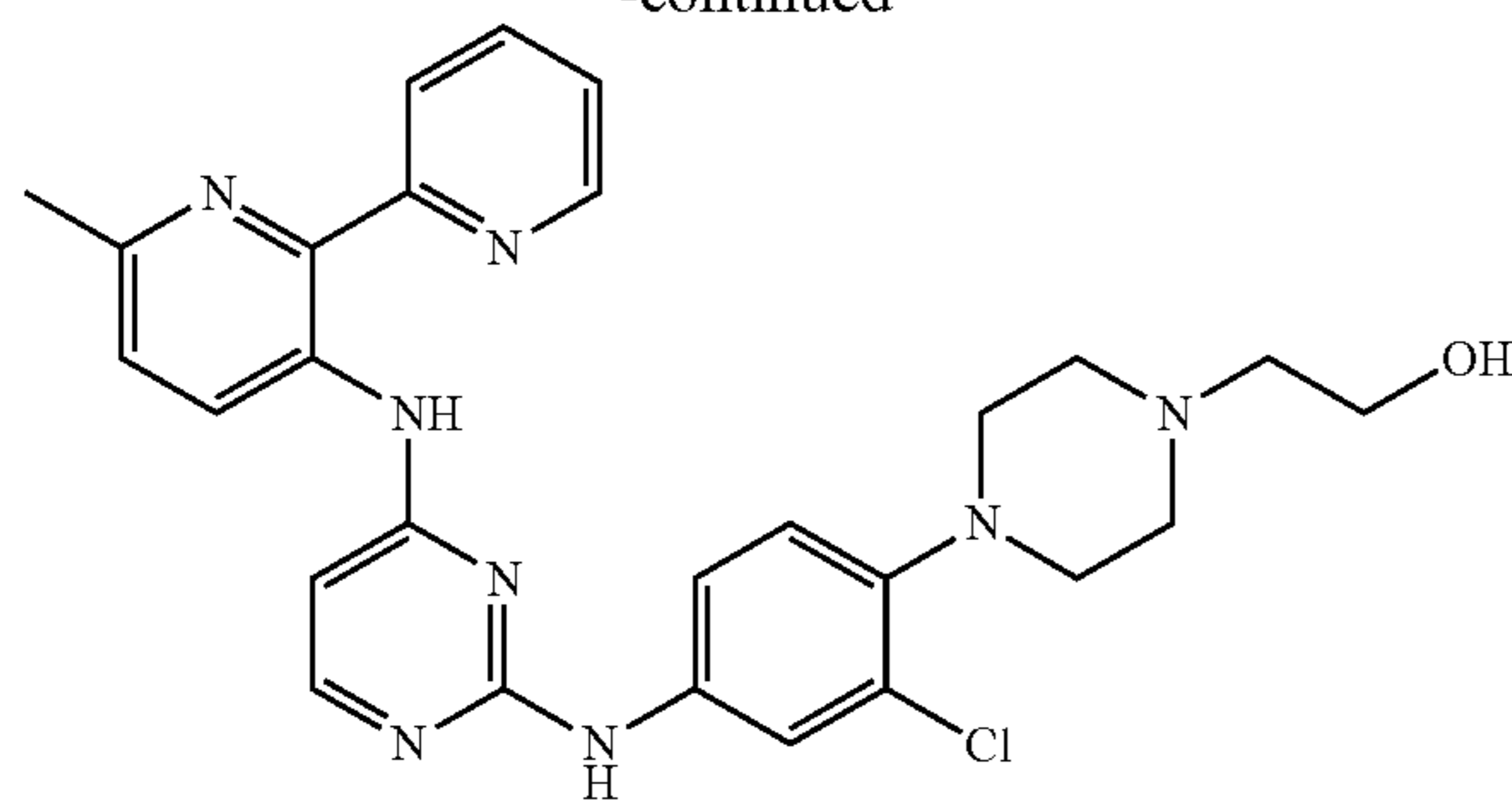
Compound 15
