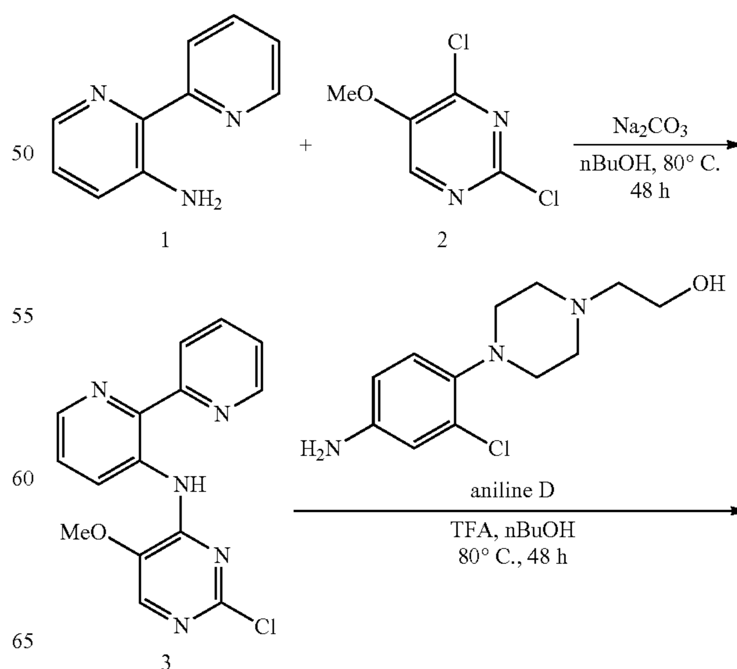
Scheme 12
