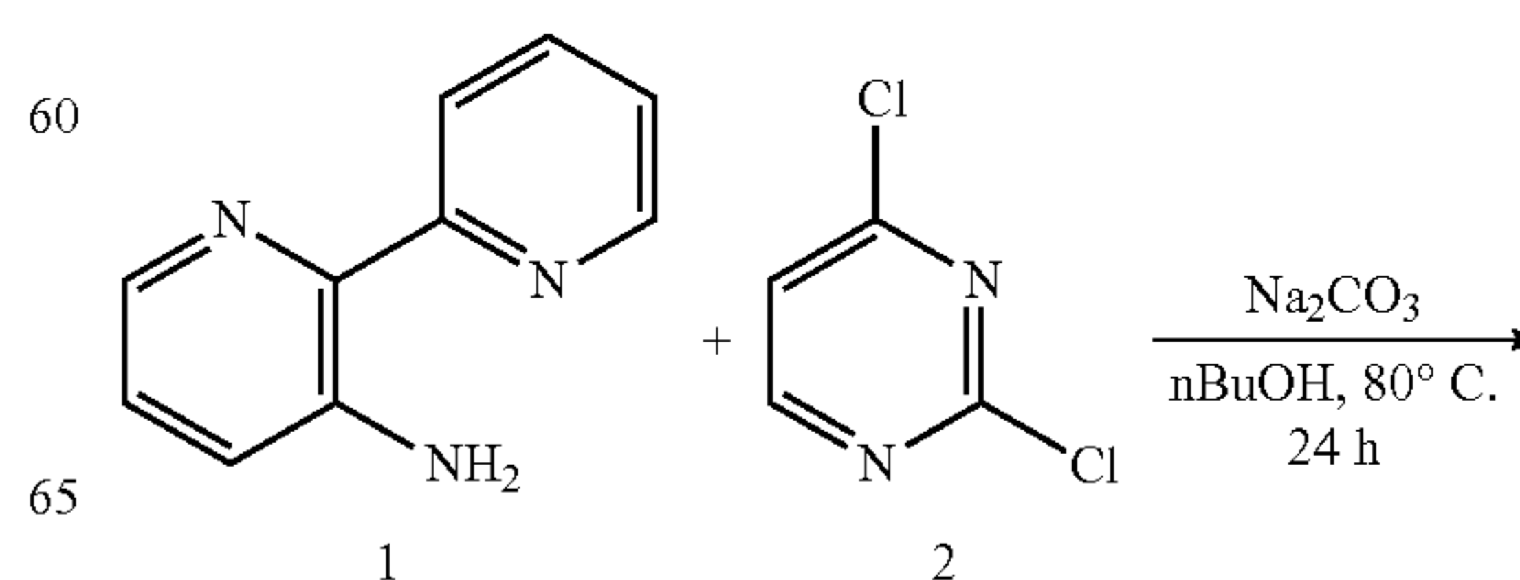
Scheme 10
