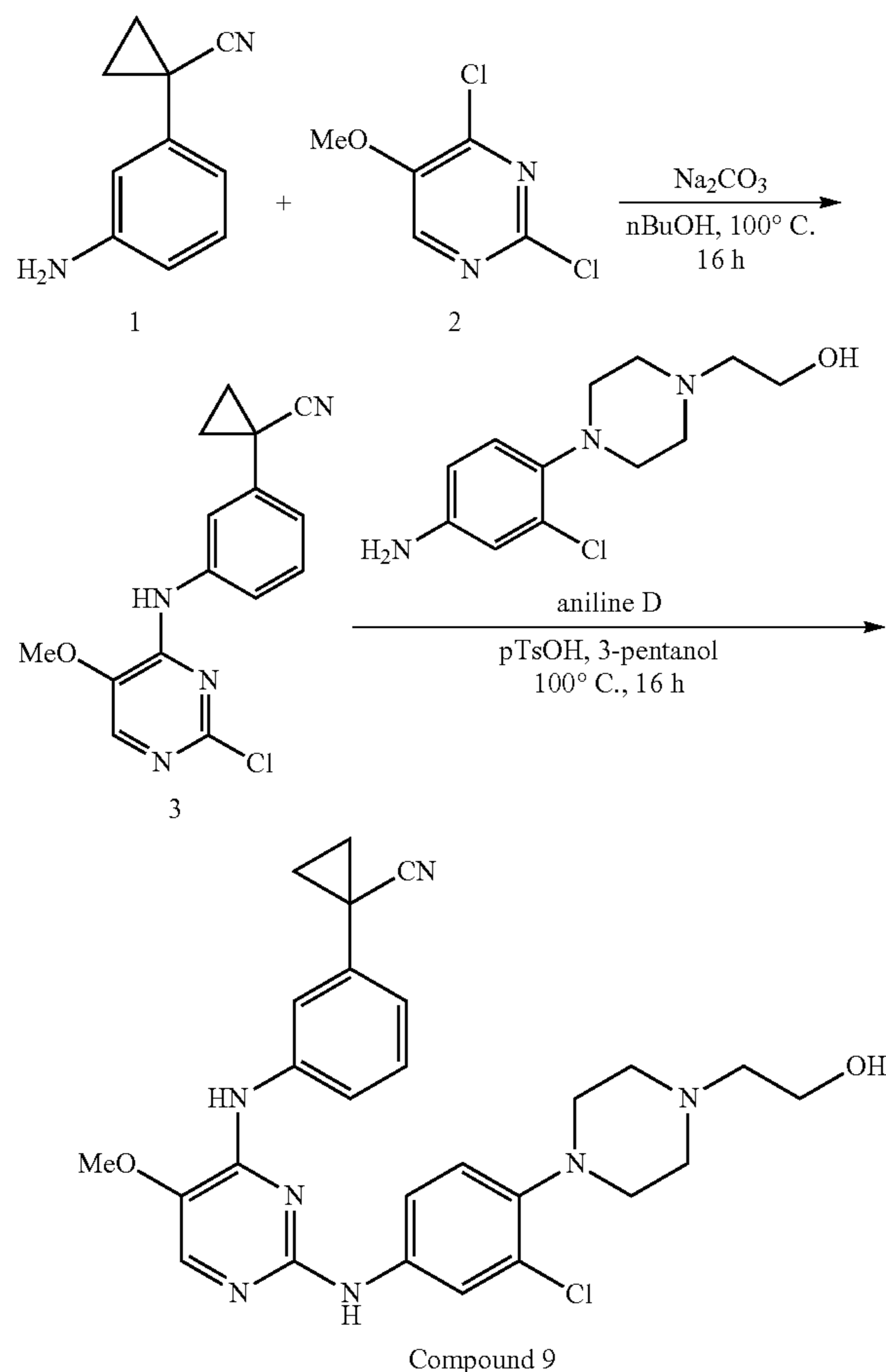
Scheme 9
