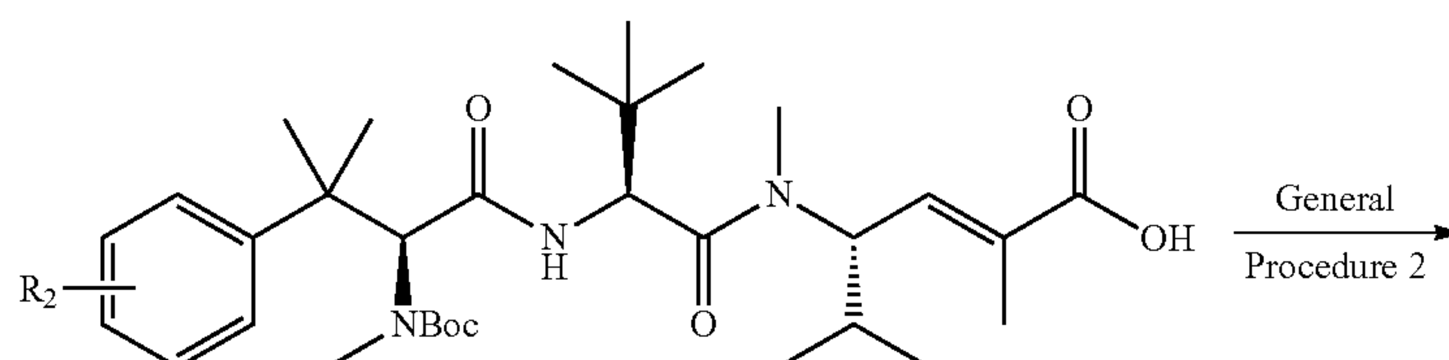
General Scheme
