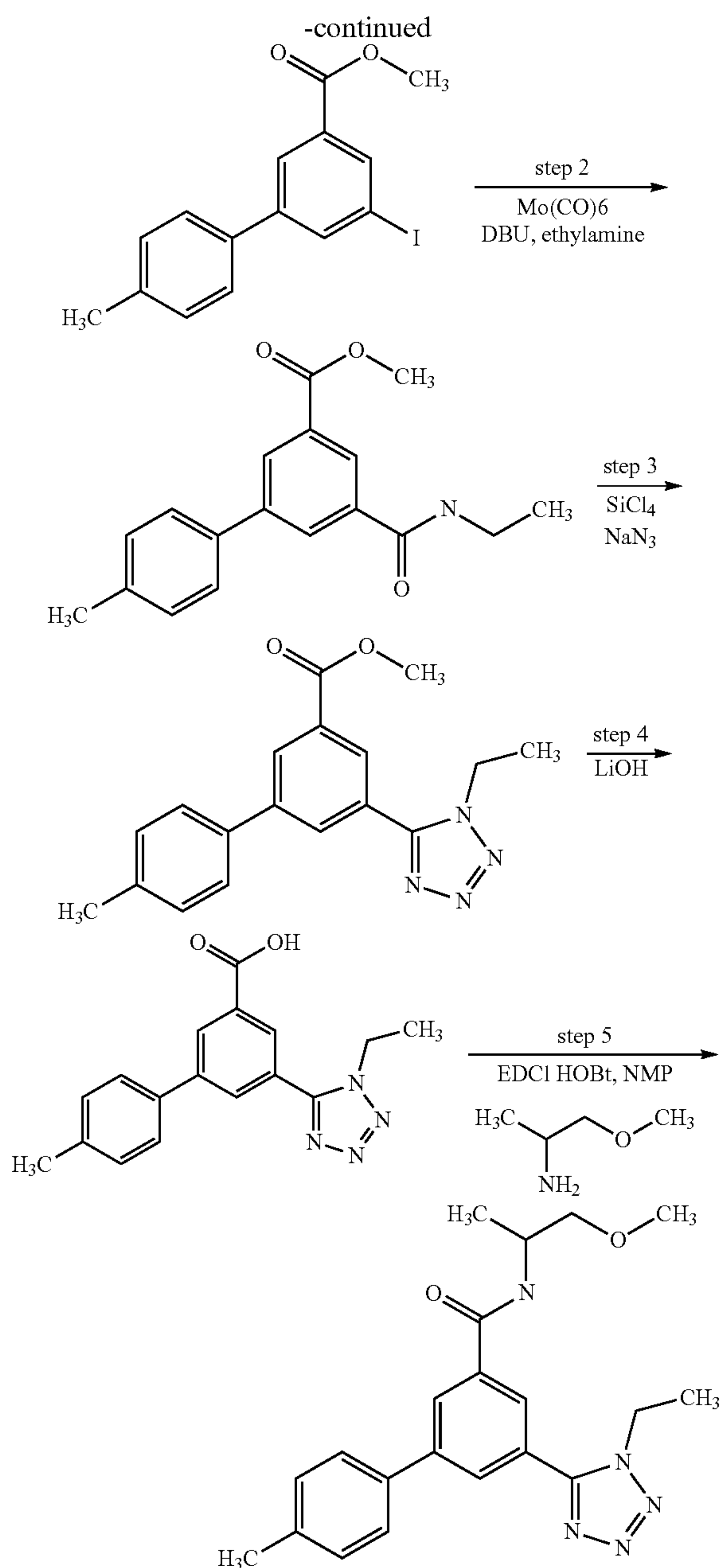
Step 1 5-Iodo-4'-methyl-biphenyl-3-carboxylic acid methyl ester
