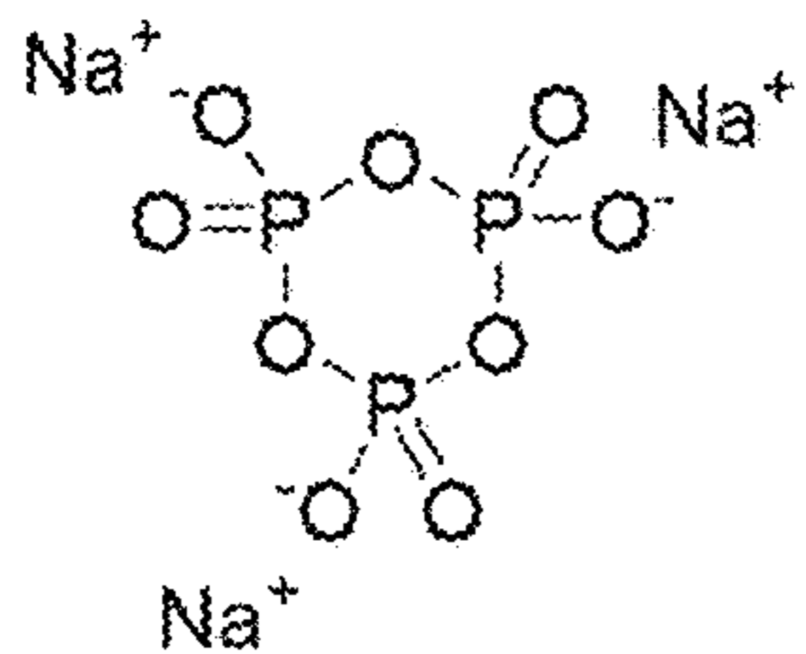
Sodium TriMetaPhosphate
