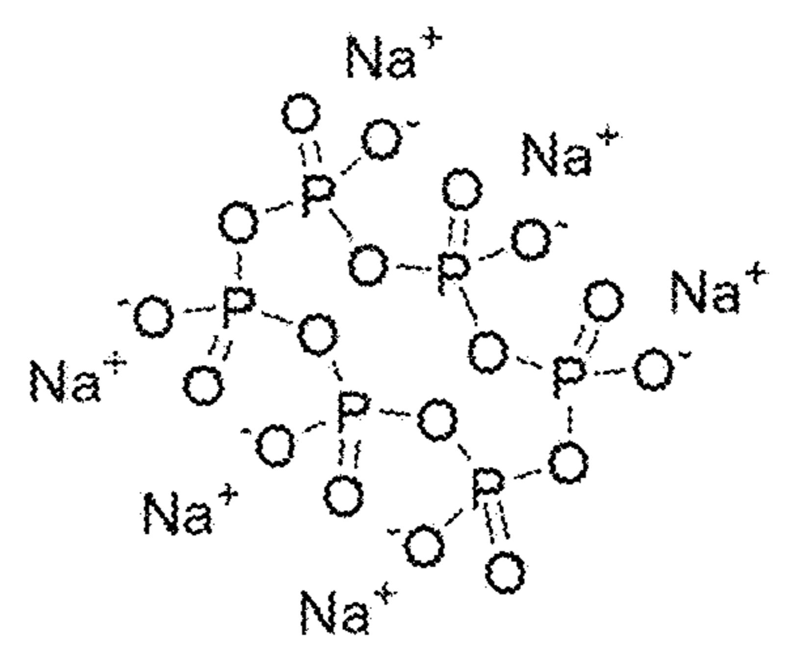
Sodium HexaMetaPhosphate
