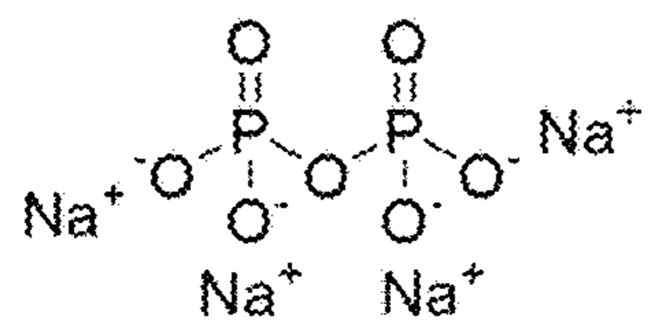
Sodium PyroPhosphate
