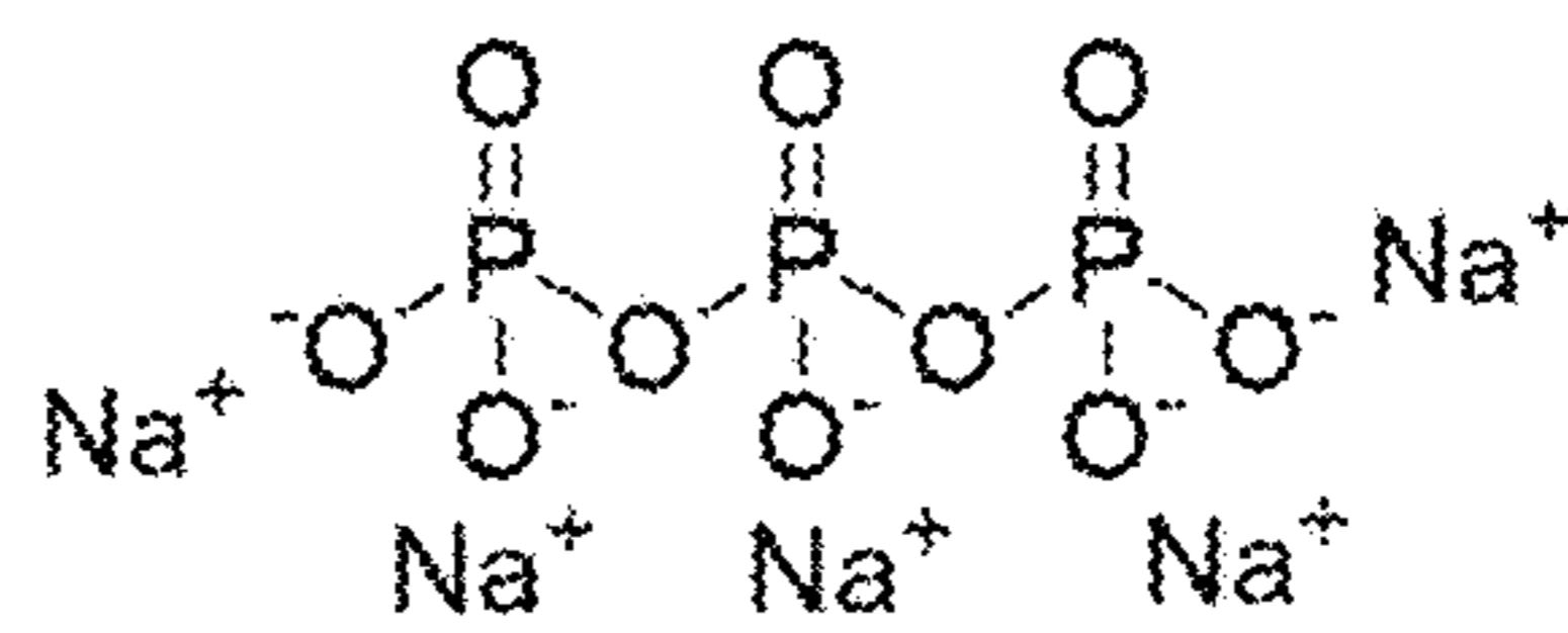
Sodium TriPolyPhosphate
