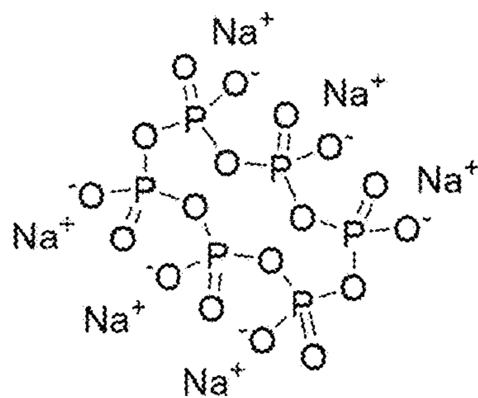
Sodium HexaMetaPhosphate
