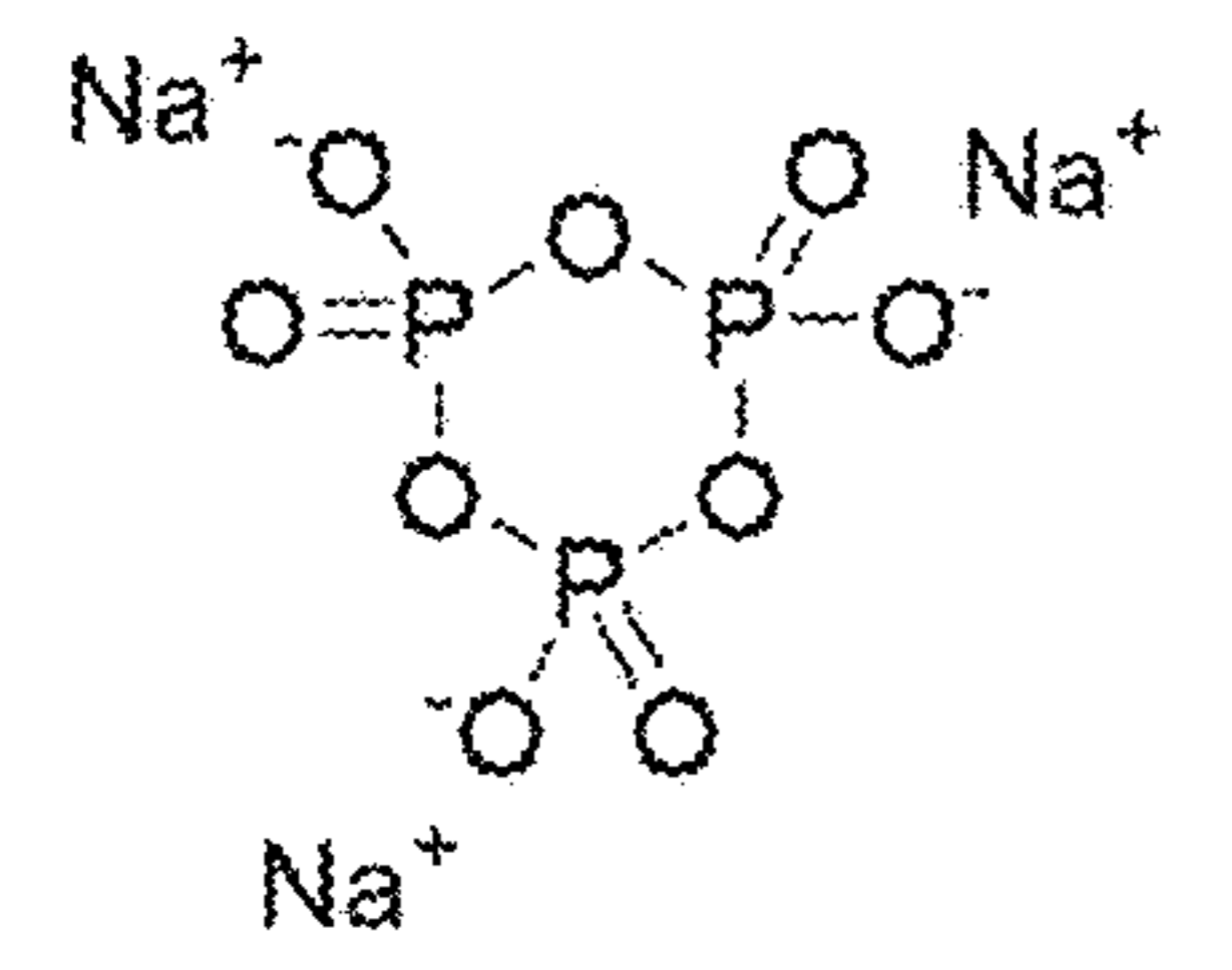
Sodium TriMetaPhosphate
