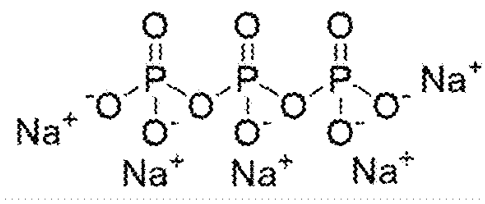
Sodium TriPolyPhosphate
