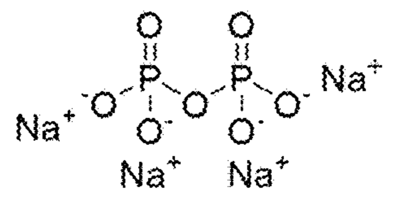
Sodium PyroPhosphate
