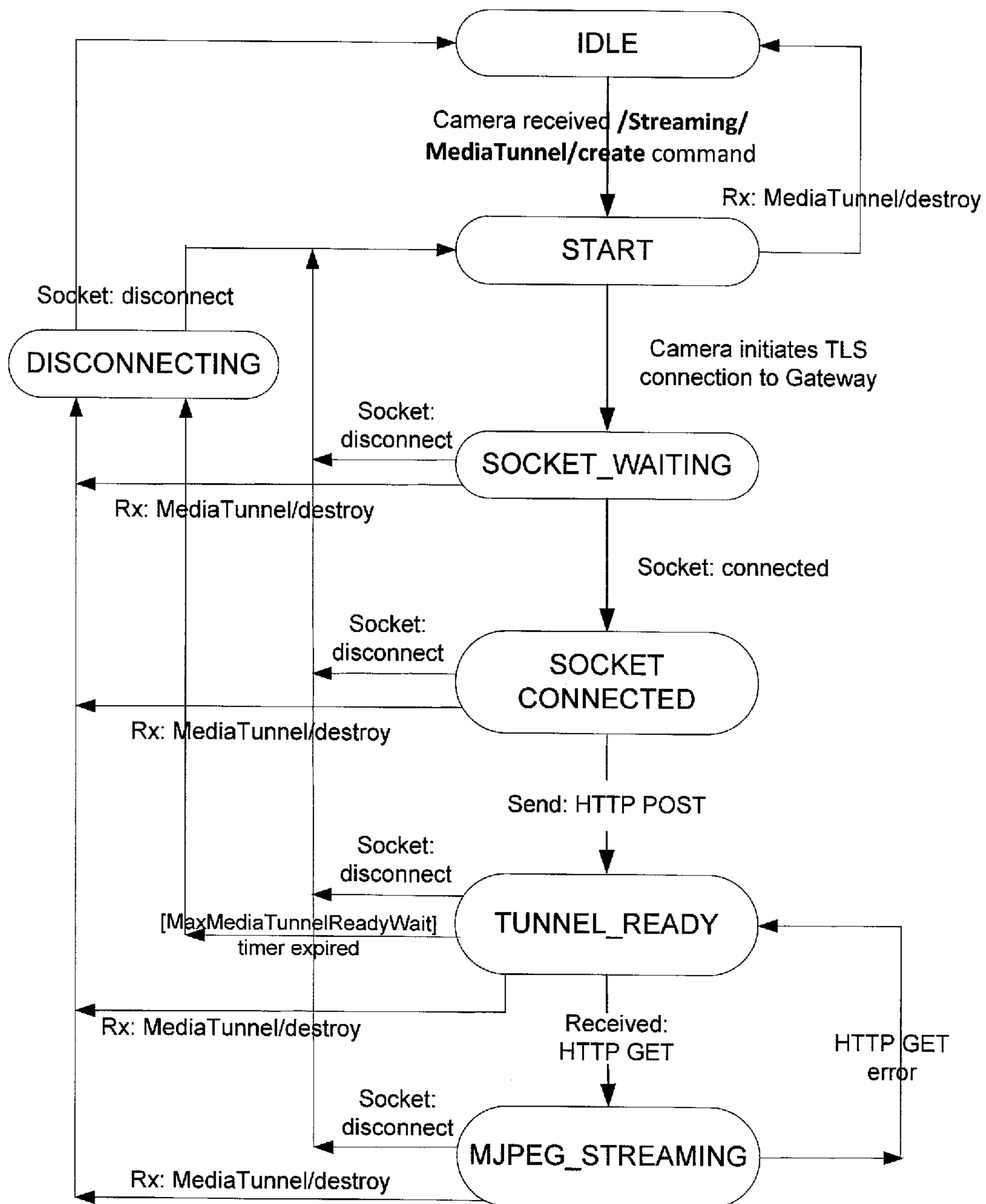
MJPEG Media Channel State Transition Diagram
