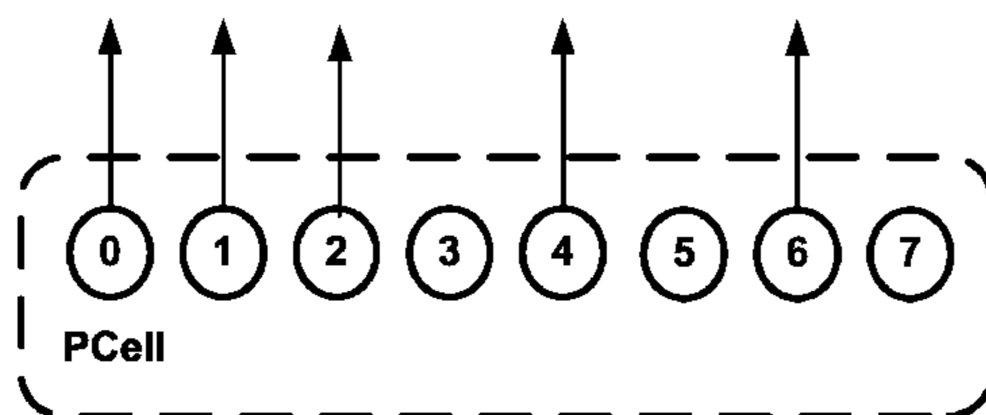
Primary PUCCH Group
