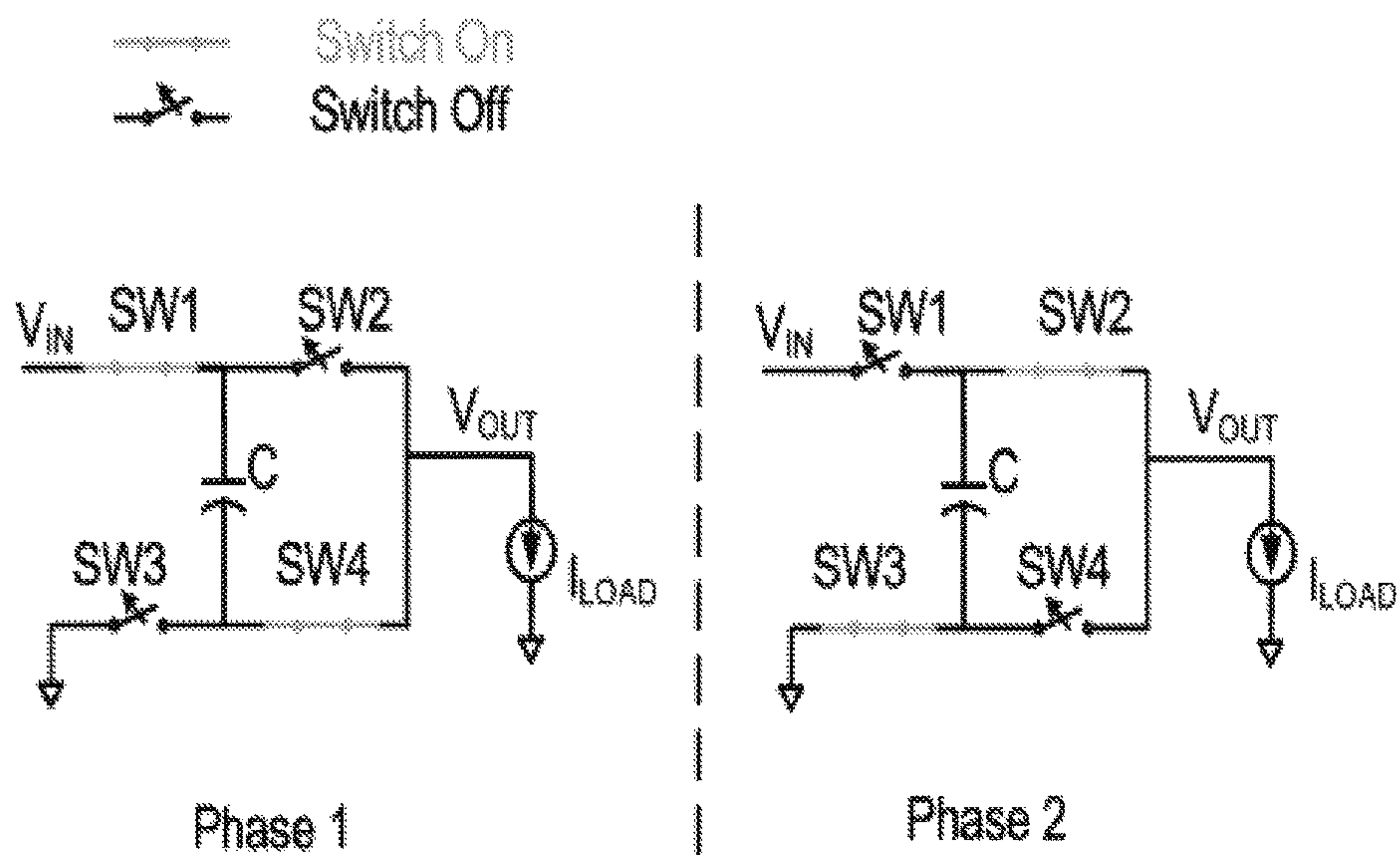
FIG. 3 (PRIOR ART)
