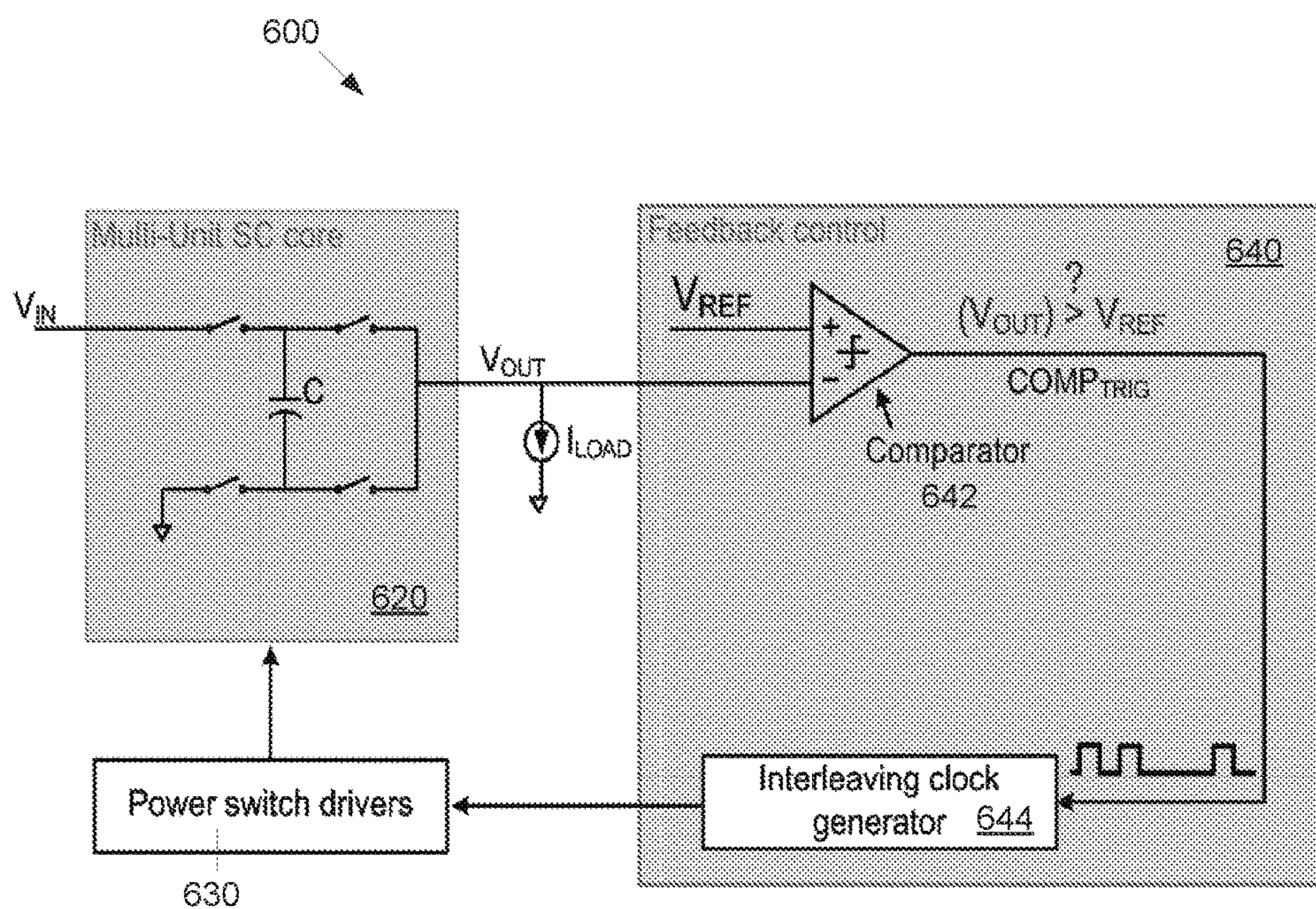
FIG. 6 (PRIOR ART)
