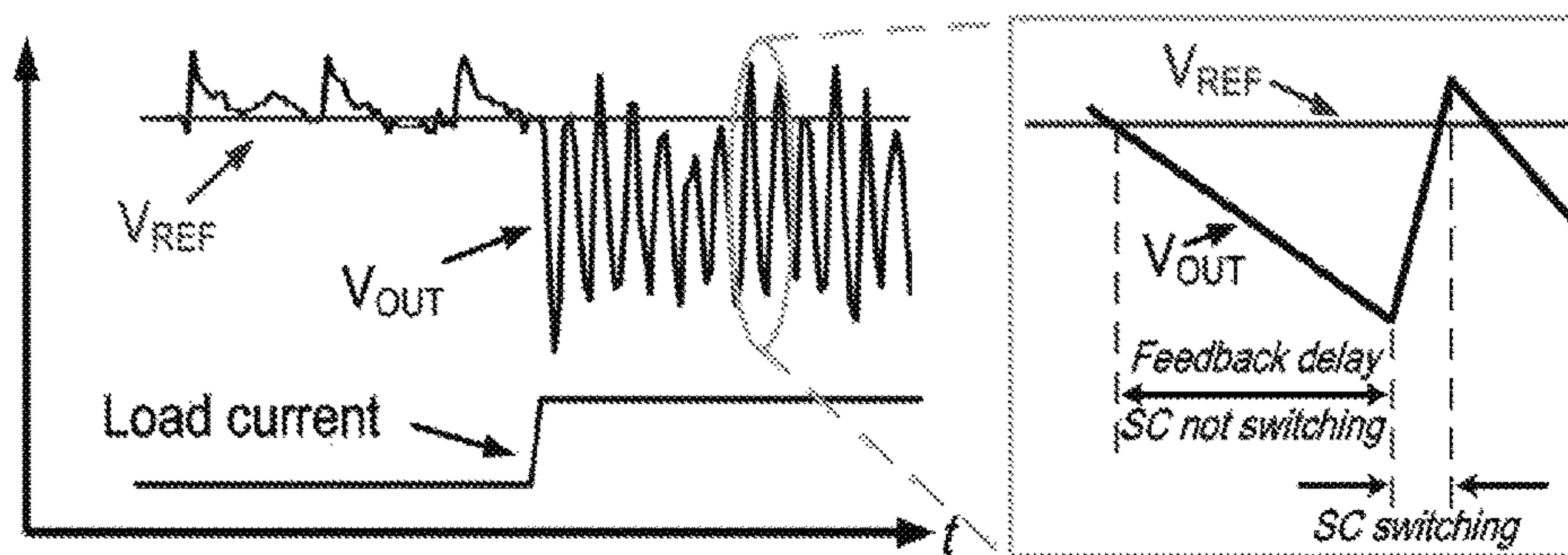
FIG. 7 (PRIOR ART)
