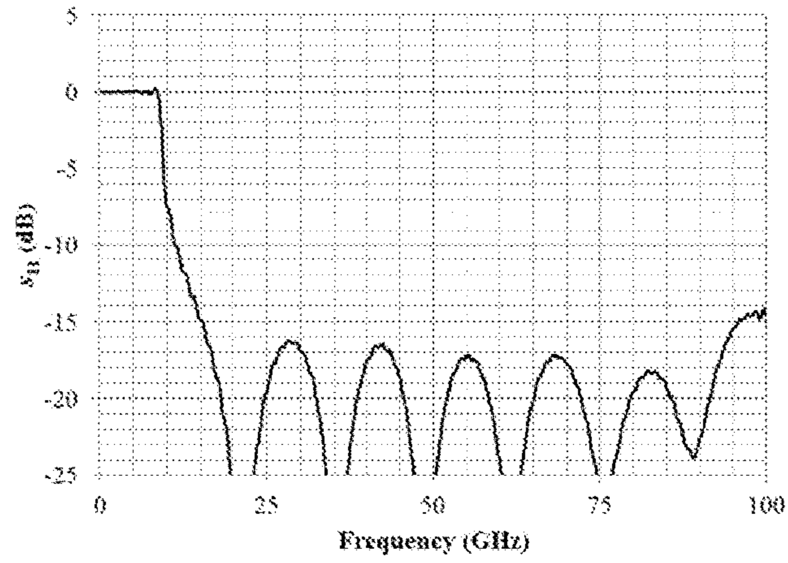
Figure 4. Simulated performance of two-probe launcher design.
