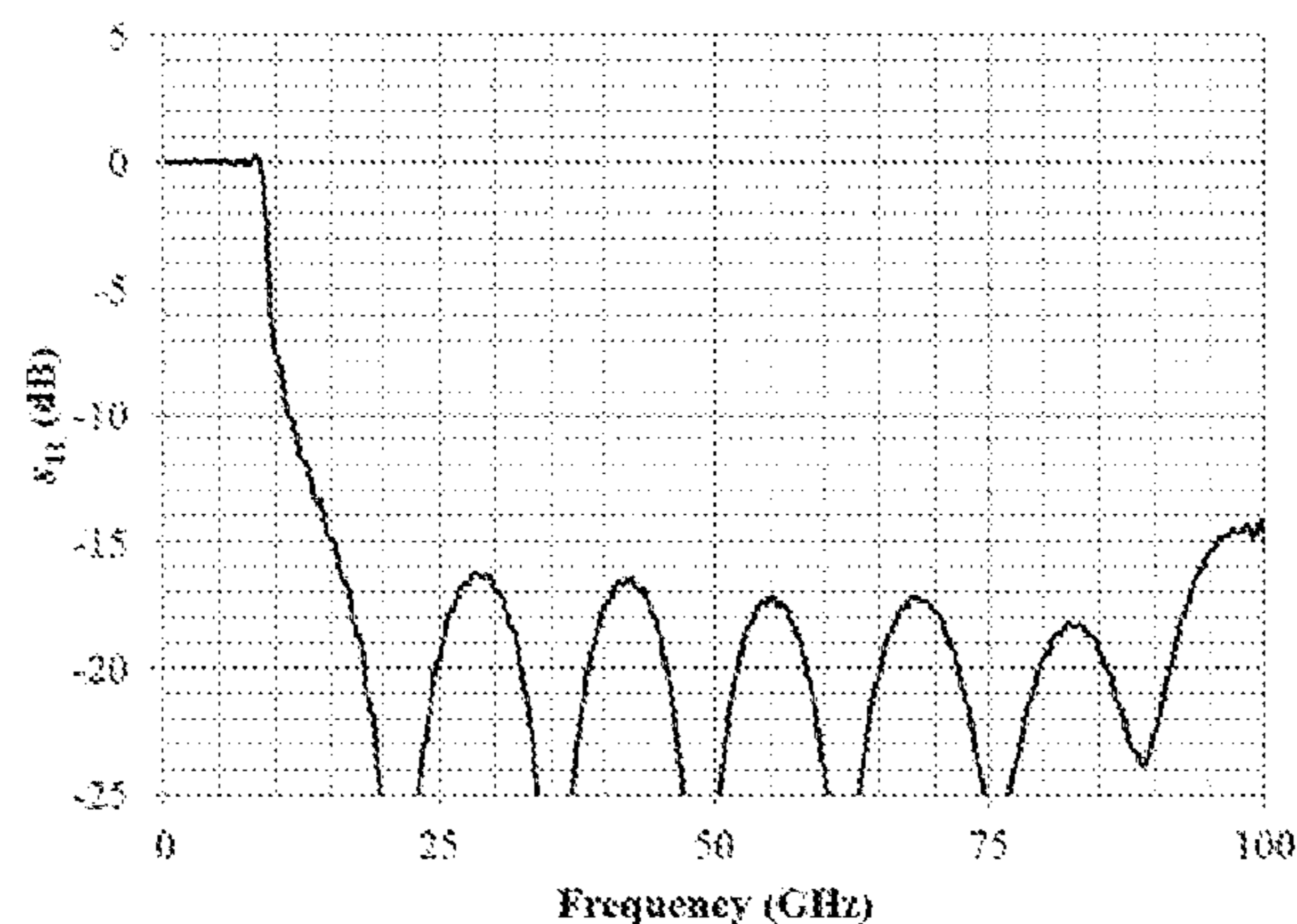
Simulated performance of two-probe launcher design.
