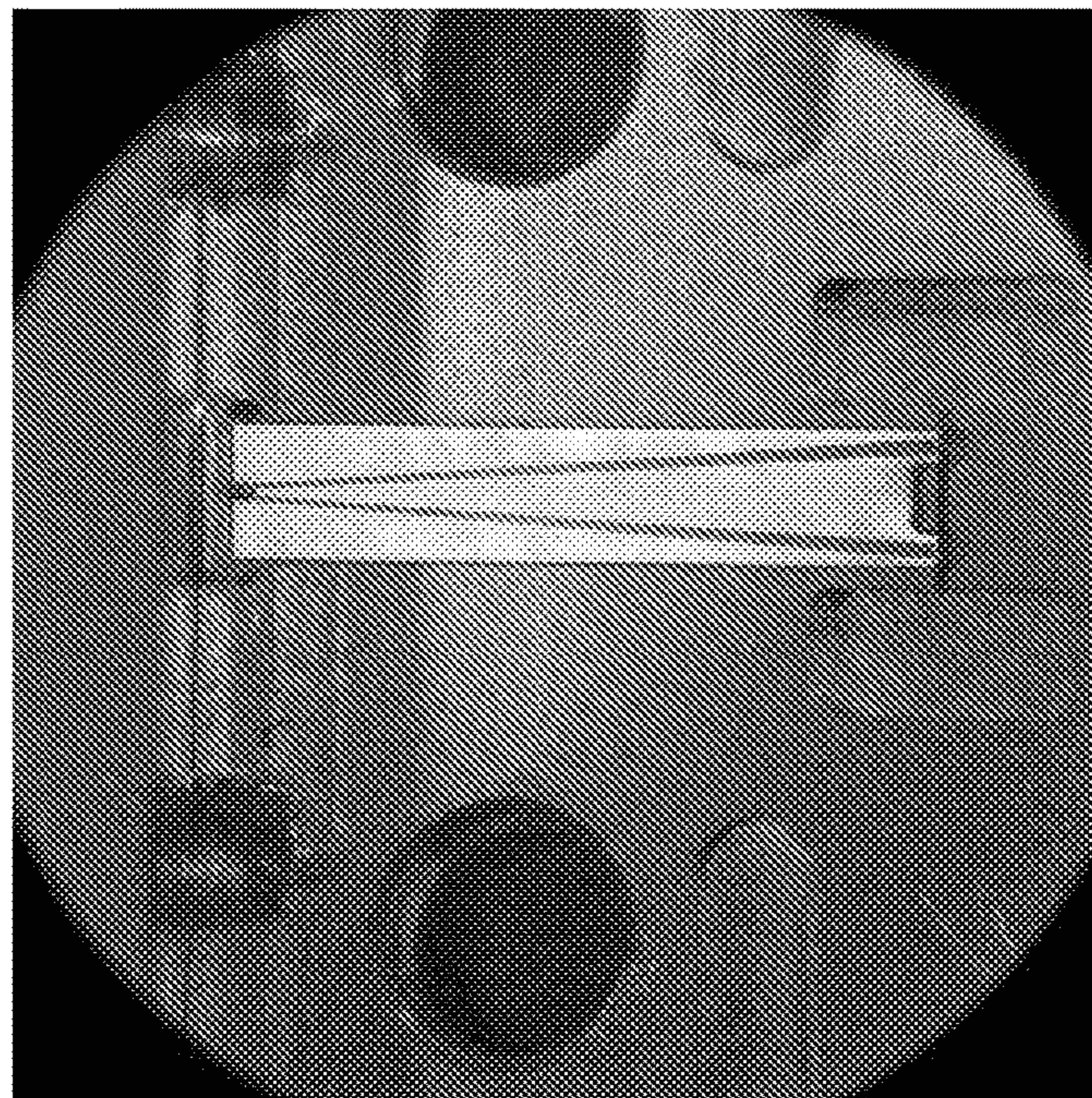
Figure 5. Photograph of launcher assembly with quartz splitter.
