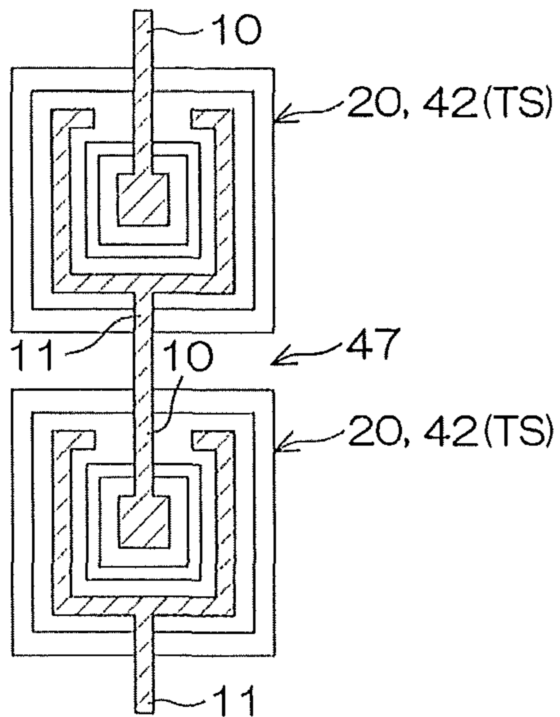
FIG. 10 (Serial connection)
