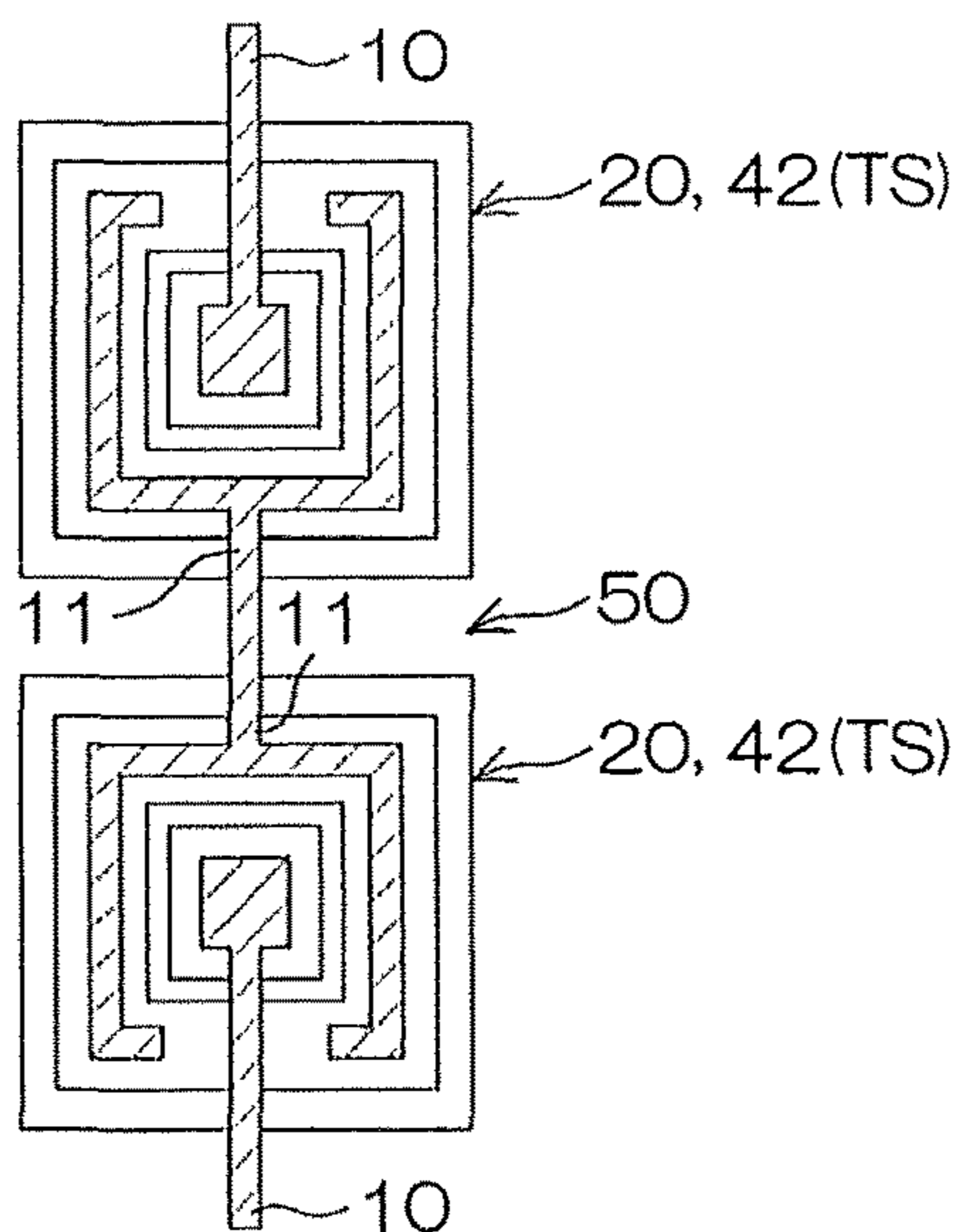
FIG. 12 (Reverse-series connection)
