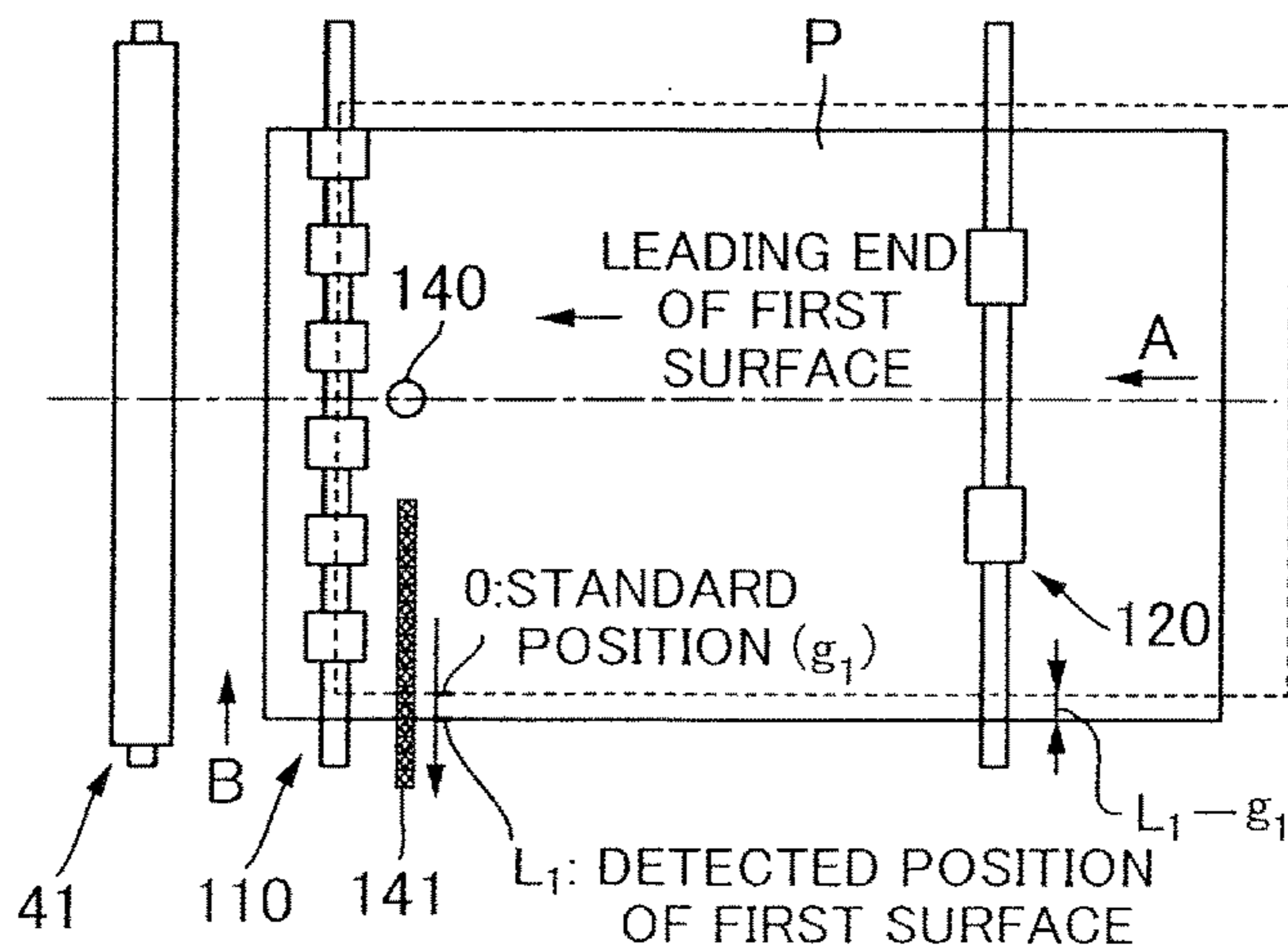
FIG.5C
