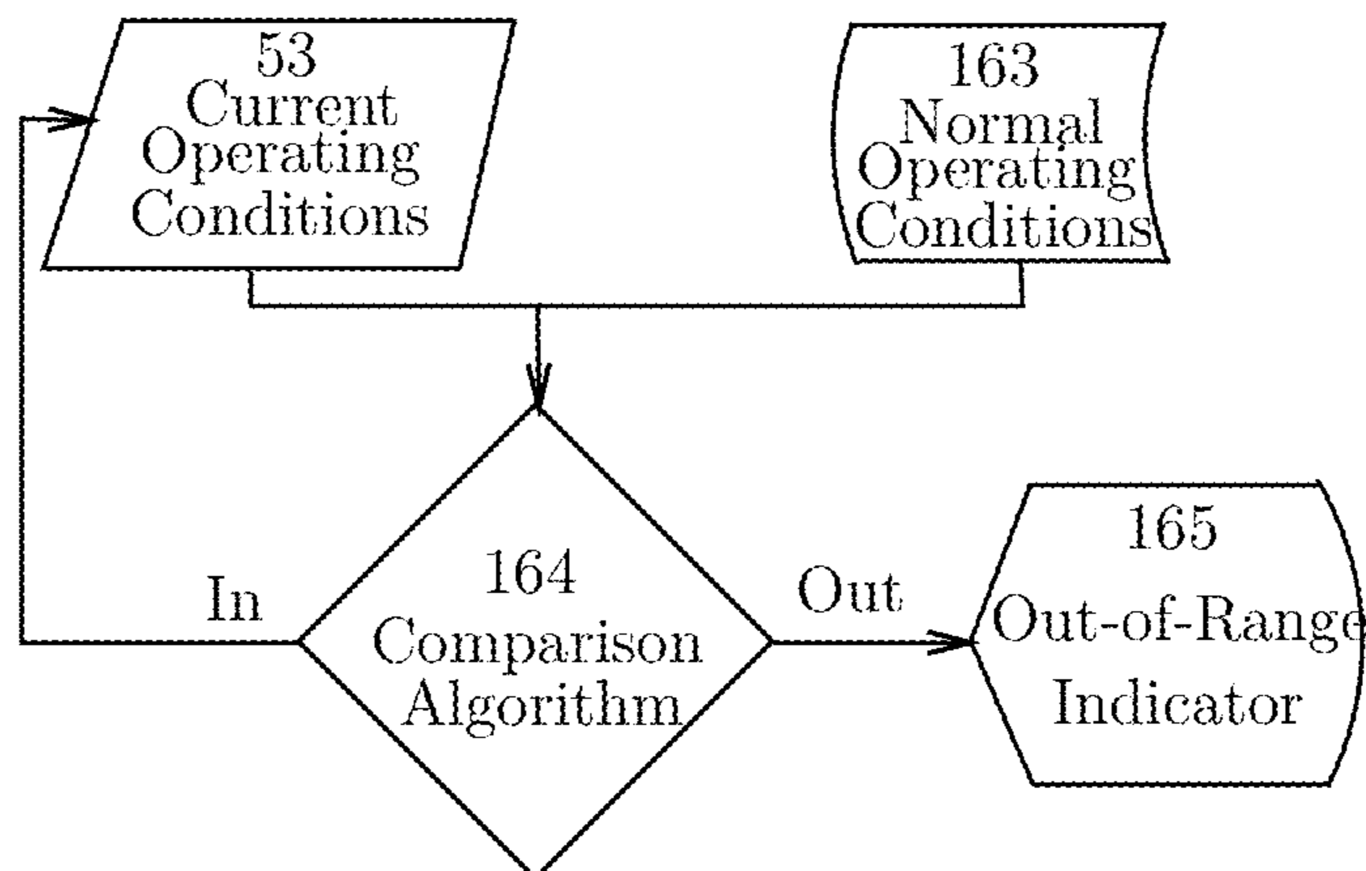
FIG. 13 Comparison Algorithm
