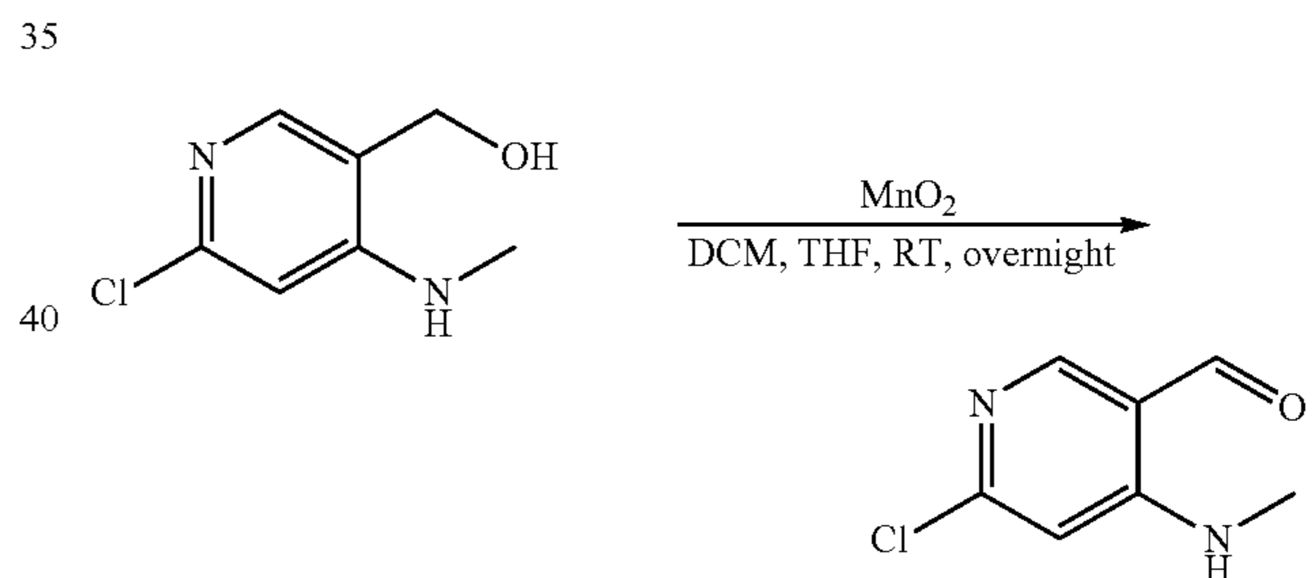
Synthesis of 6-chloro-4-(methylamino)nicotinaldehyde
