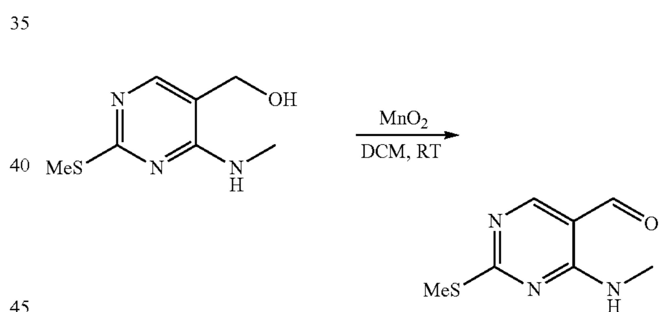
Step 3: Synthesis of 4-(methylamino)-2-(methylthio)pyrimidine-5-carbaldehyde
