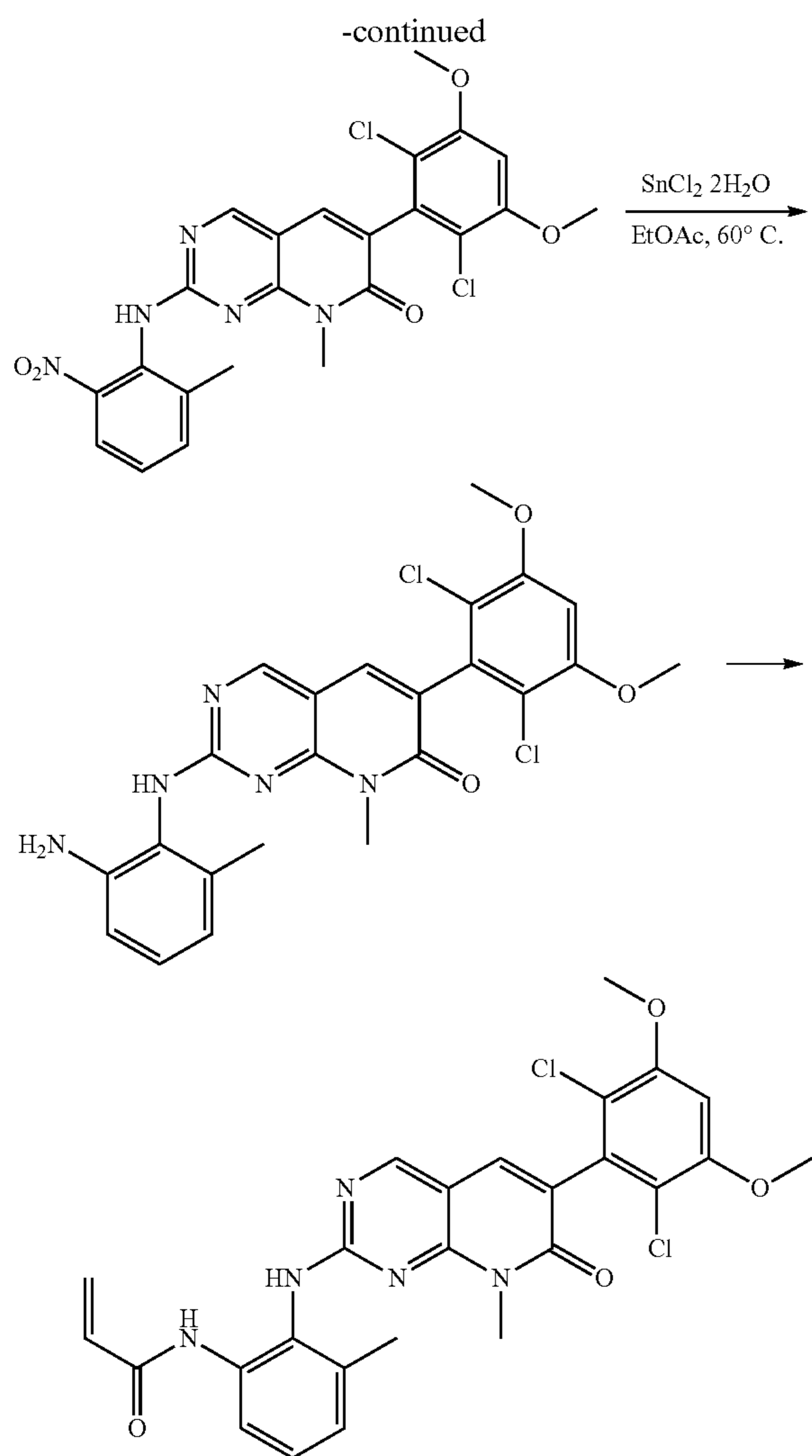
Step 1: Synthesis of ethyl 4-(methylamino)-2-(methylthio)pyrimidine-5-carboxylate
