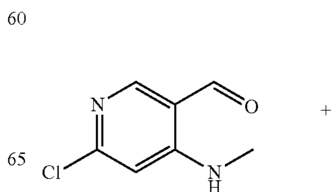
Synthesis of 7-chloro-3-(3,5-dimethoxyphenyl)-1-methyl-1,6-naphthyridin-2(1H)-one
