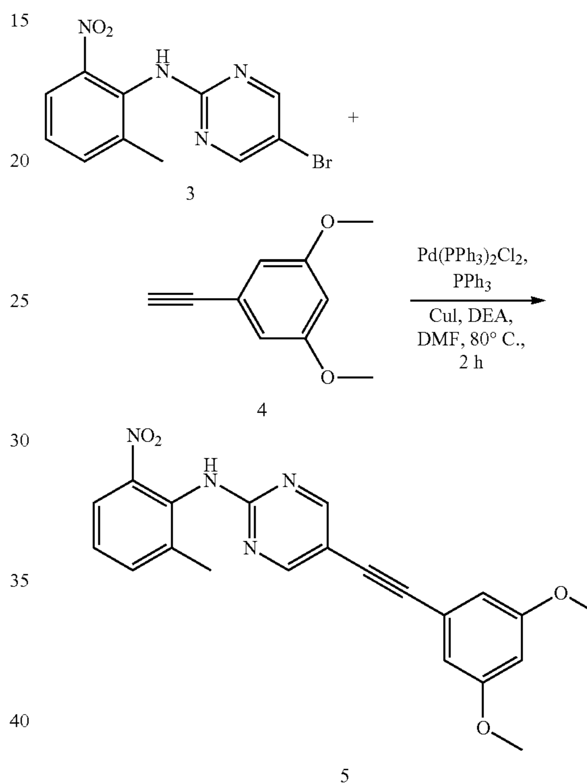
Synthesis of 5-bromo-N-(2-methyl-6-nitrophenyl)pyrimidin-2-amine
