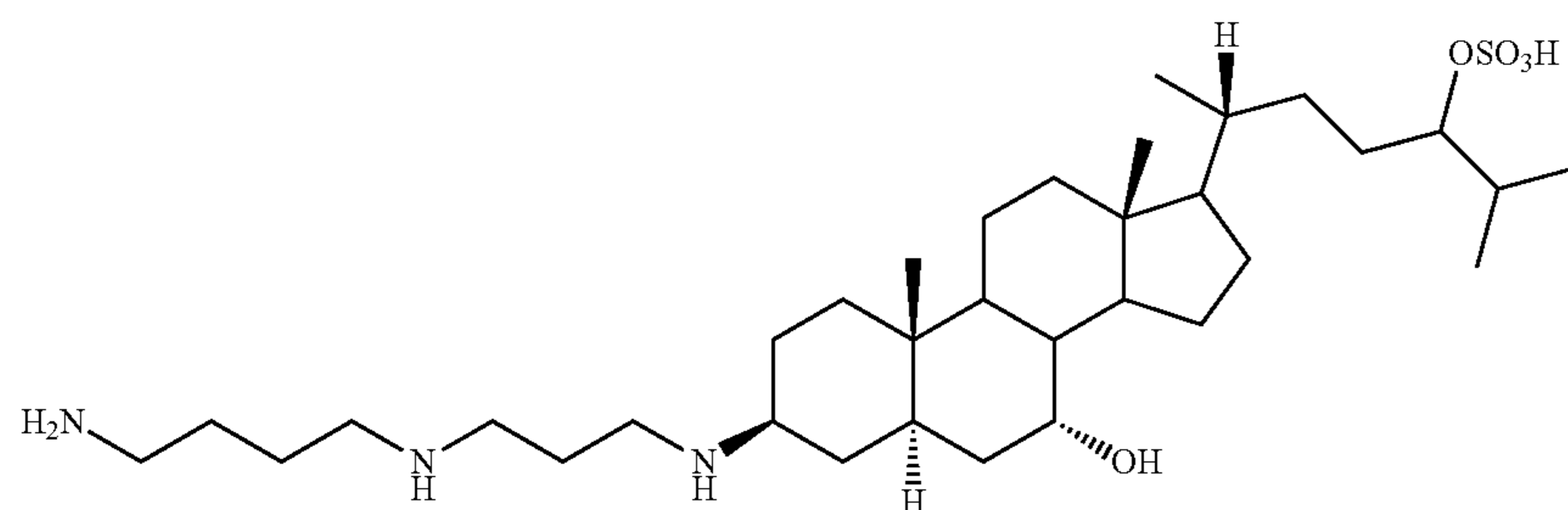
(Squalamine)
