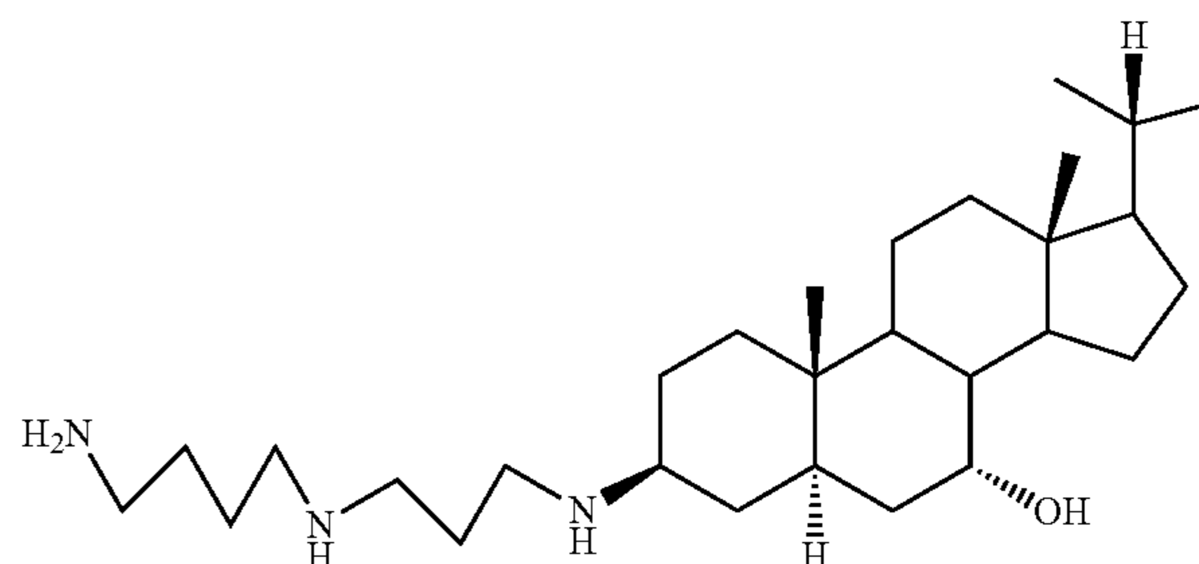
Compound 1
