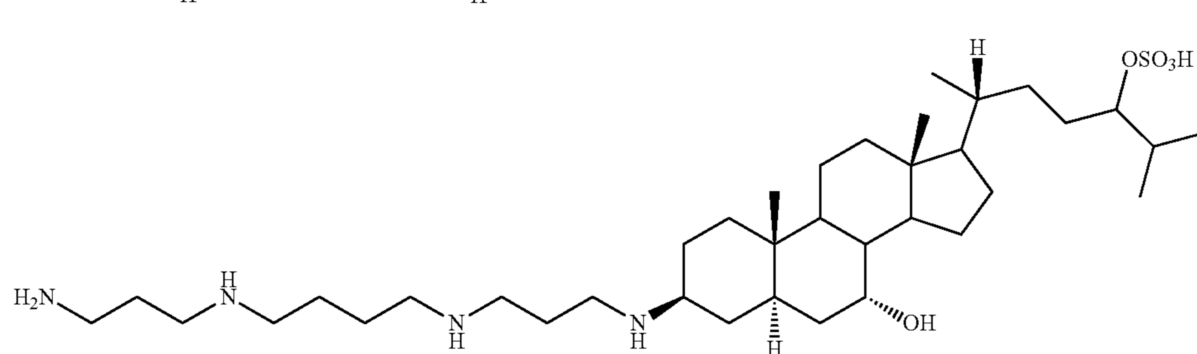
Compound 7
