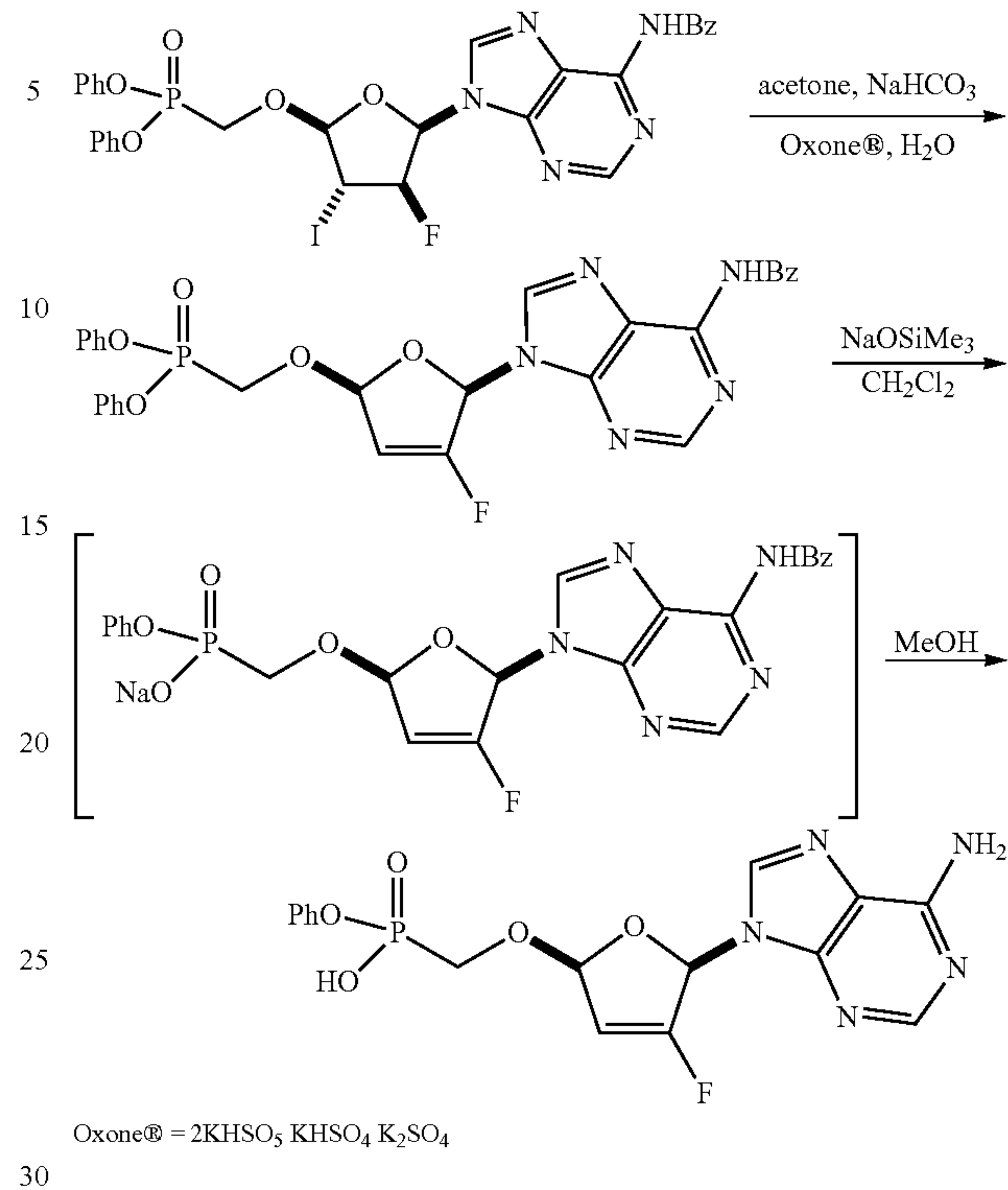
Scheme 13
