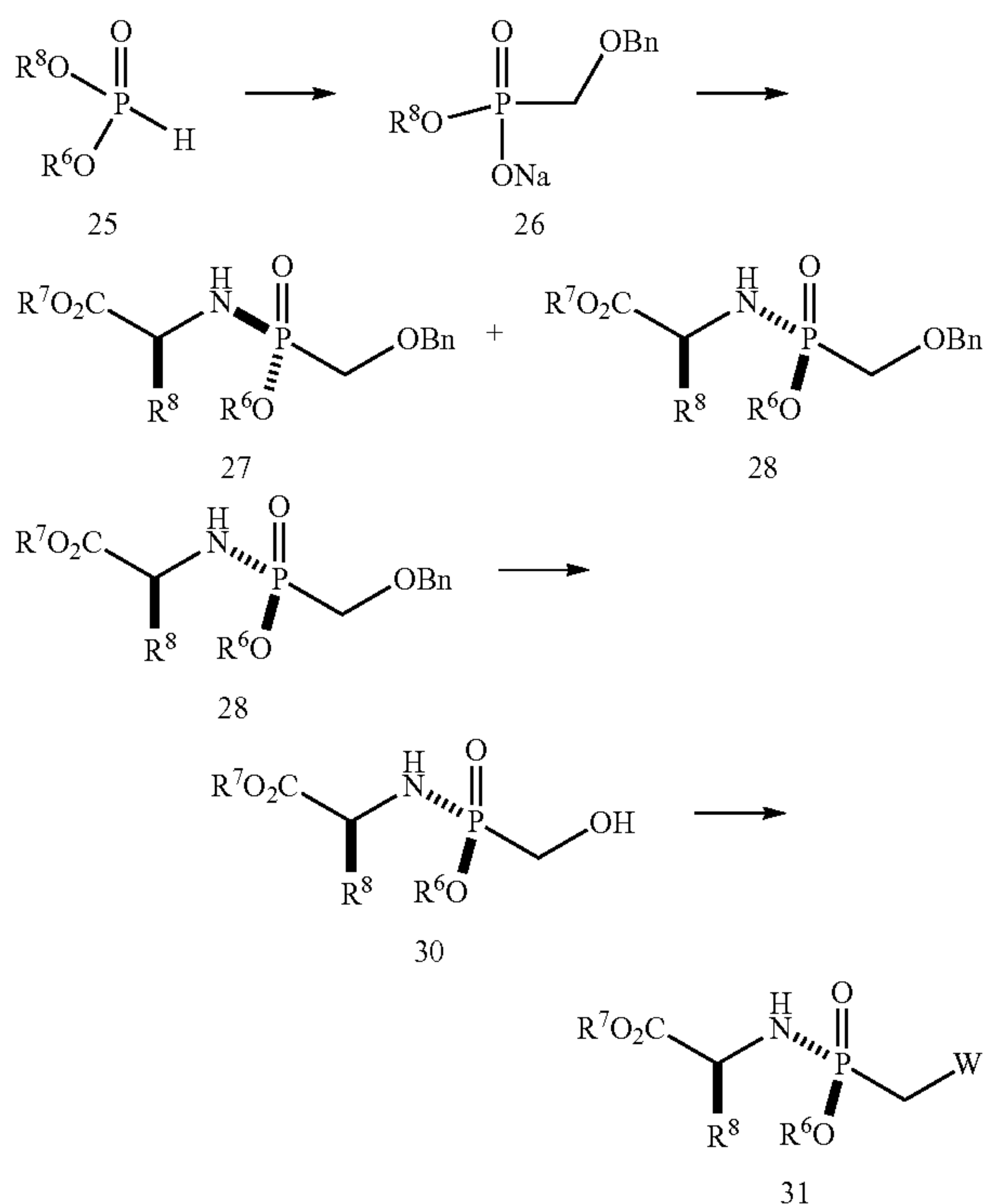
Scheme 9
