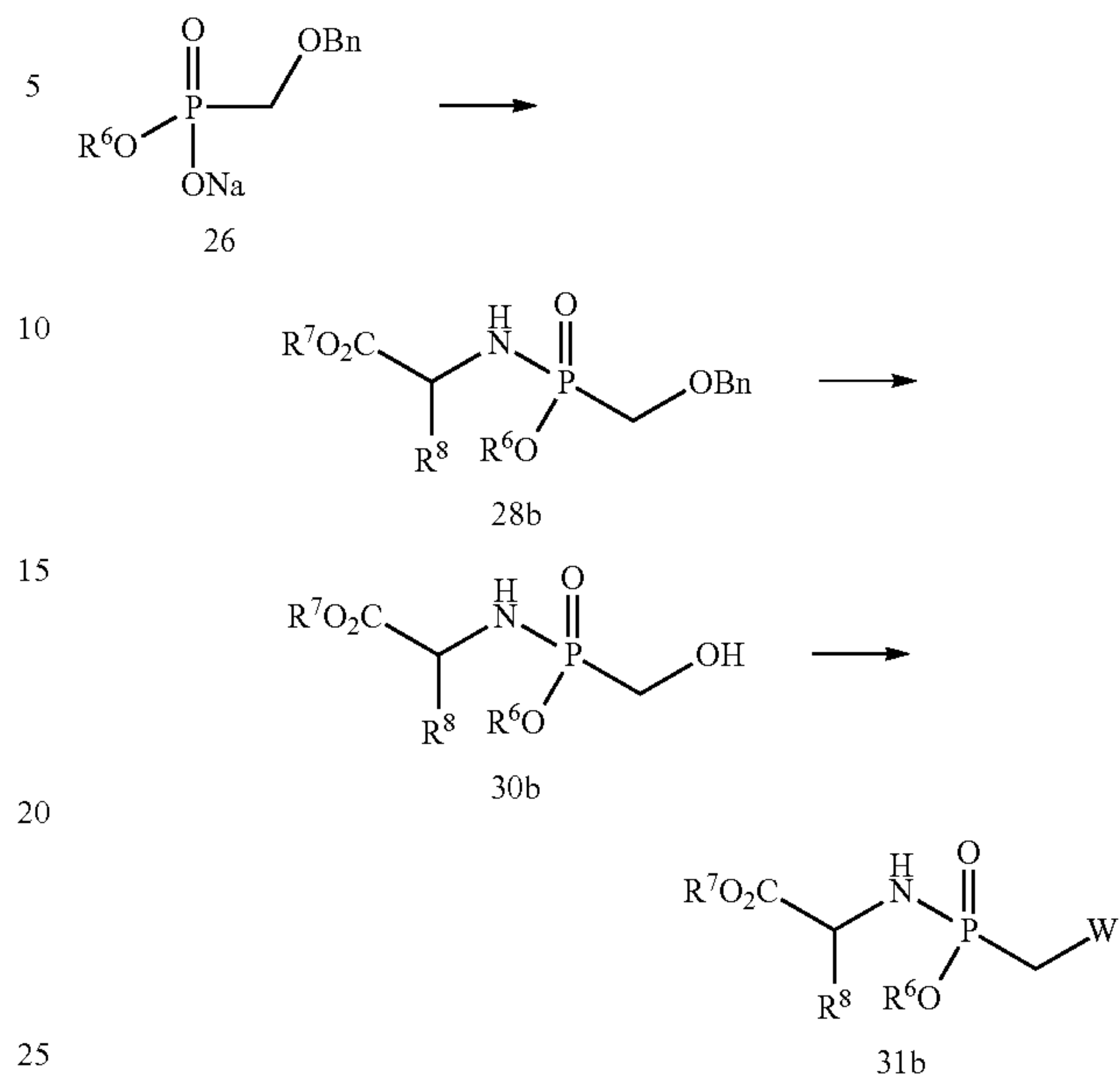
Scheme 10
