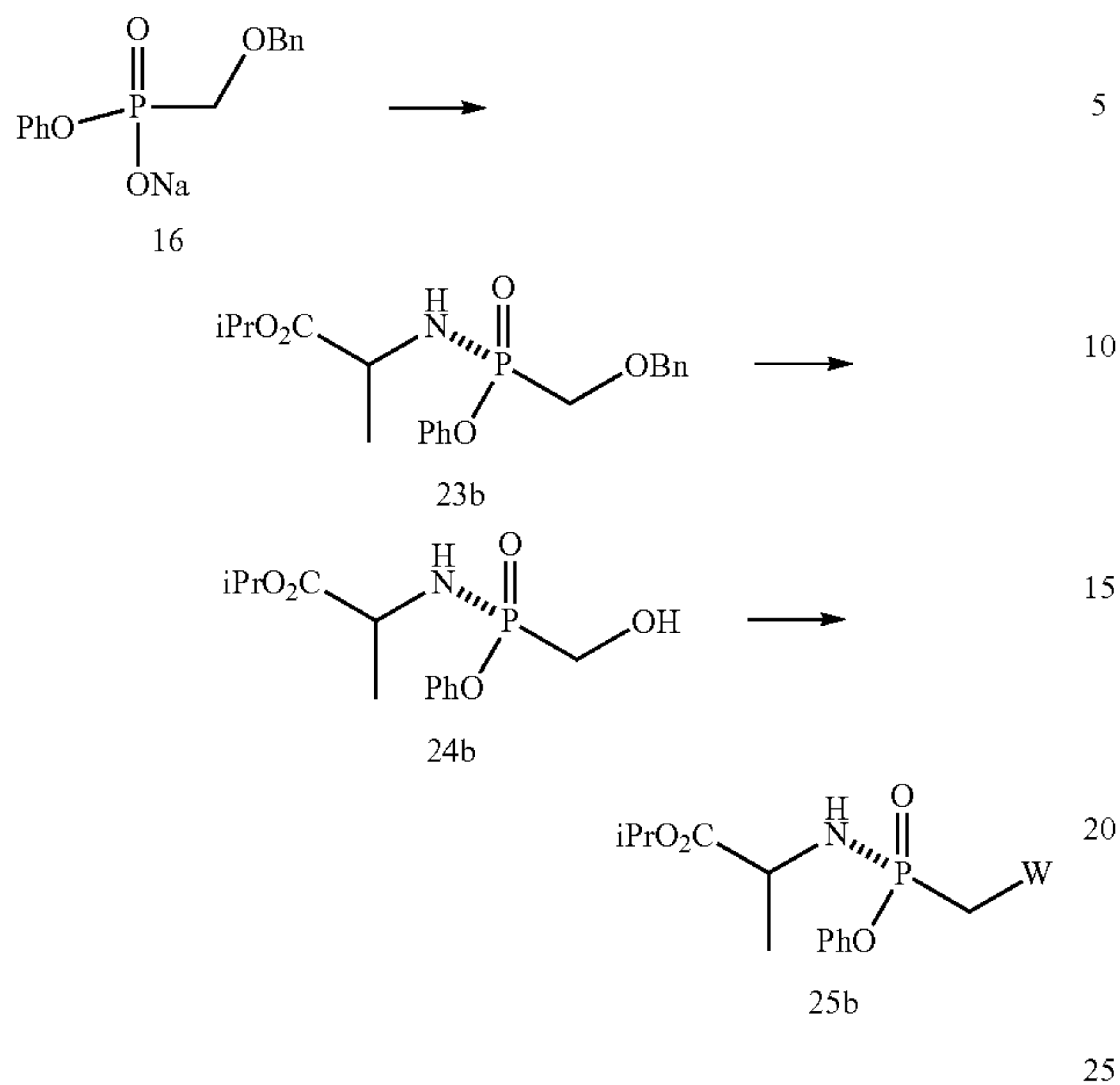
Scheme 8
