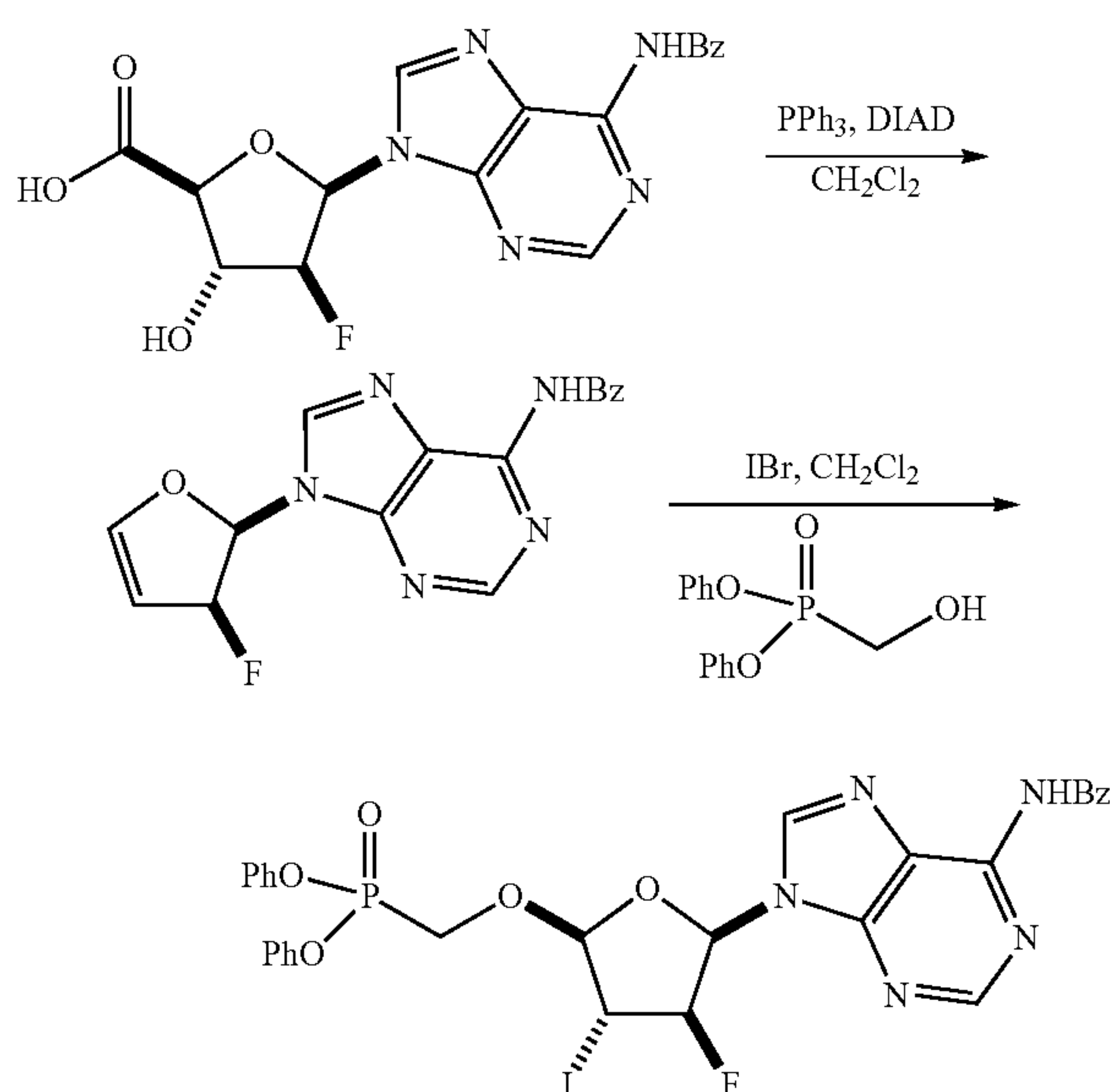
Scheme 12
