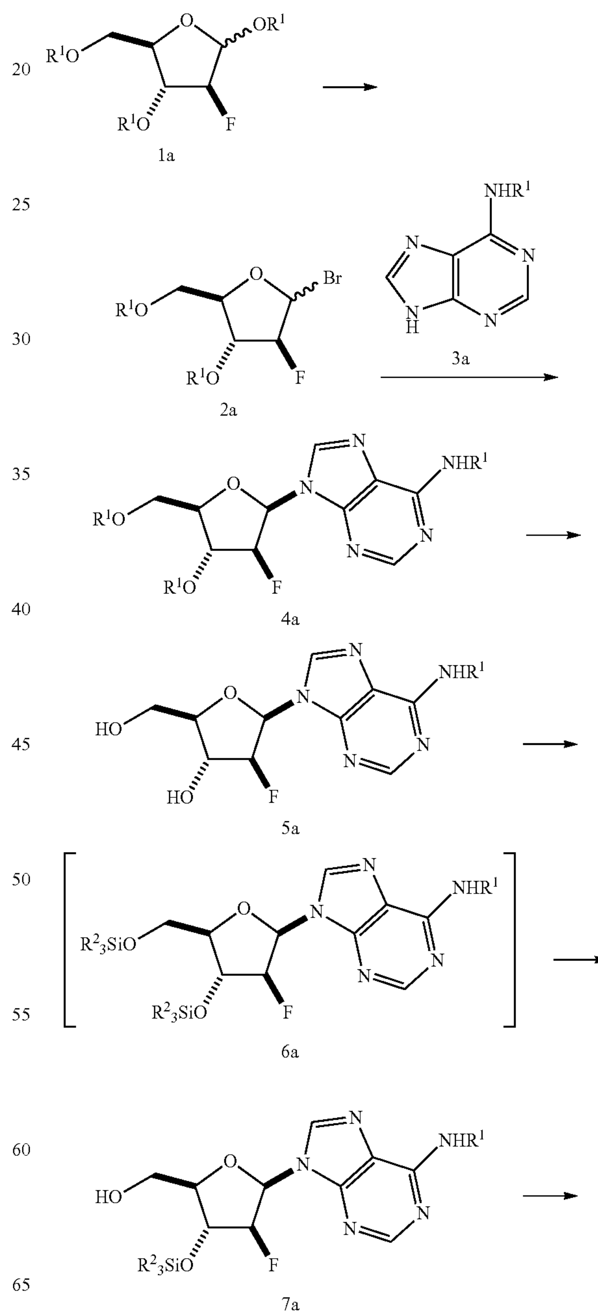
Scheme 1
