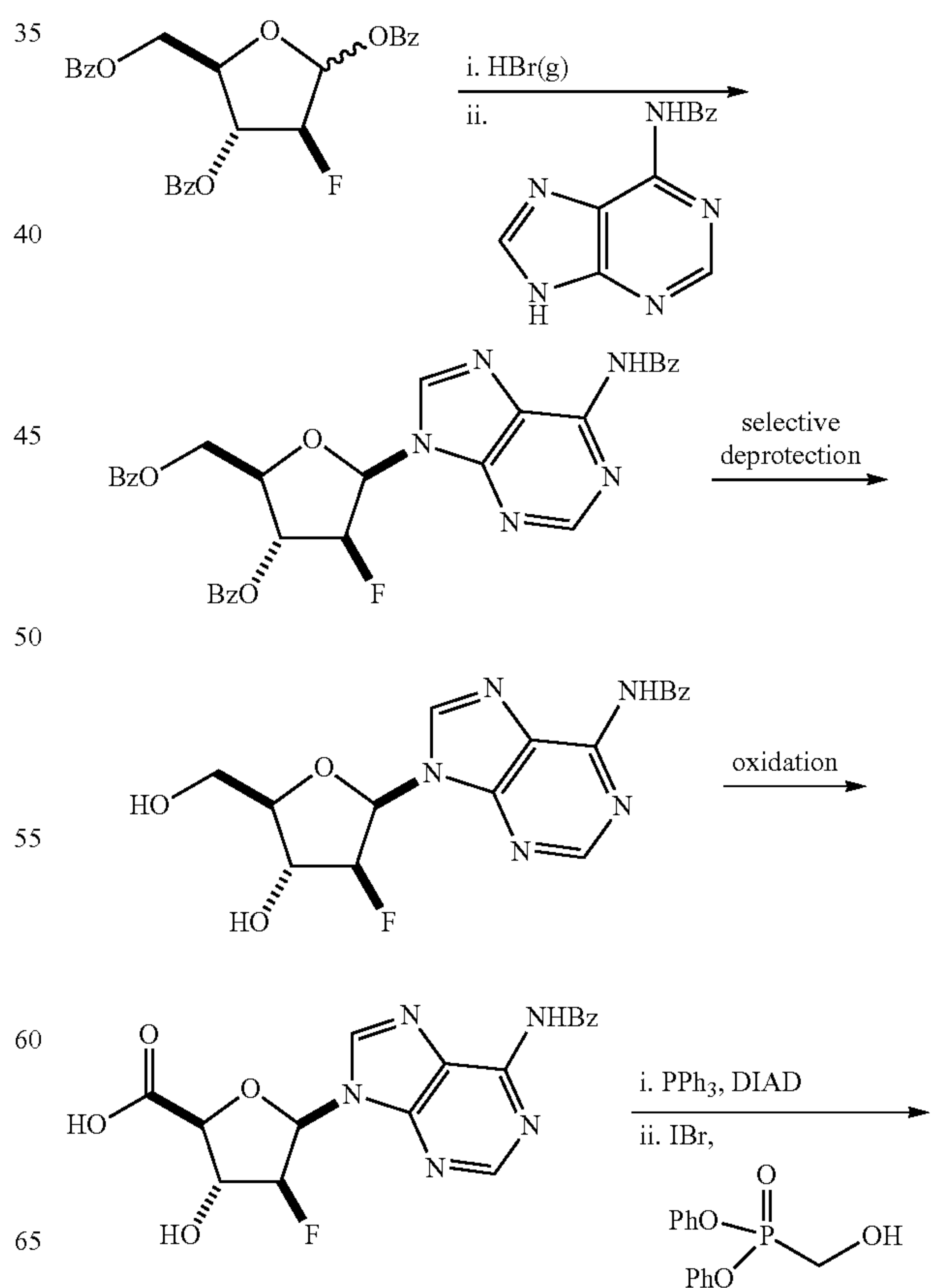
Scheme 11
