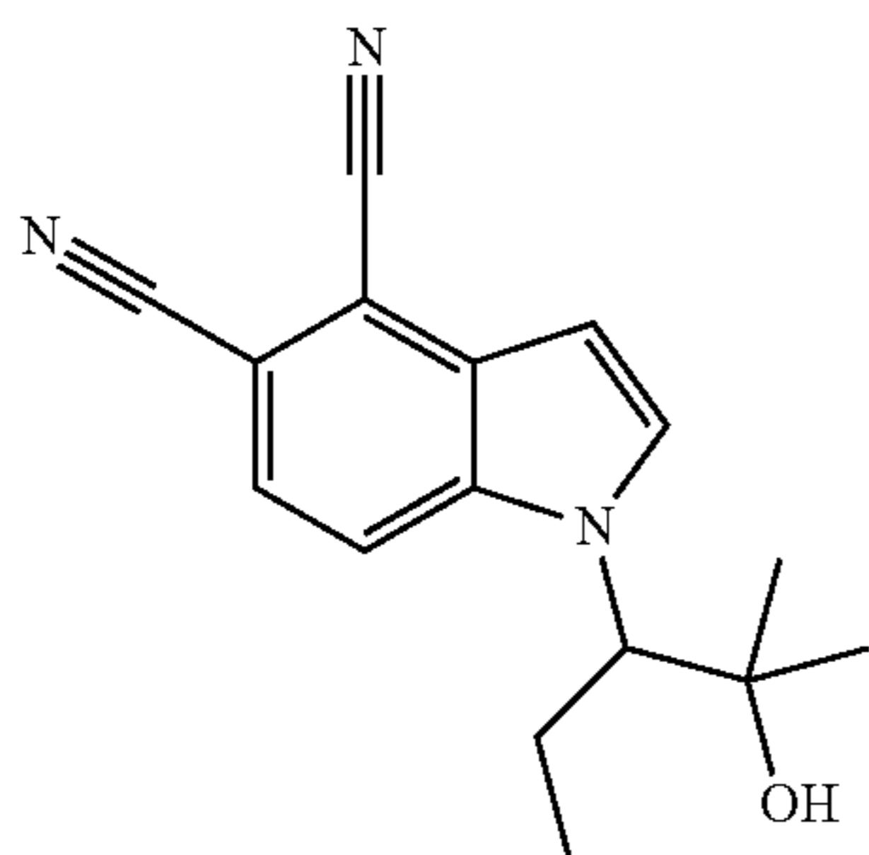
1-(2-Hydroxy-2-methylpentan-3-yl)-1H-indole-4,5-dicarbonitrile
