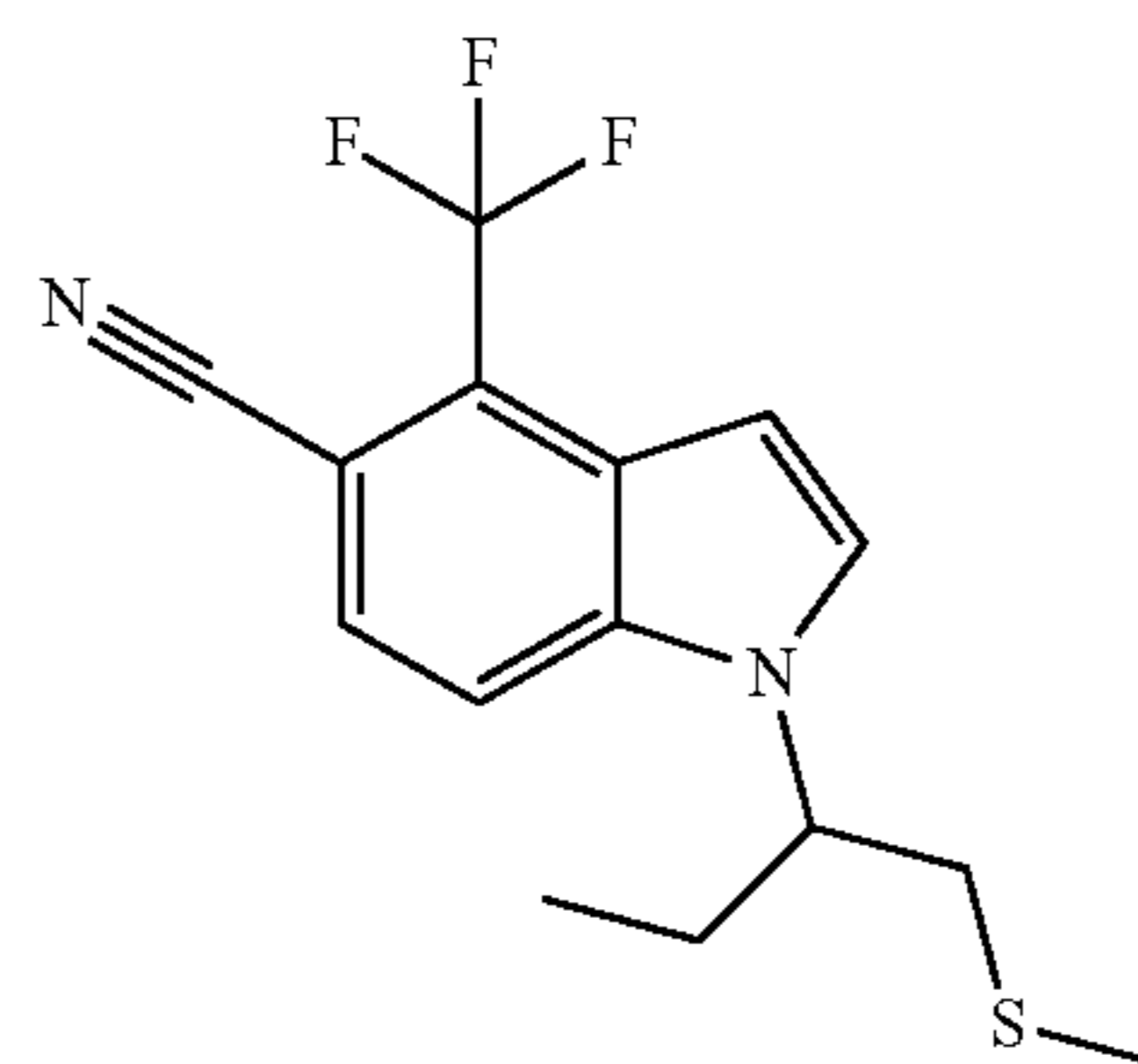
1-(1-(Methylthio)butan-2-yl)-4-(trifluoromethyl)-1H-indole-5-carbonitrile
