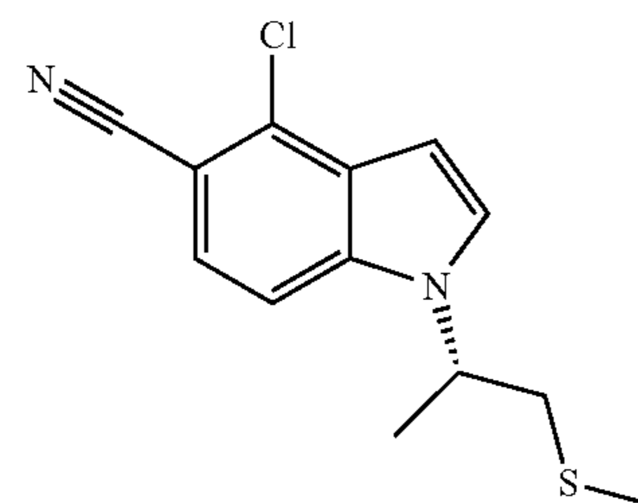
(S)-4-Chloro-1-(1-(methylthio)propan-2-yl)-1H-indole-5-carbonitrile
