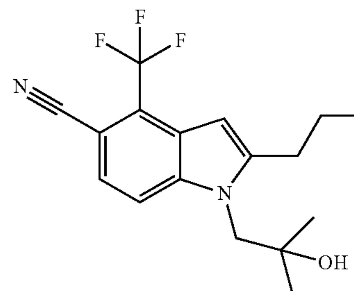
1-(2-Hydroxy-2-methylpropyl)-2-propyl-4-(trifluoromethyl)-1H-indole-5-carbonitrile
