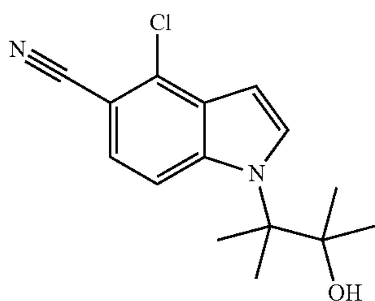
B. 4-Chloro-1-(3-hydroxy-2,3-dimethylbutan-2-yl)-1H-indole-5-carbonitrile
