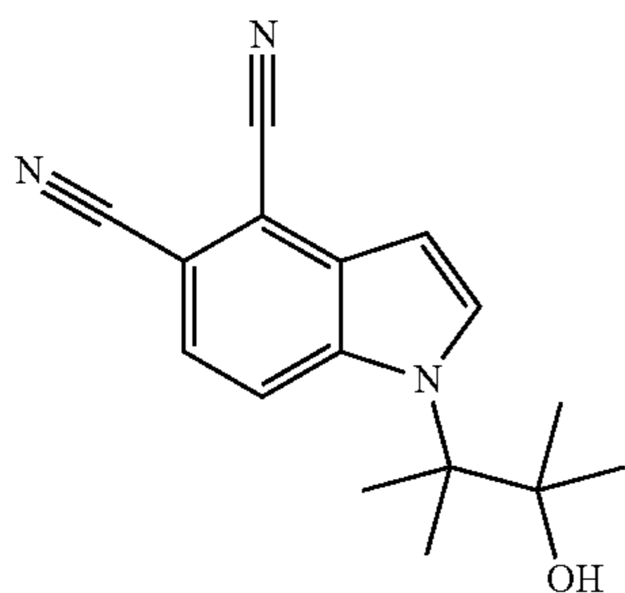
1-(3-Hydroxy-2,3-dimethylbutan-2-yl)-1H-indole-4,5-dicarbonitrile
