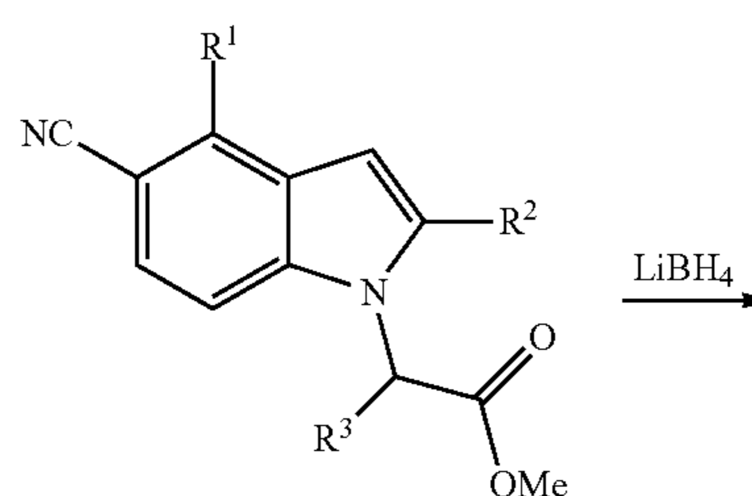
Scheme 2
