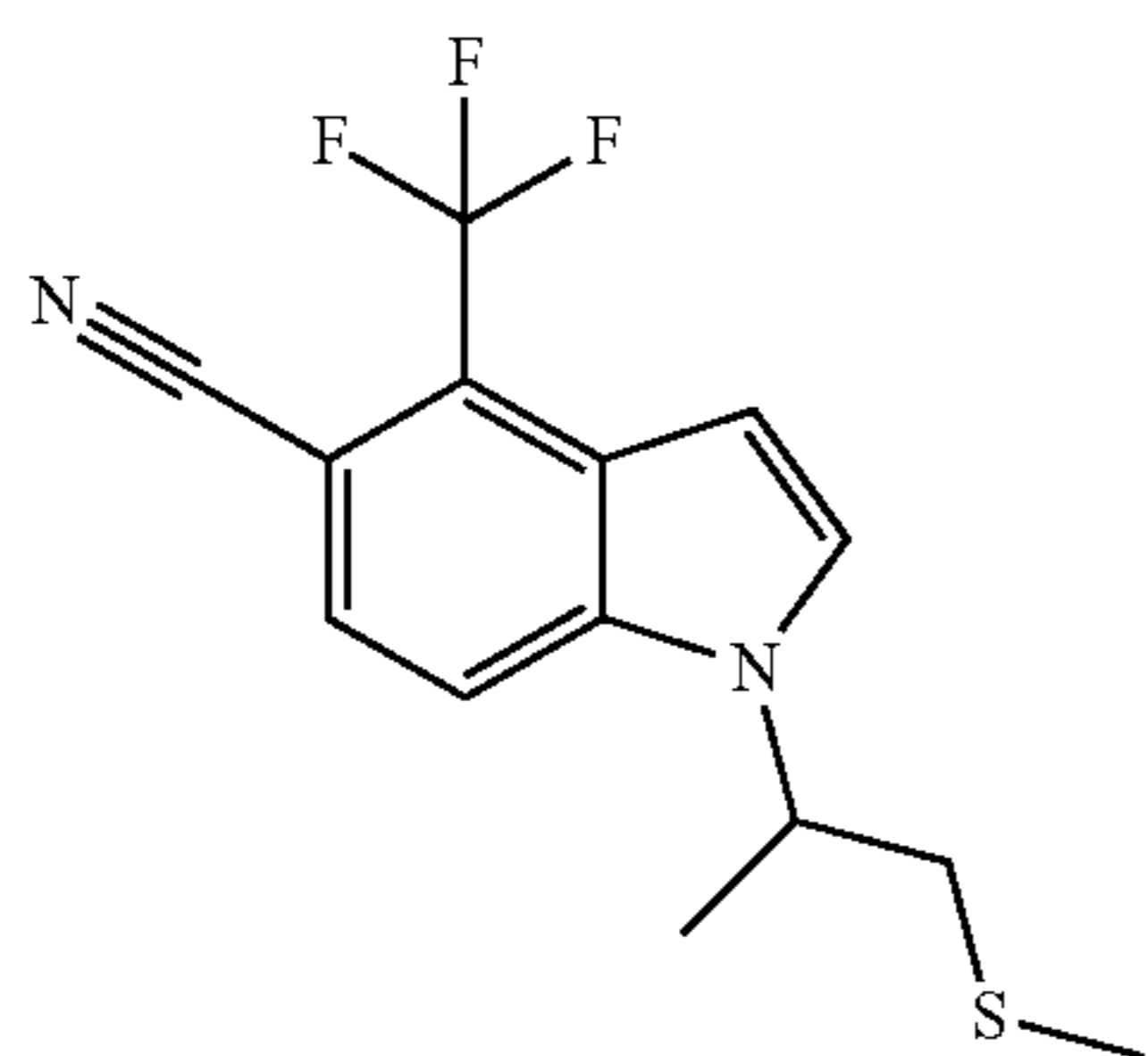
1-(1-(Methylthio)propan-2-yl)-4-(trifluoromethyl)-1H-indole-5-carbonitrile
