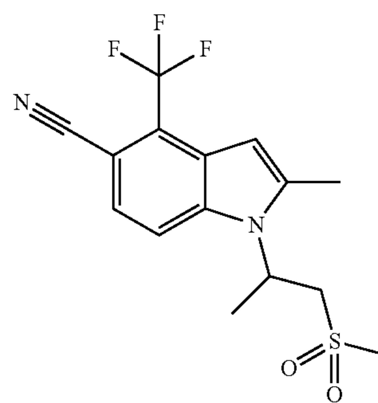
2-Methyl-1-(1-(methylsulfonyl)propan-2-yl)-4-(trifluoromethyl)-1H-indole-5-carbonitrile
