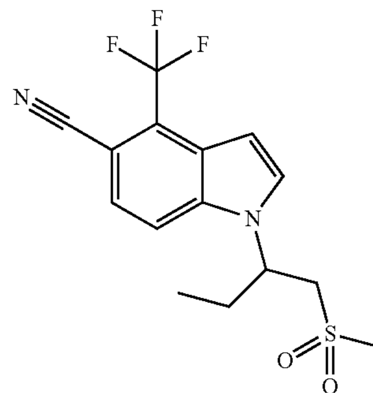
1-(1-(Methylsulfonyl)butan-2-yl)-4-(trifluoromethyl)-1H-indole-5-carbonitrile
