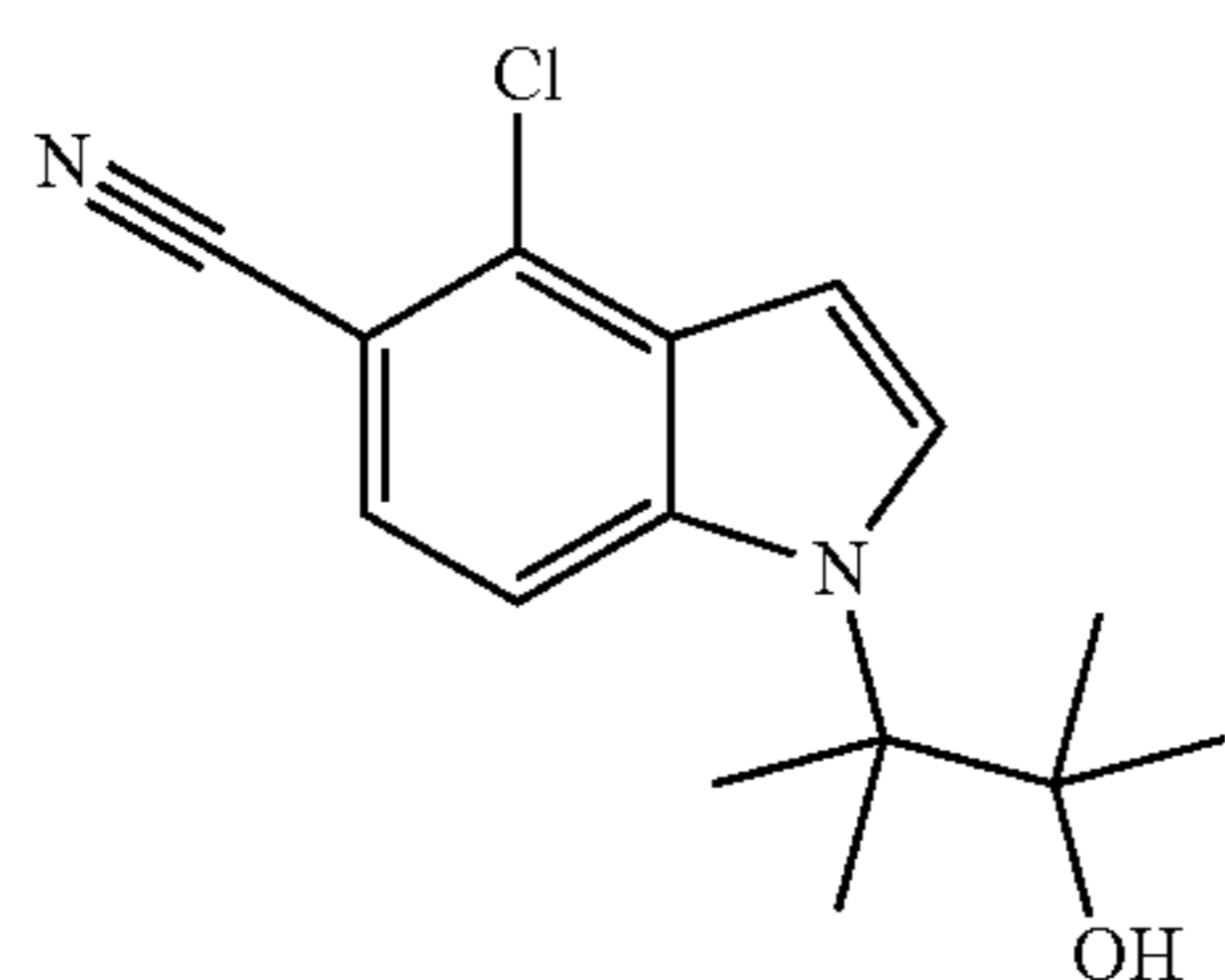
4-Chloro-1-(3-hydroxy-2,3-dimethylbutan-2-yl)-1H-indole-5-carbonitrile
