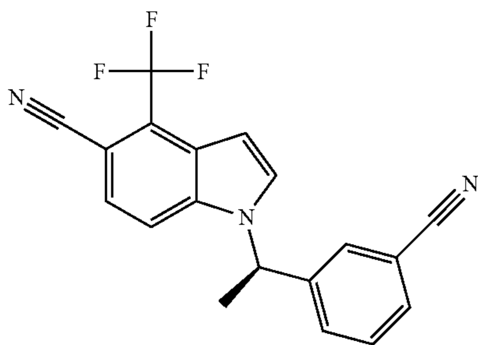
(R)-1-(1-(3-Cyanophenyl)ethyl)-4-(trifluoromethyl)-1H-indole-5-carbonitrile
