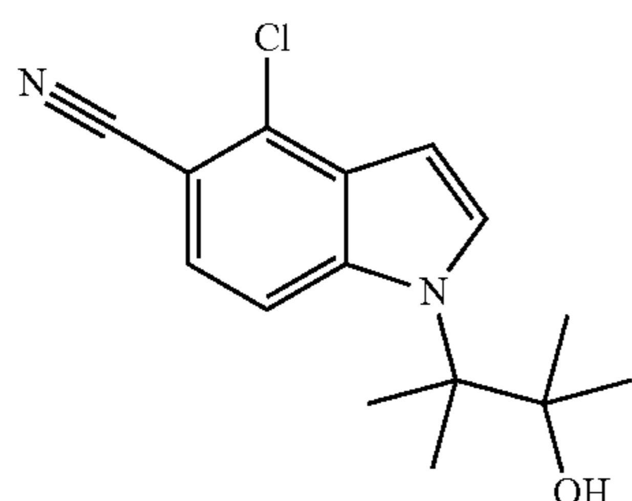
B. 4-Chloro-1-(3-hydroxy-2,3-dimethylbutan-2-yl)-1H-indole-5-carbonitrile
