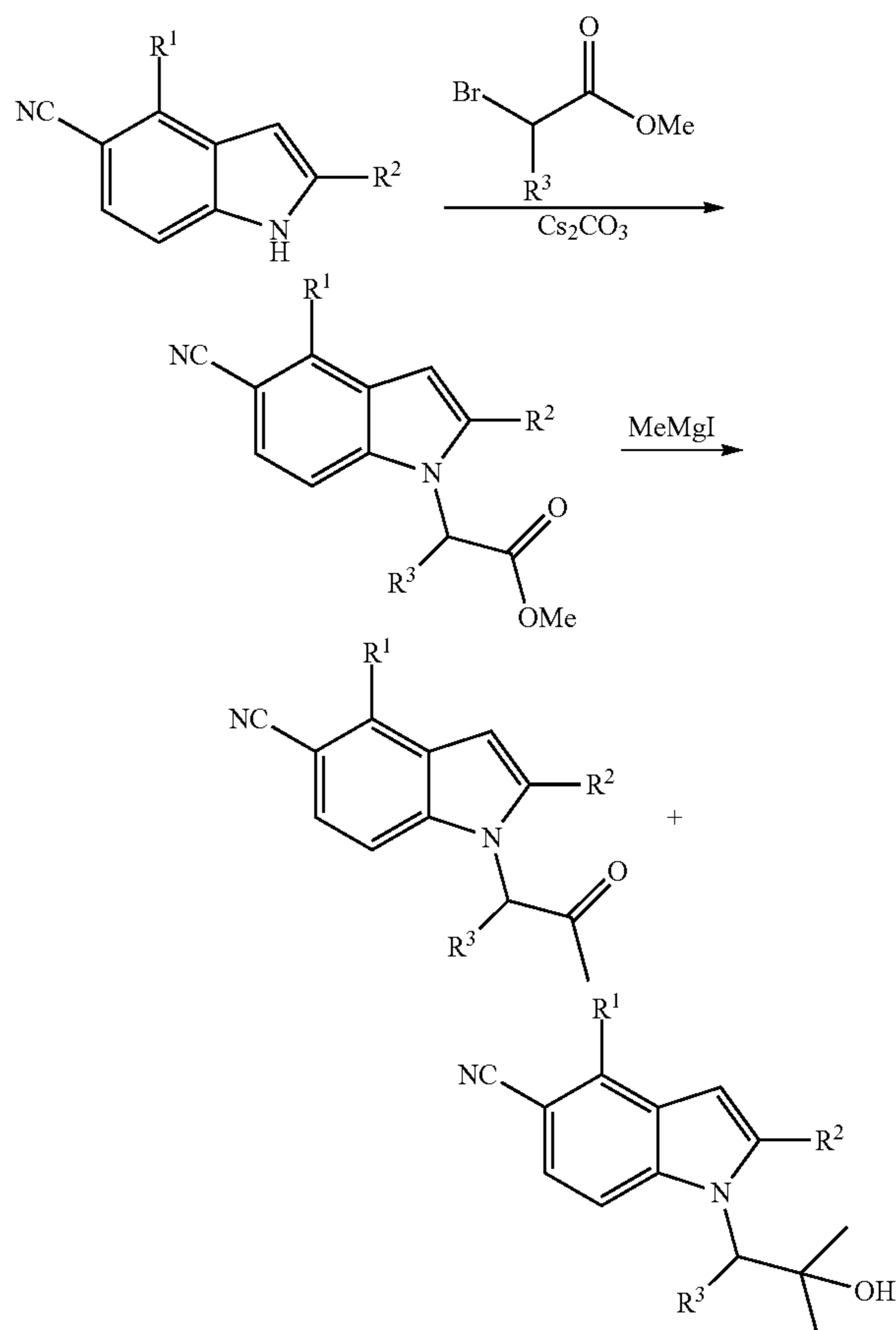
Scheme 1
