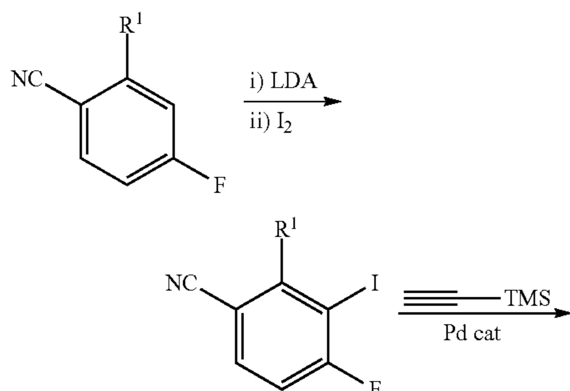
Scheme 3
