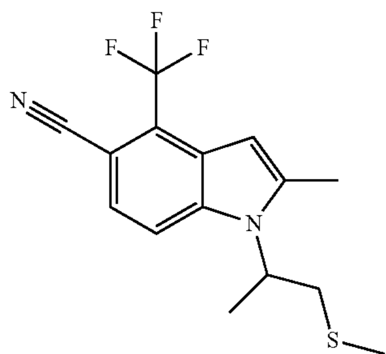
2-Methyl-1-(1-(methylthio)propan-2-yl)-4-(trifluoromethyl)-1H-indole-5-carbonitrile
