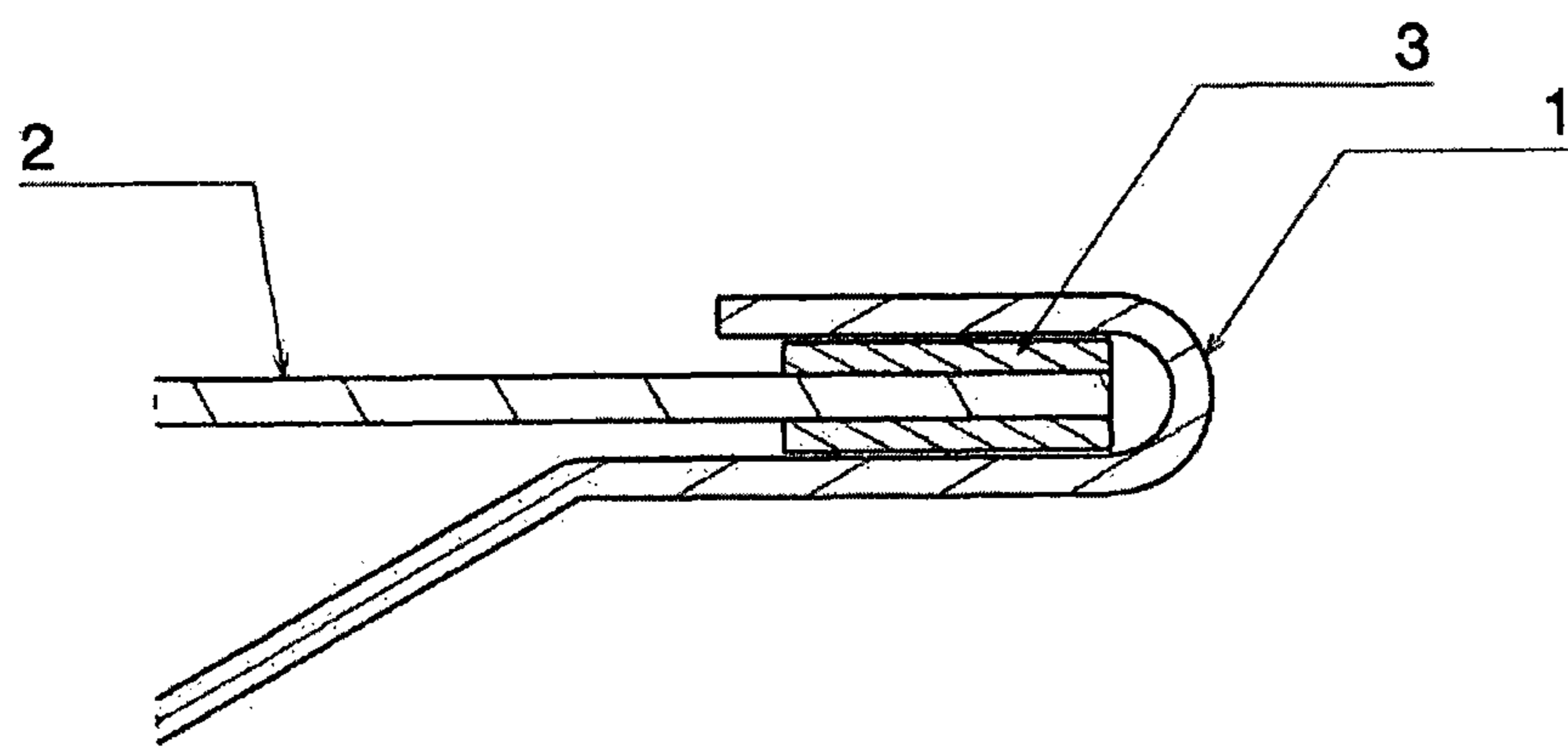
Figure 2 (PRIOR ART)
