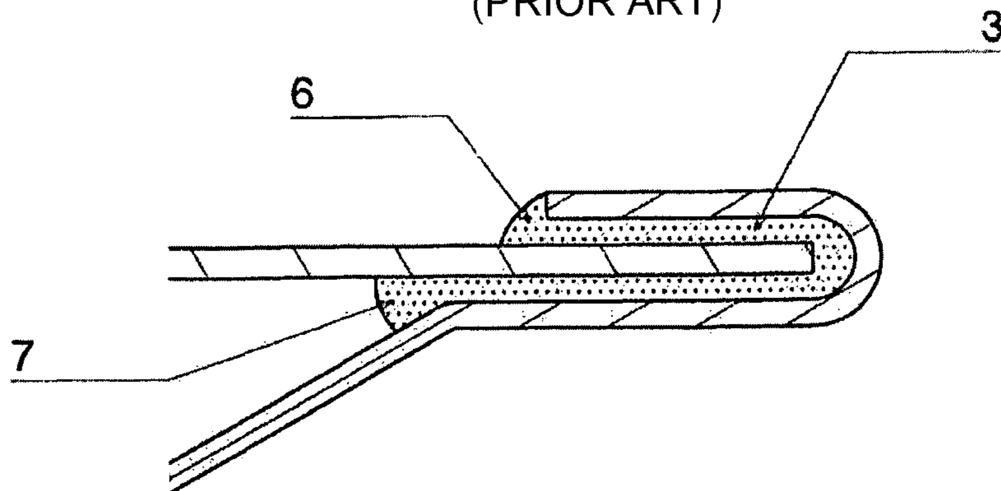
Figure 3 (PRIOR ART)
