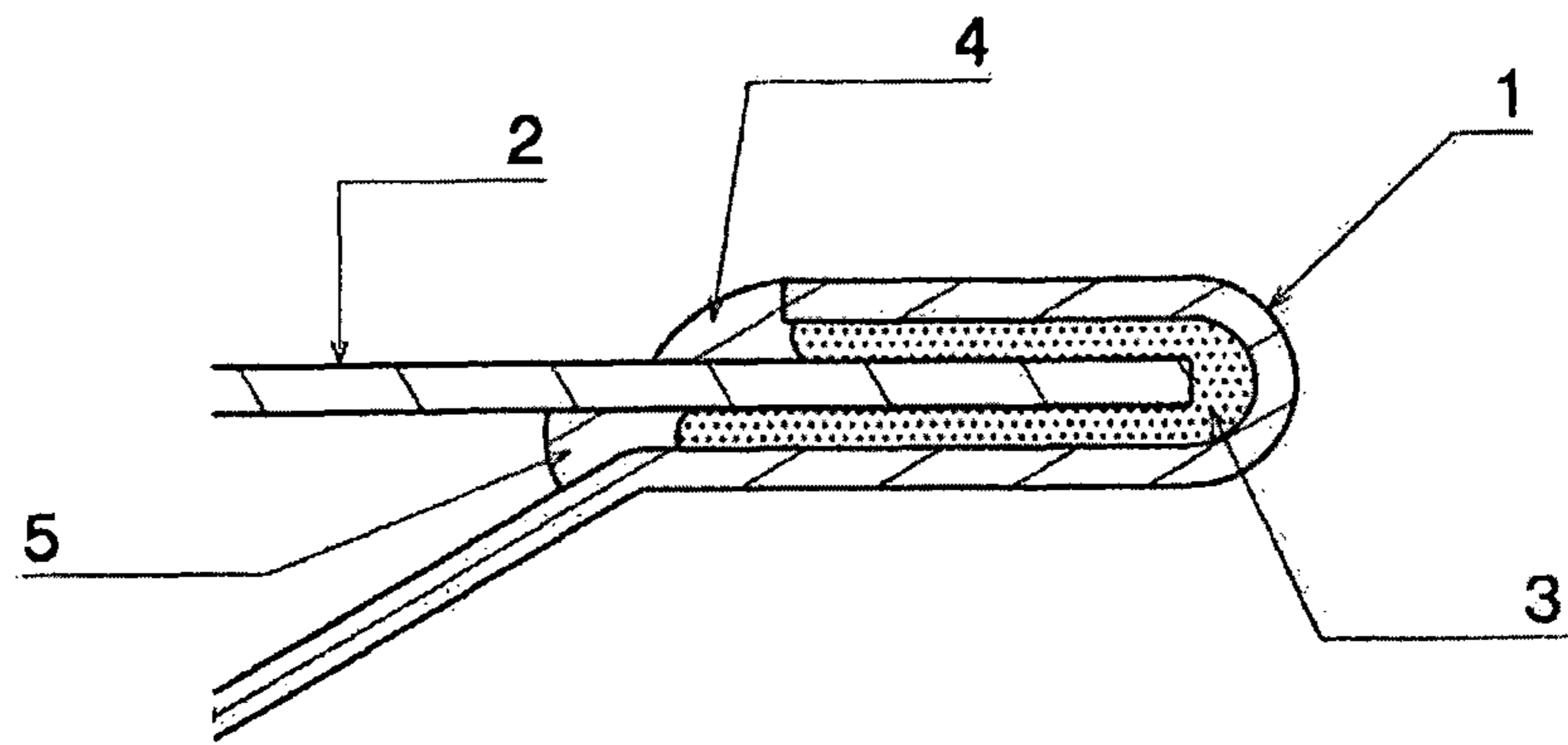
Figure 1 (PRIOR ART)
