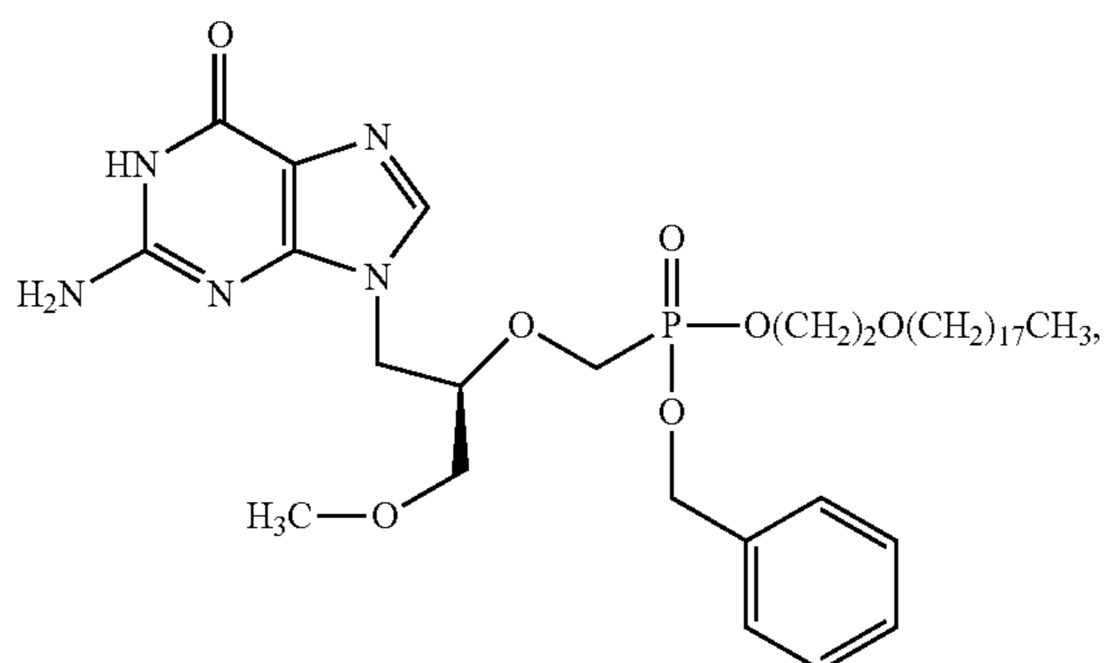
benzyl octadecyloxyethyl 9-(R)-[3-methoxy-2-(phosphonomethoxy)propyl] guanine
