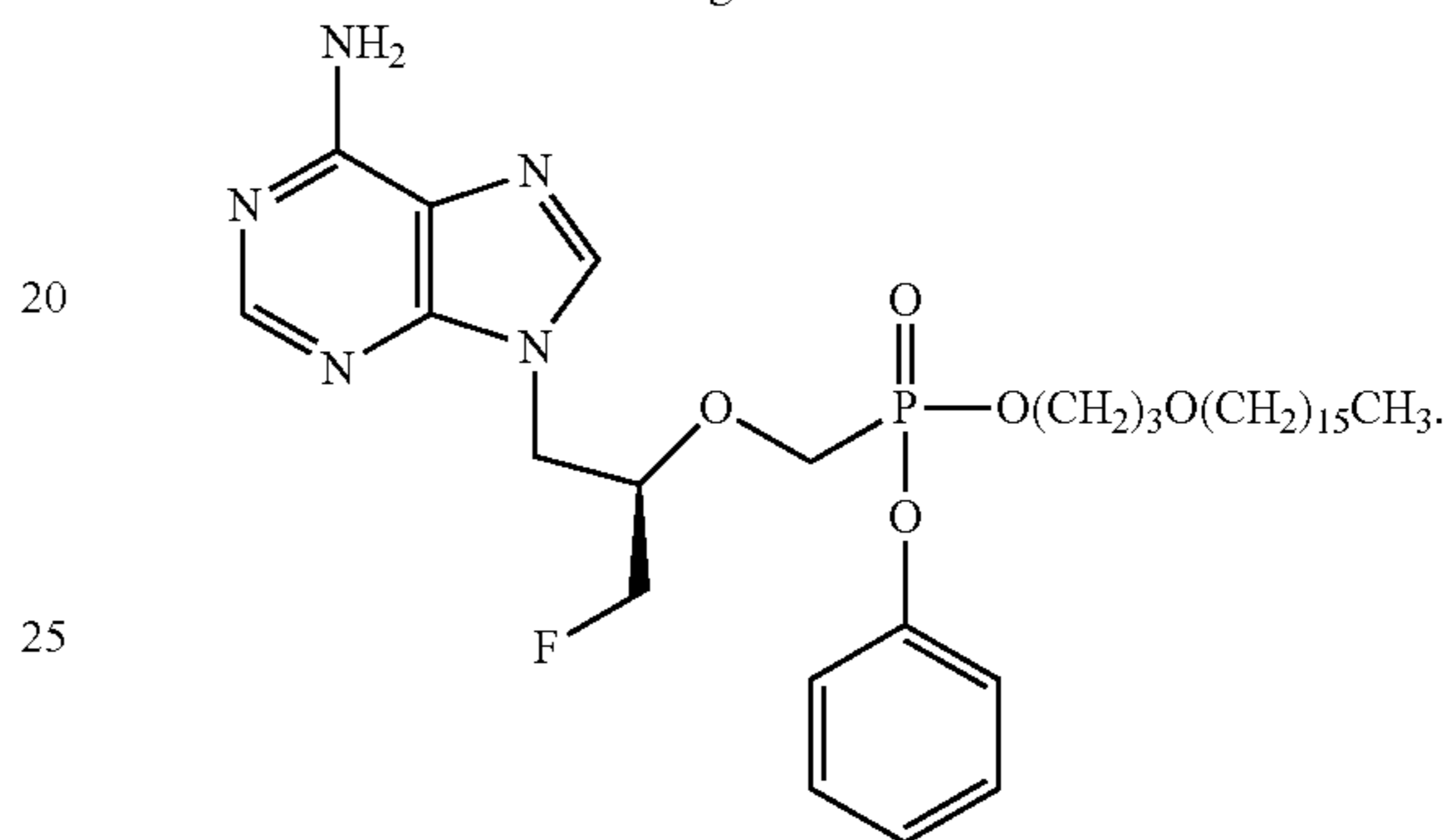
phenyl hexadecyloxypropyl 9-(R)-[3-fluoro-2-(phosphonomethoxy)propyl] adenine
