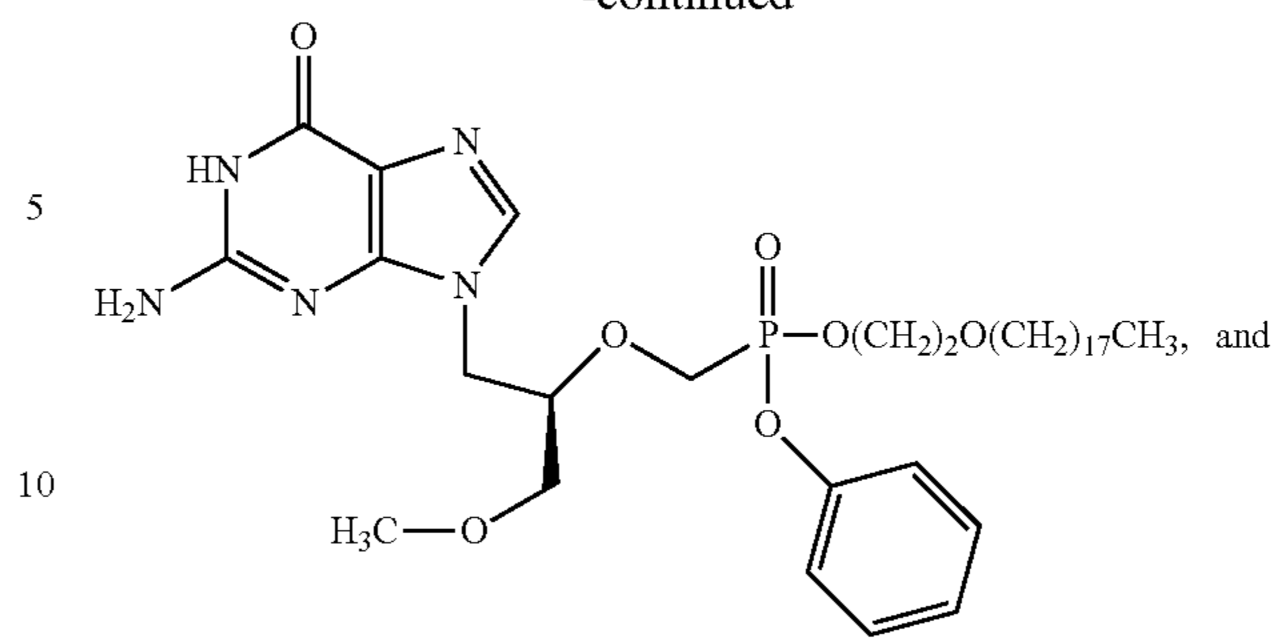
Phenyl octadecyloxyethyl 9-(R)-[3-methoxy-2-(phosphonomethoxy)propyl] guanine
