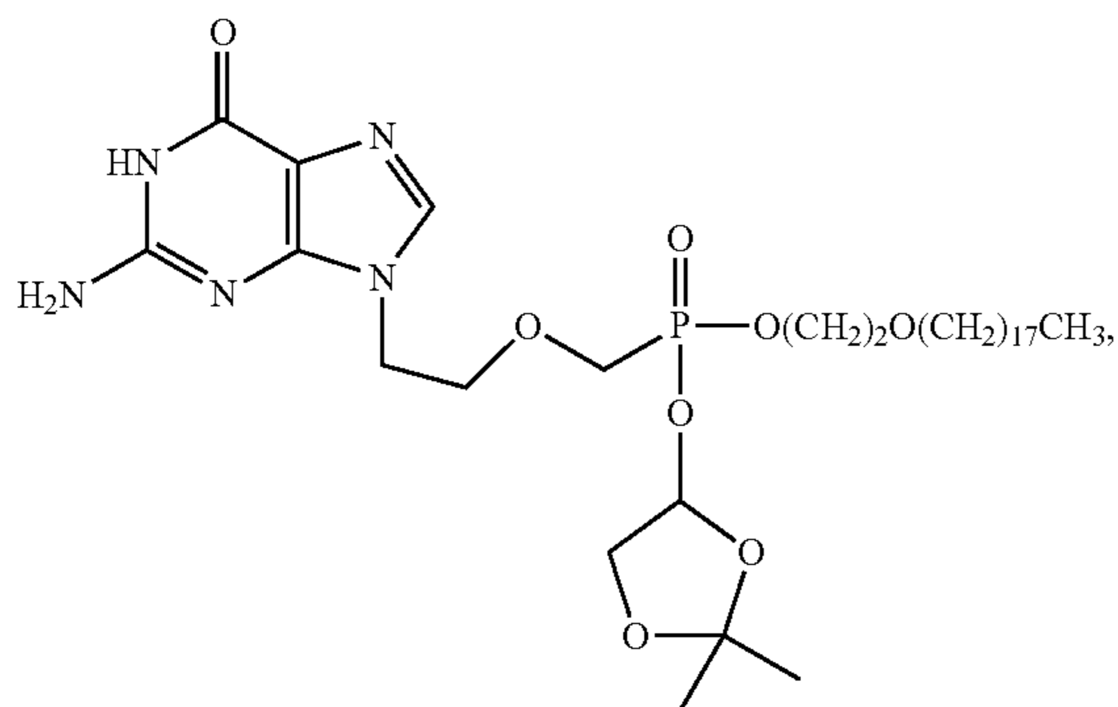
isopropylidenglyceryl octadecyloxyethyl 9-[2-(phosphonomethoxy)ethyl]guanine
