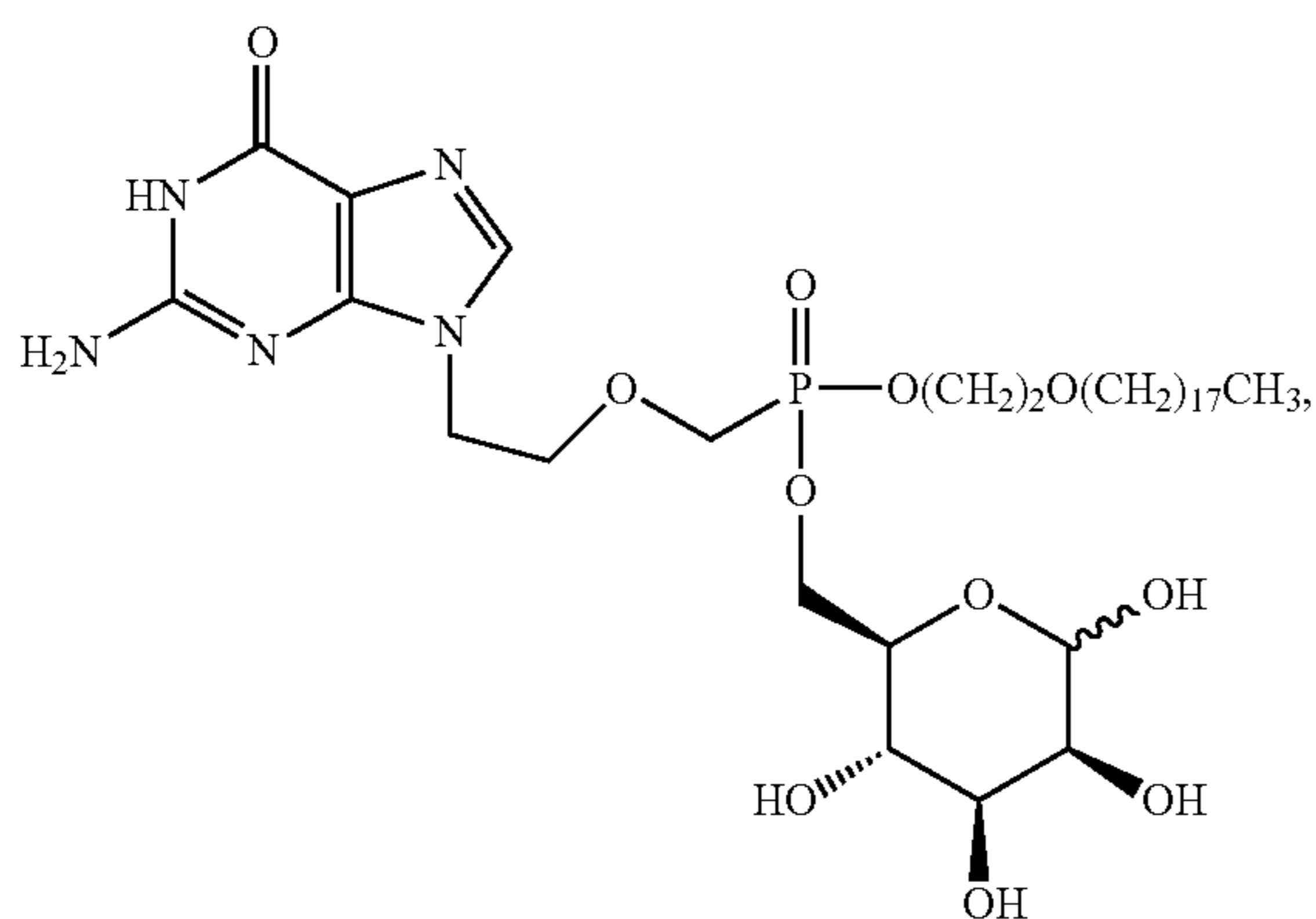
mannosyl octadecyloxyethyl 9-[2-(phosphonomethoxy)ethyl]guanine
