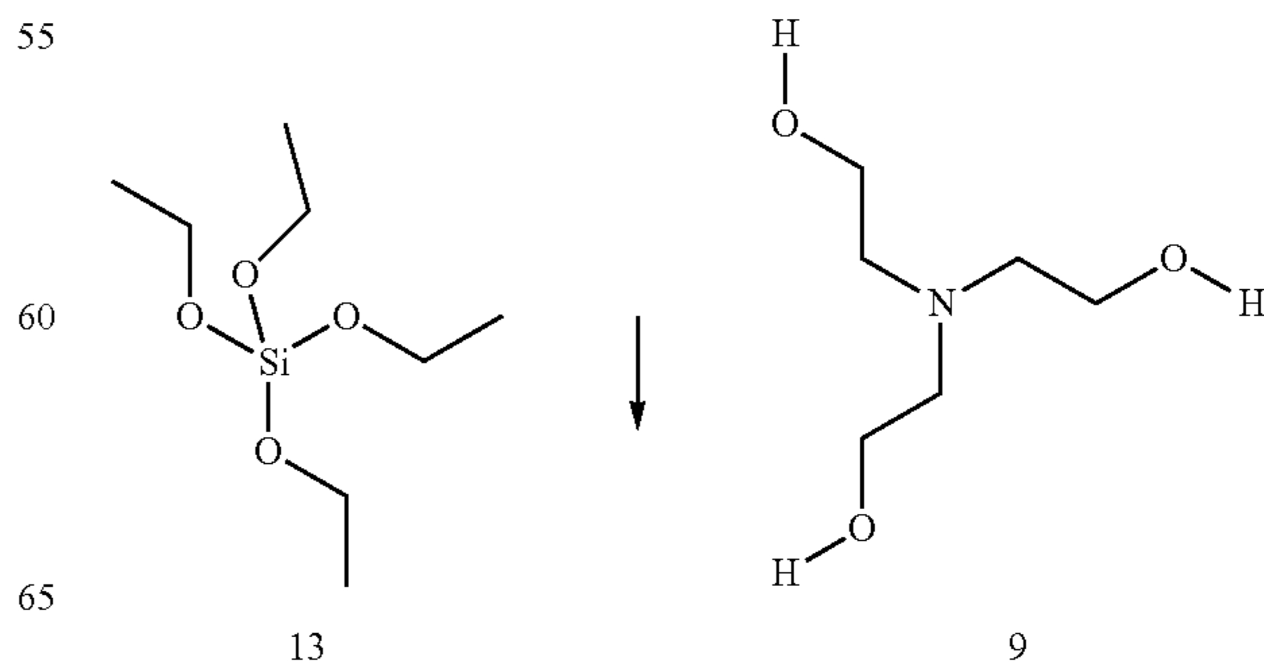
REACTION SCHEME 5
