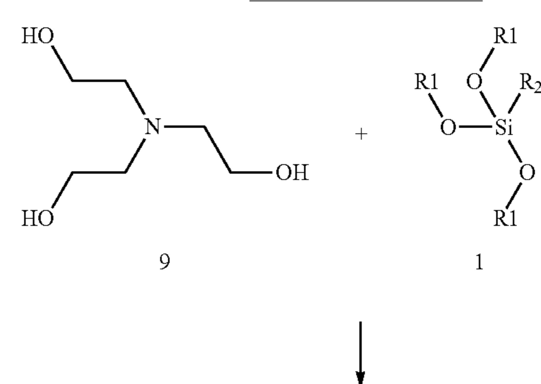
REACTION SCHEME 2
