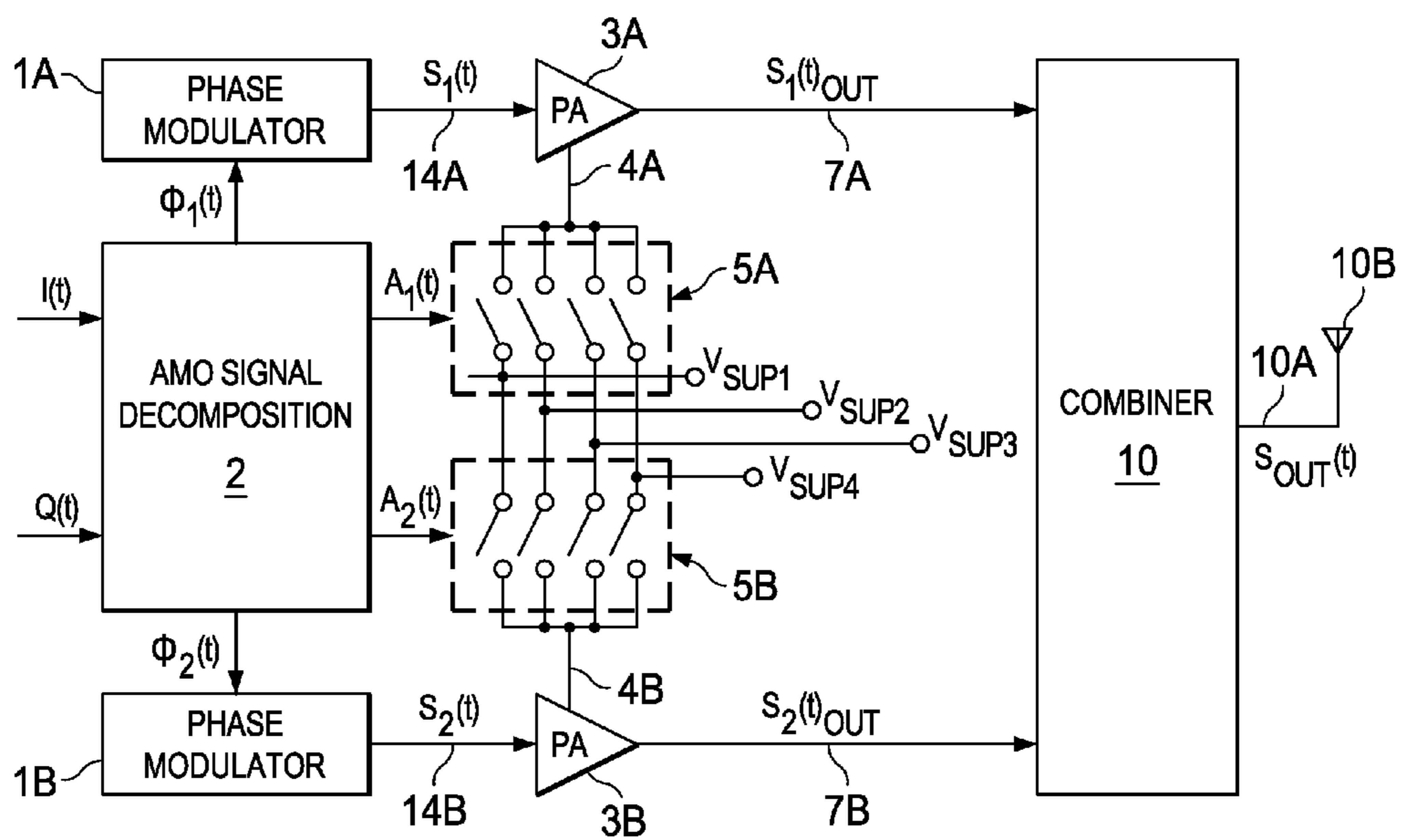
FIG. 2 (PRIOR ART)
