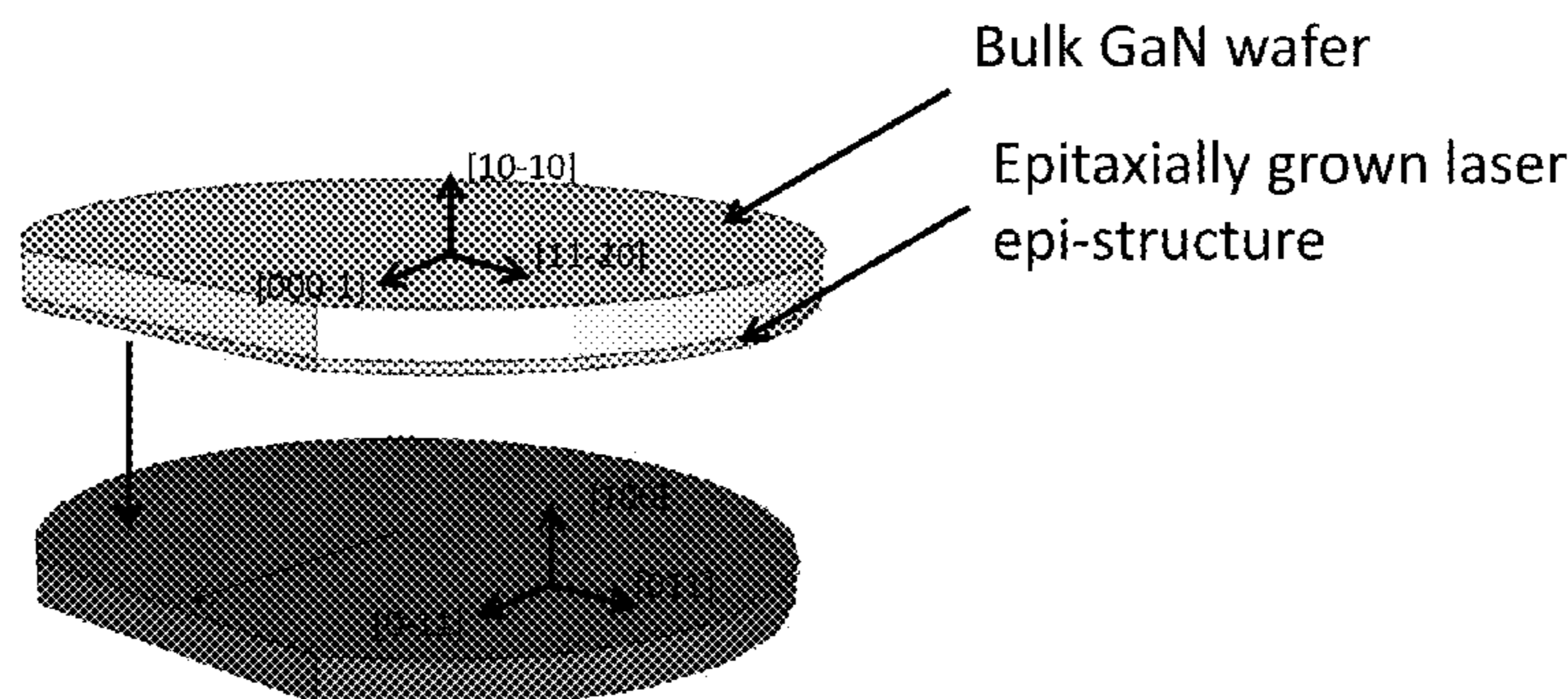
Handle wafer assisted cleaving
