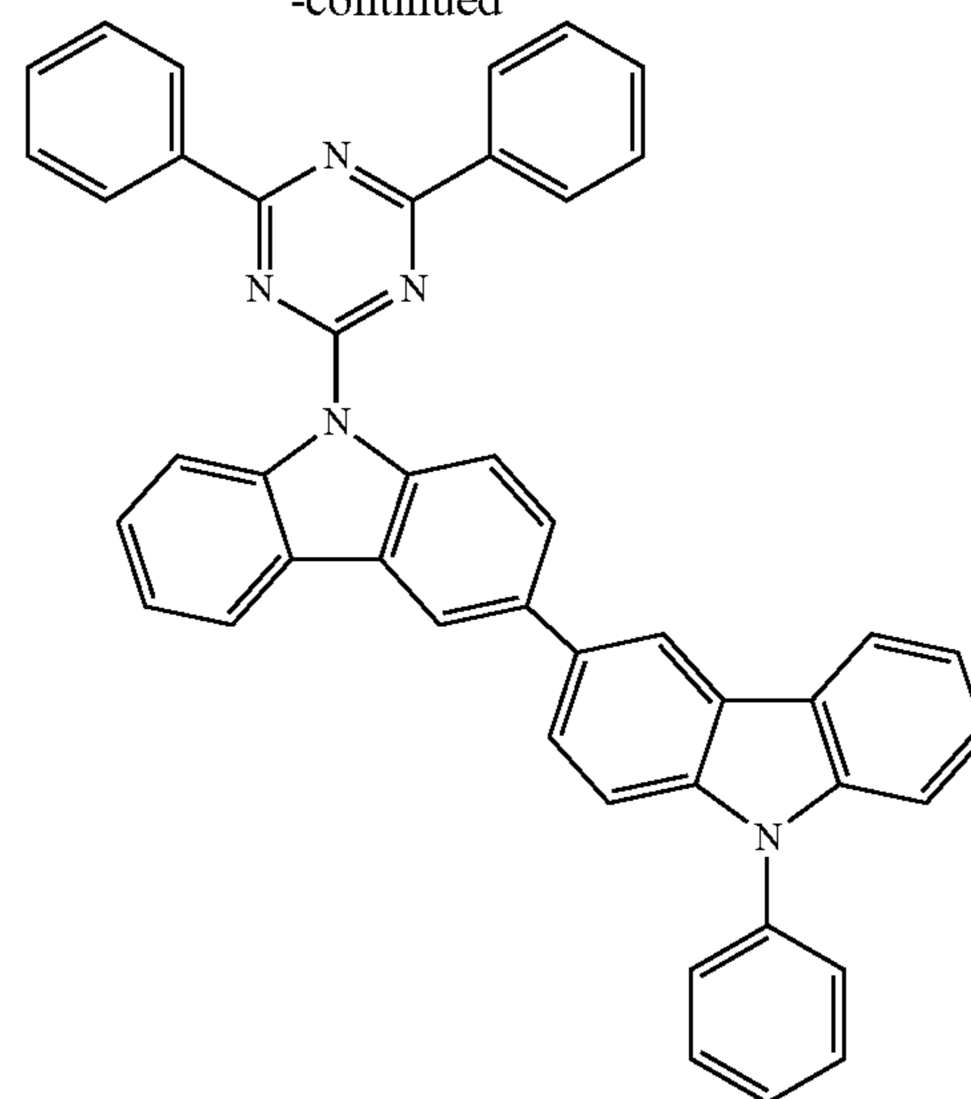
Compound 5
