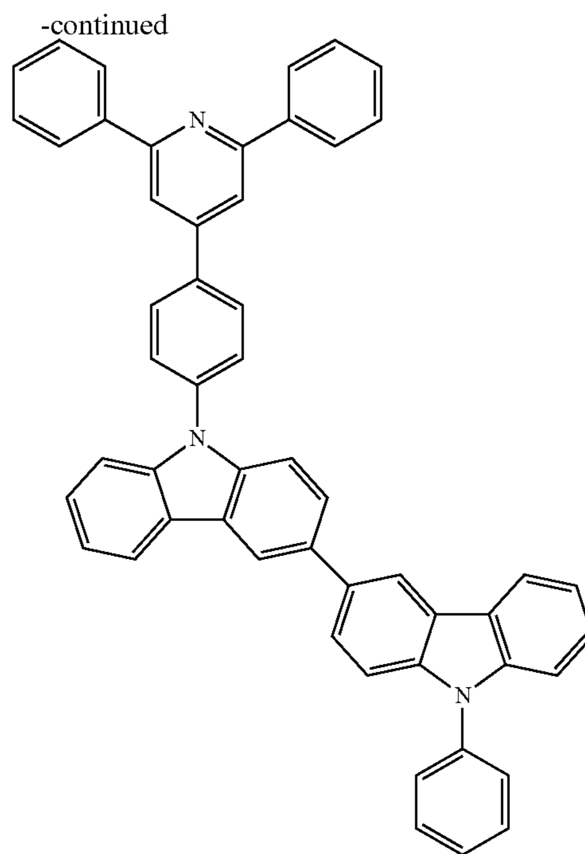
Compound 2
