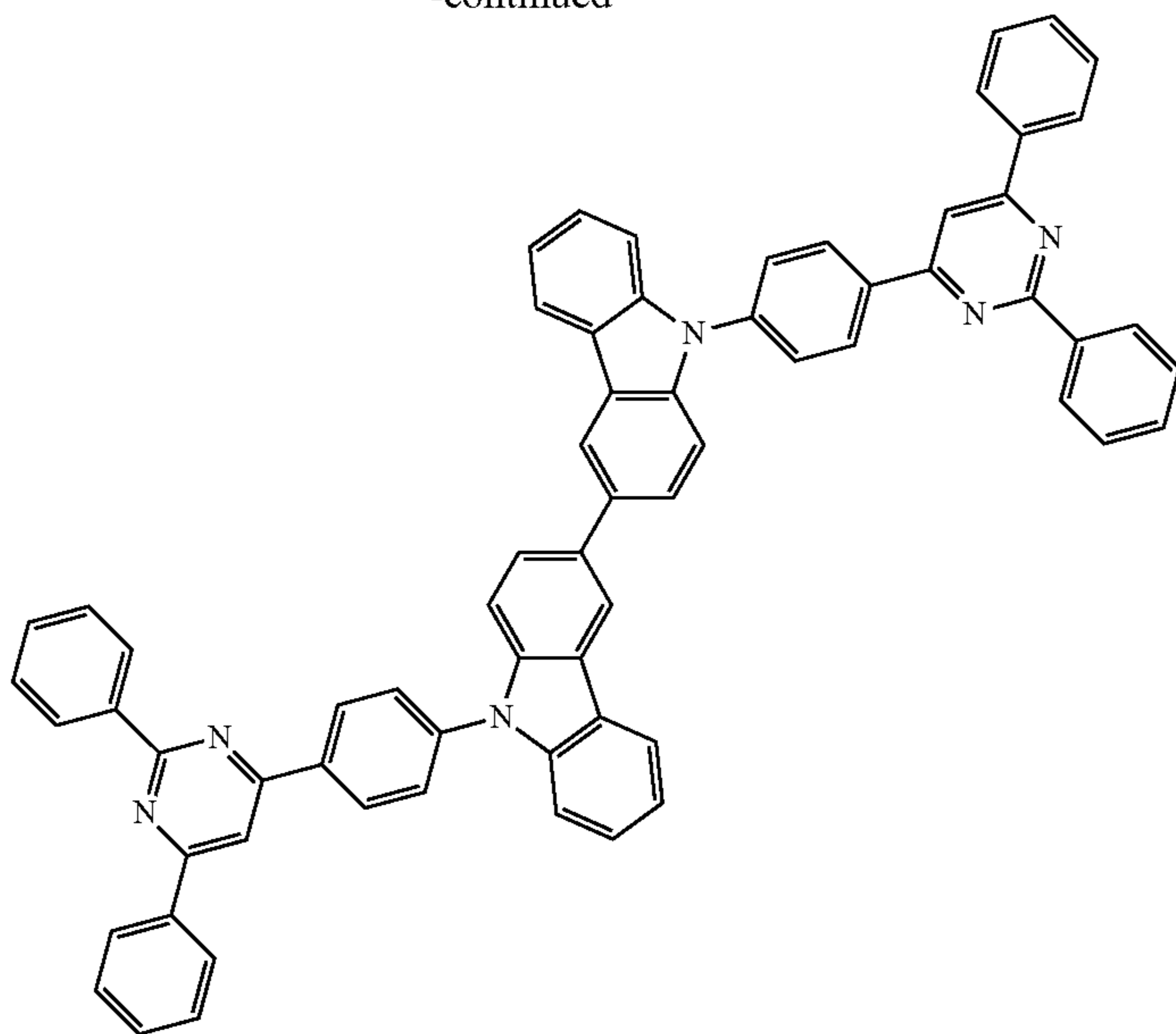
Compound 4
