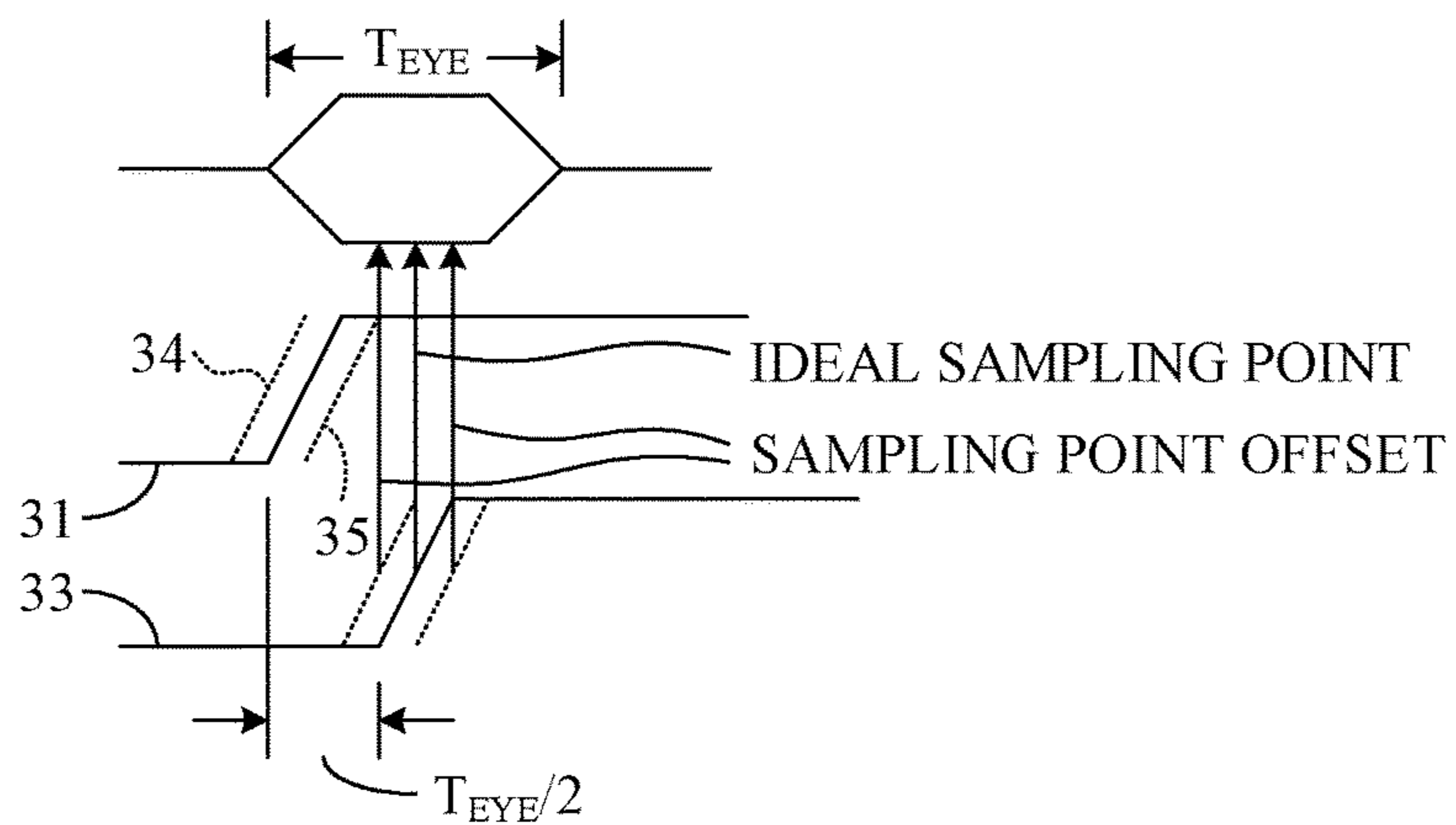
FIG. 2 (Prior Art)
