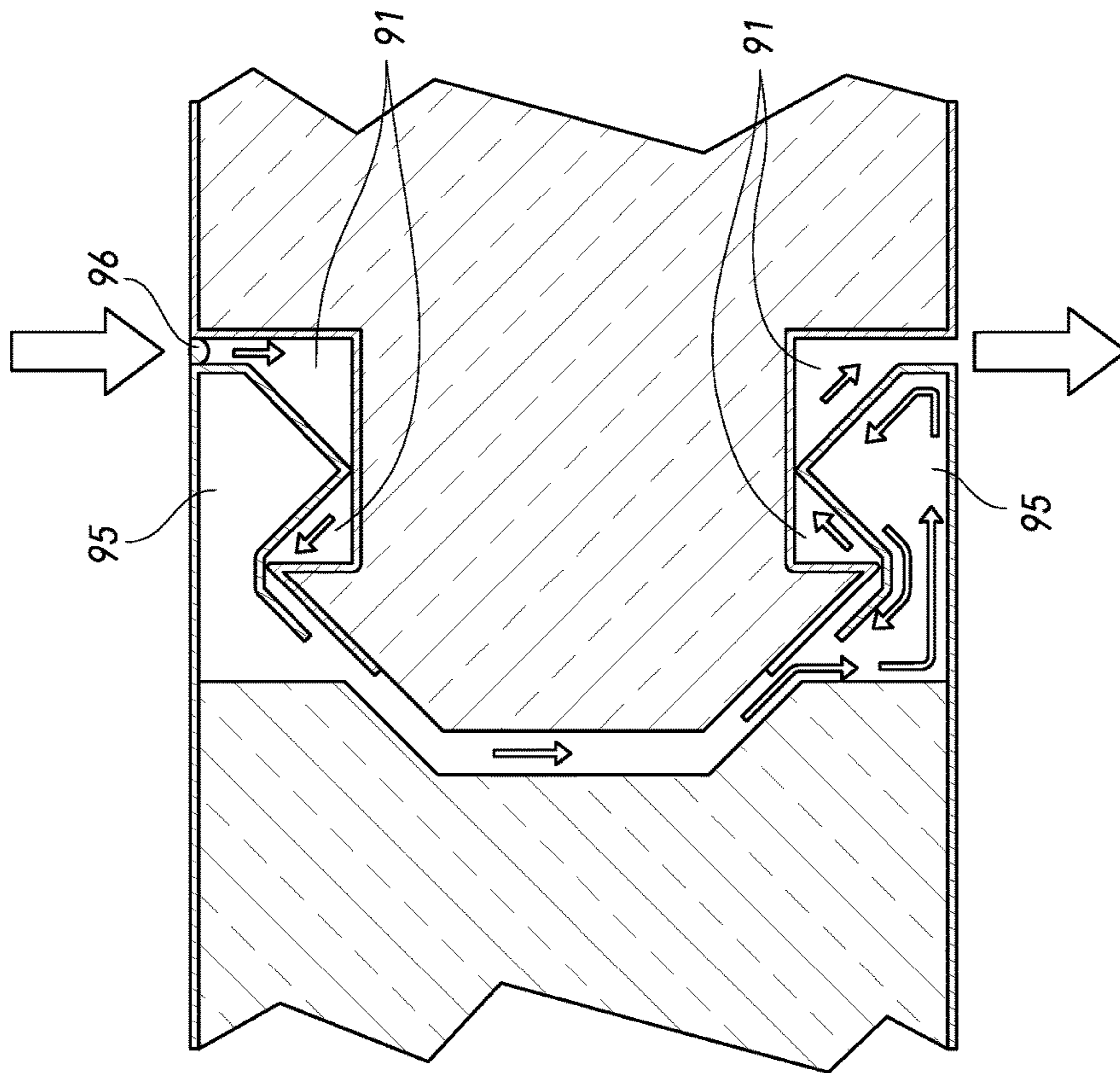
FIG. 10 (PRIOR ART)
