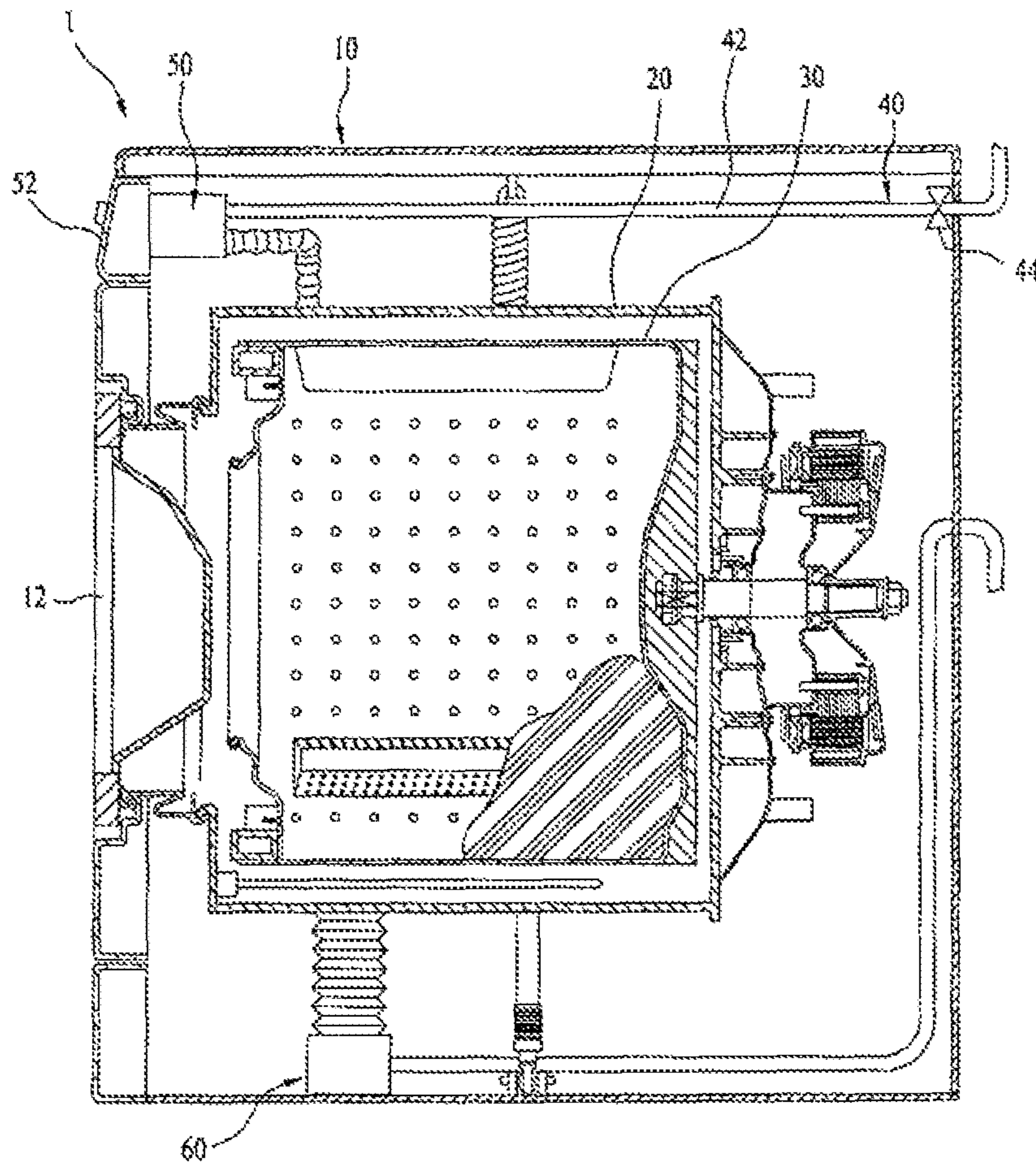
FIG. 1 CONVENTIONAL ART
