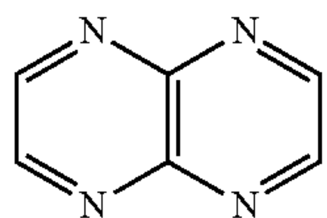
pyrazino[2,3-b]pyrazine
