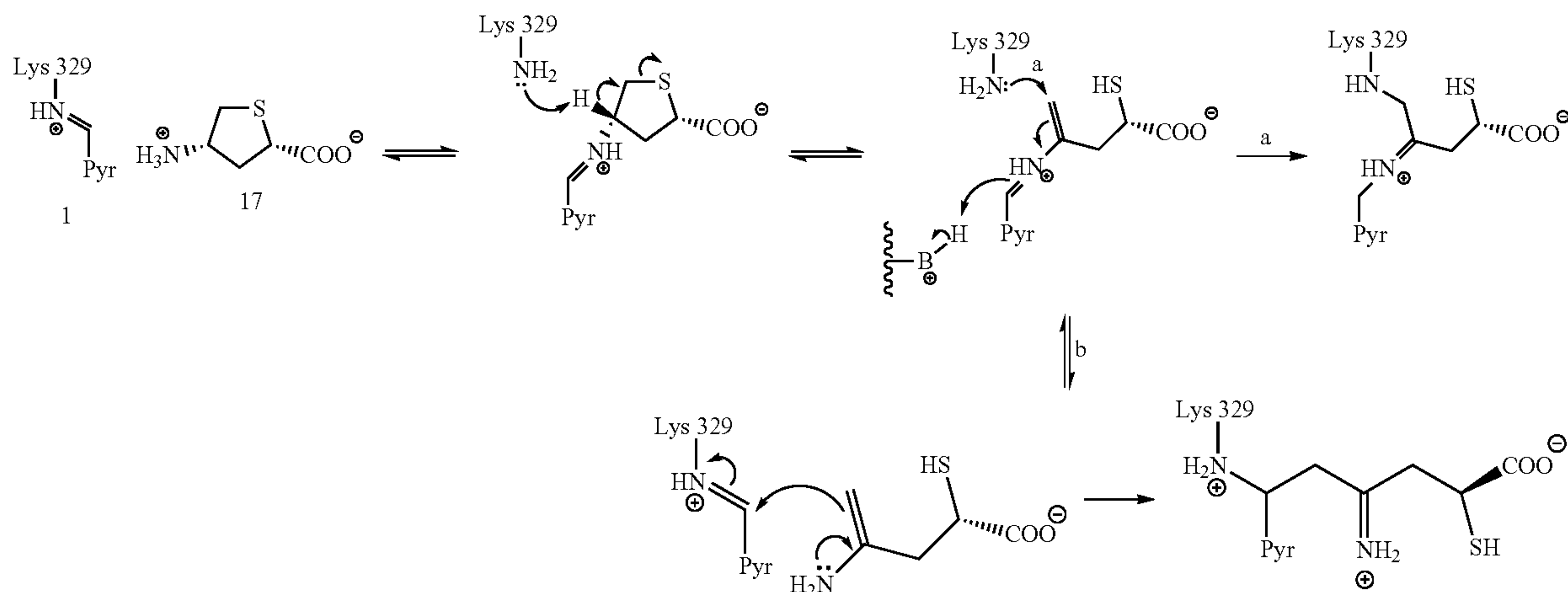
Scheme 2. Michael addition (pathway a) and enamine addition (pathway b) mechanisms for 17
