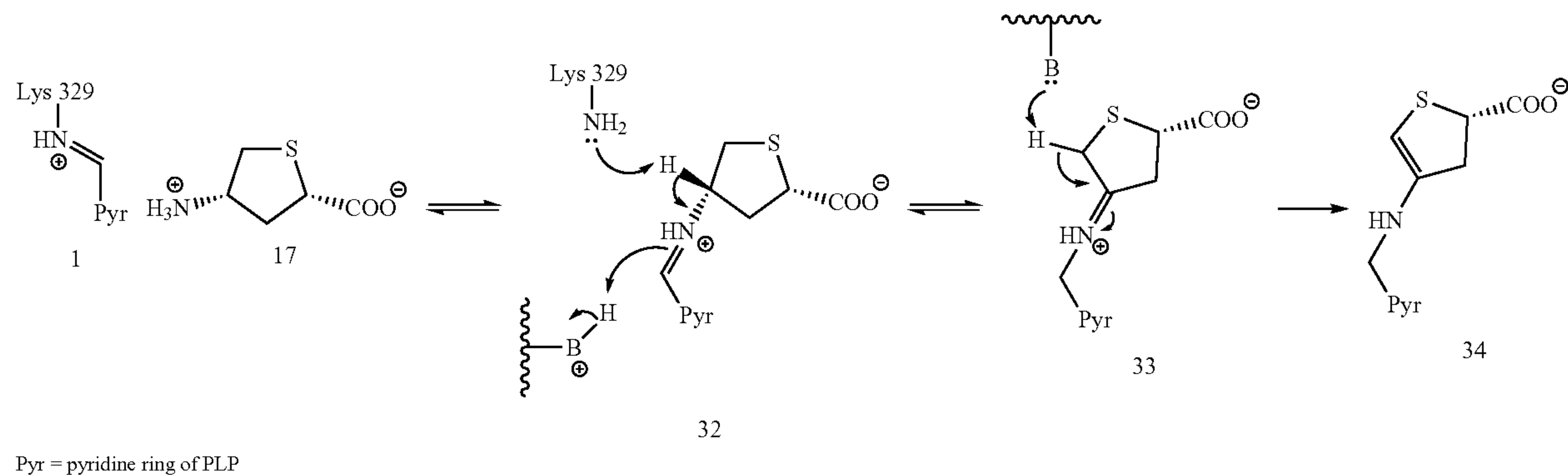
Scheme 4. Proposed mechanism for the inactivation of GABA-AT by 17
