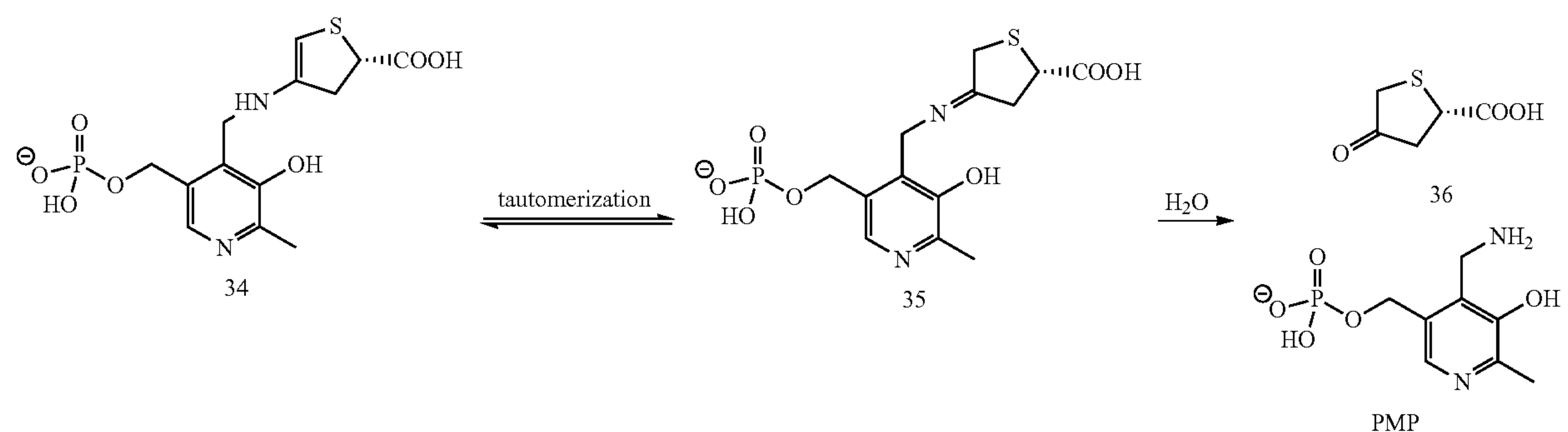
Scheme 5. Hydrolysis of Metabolite 34
