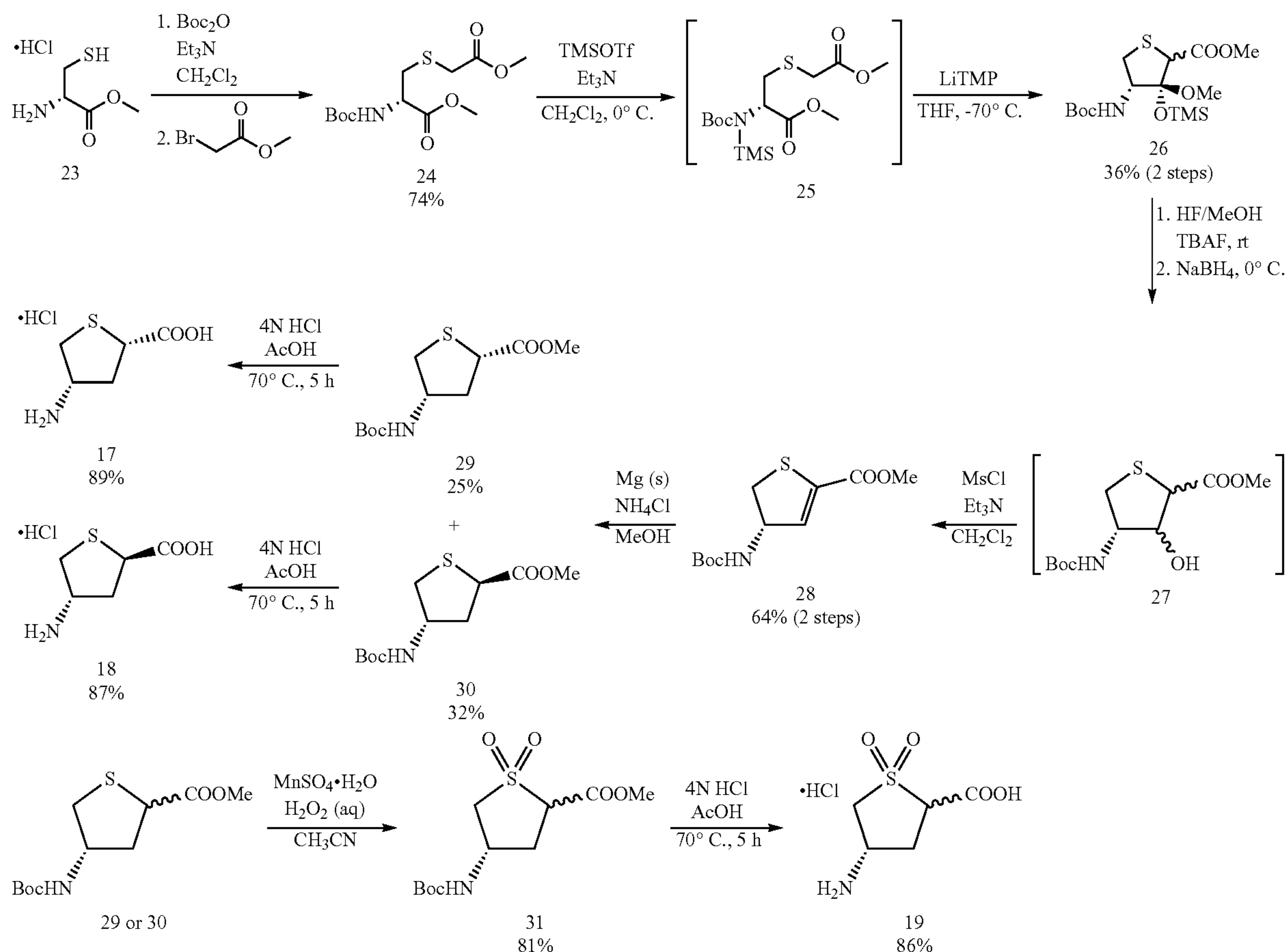
Scheme 3. Syntheses of GABA Analogs 17-19
