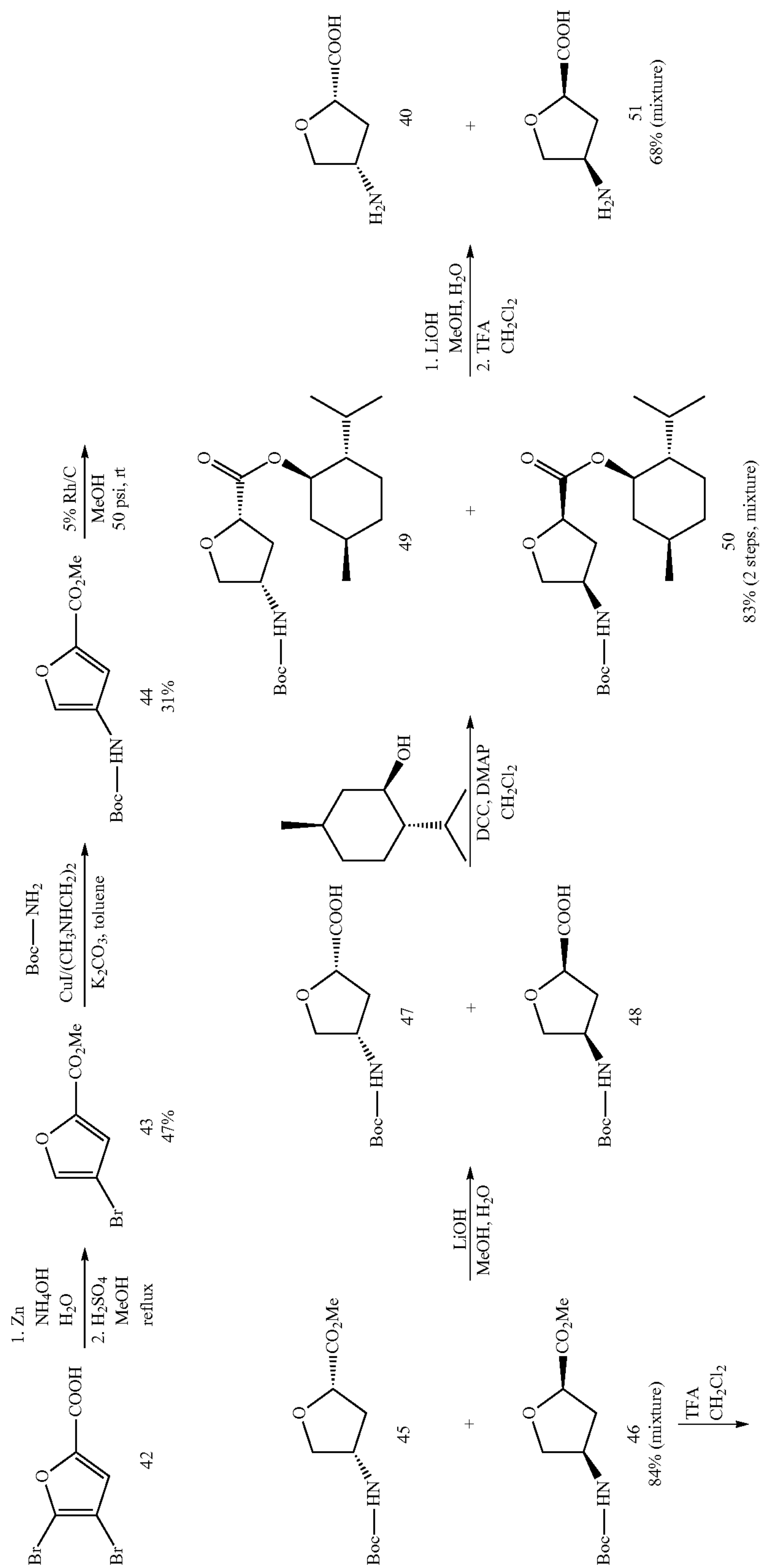
Scheme 7. Synthesis of Tetrahydrofuran Analog 40
