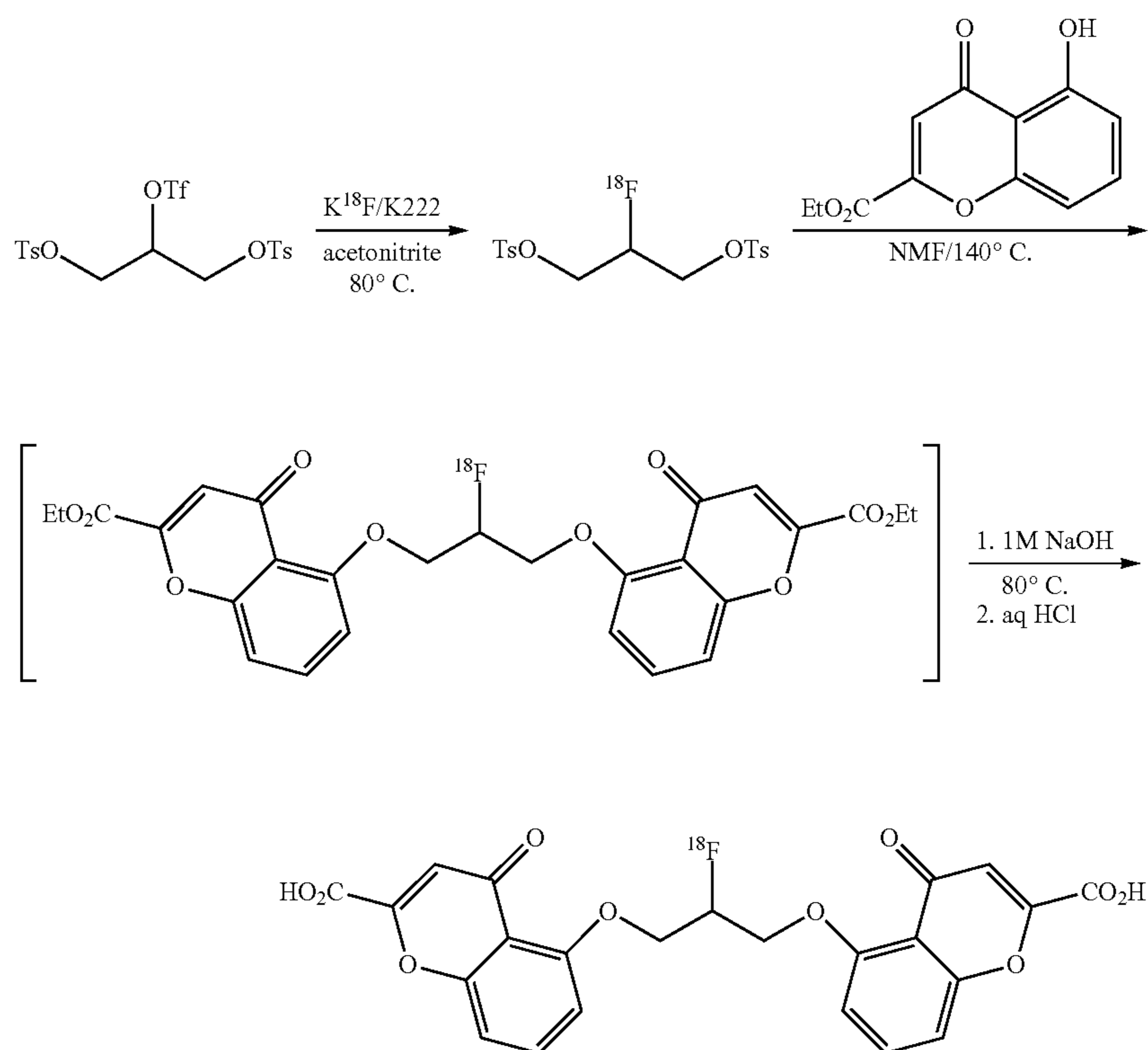
Radiofluorination - Scheme 1
