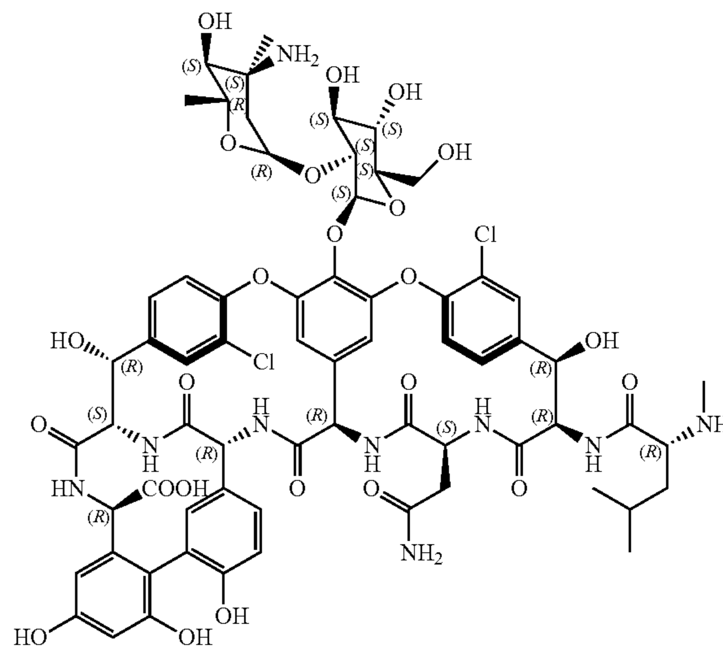
Formula 1
