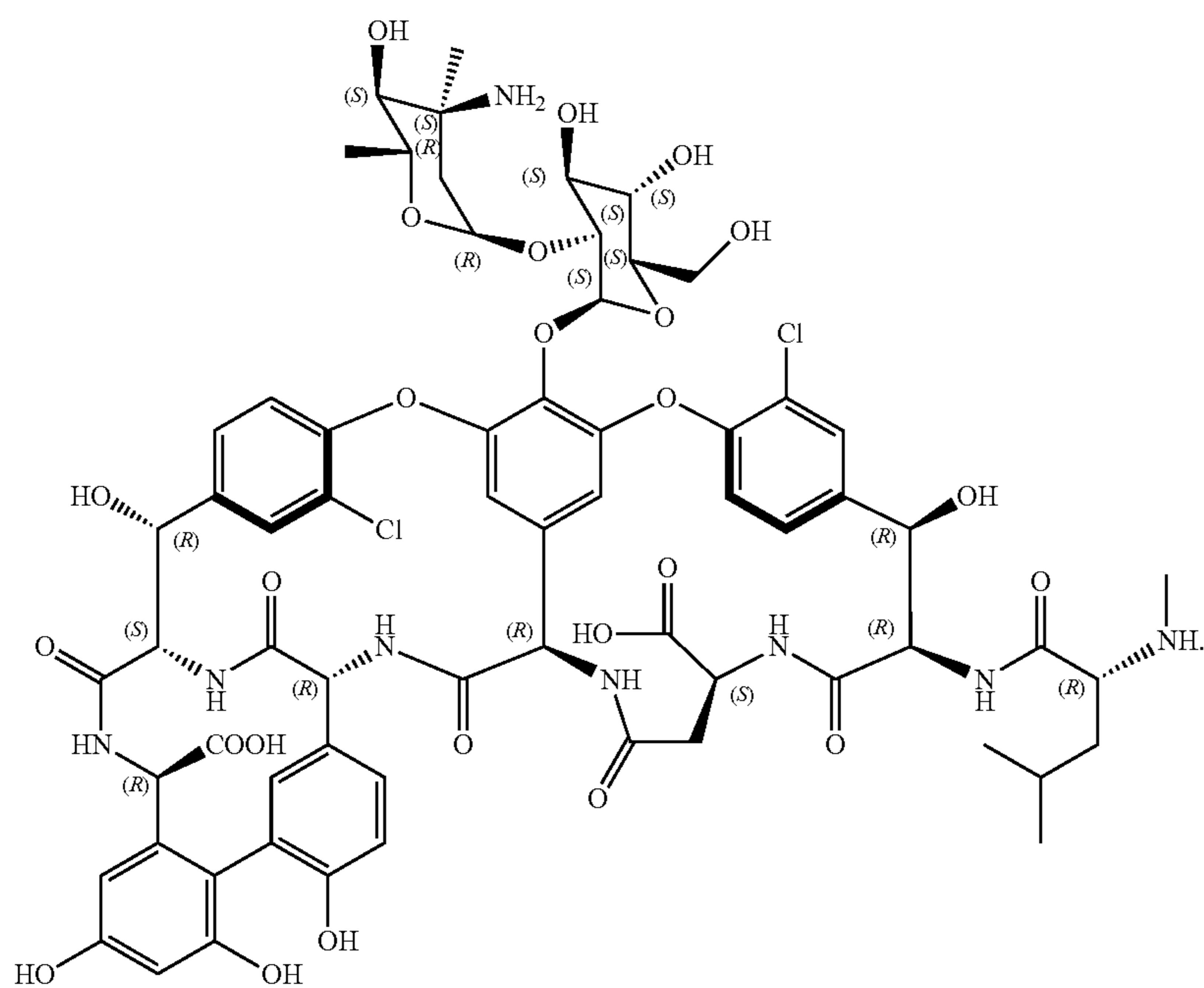
CDP1 minor
