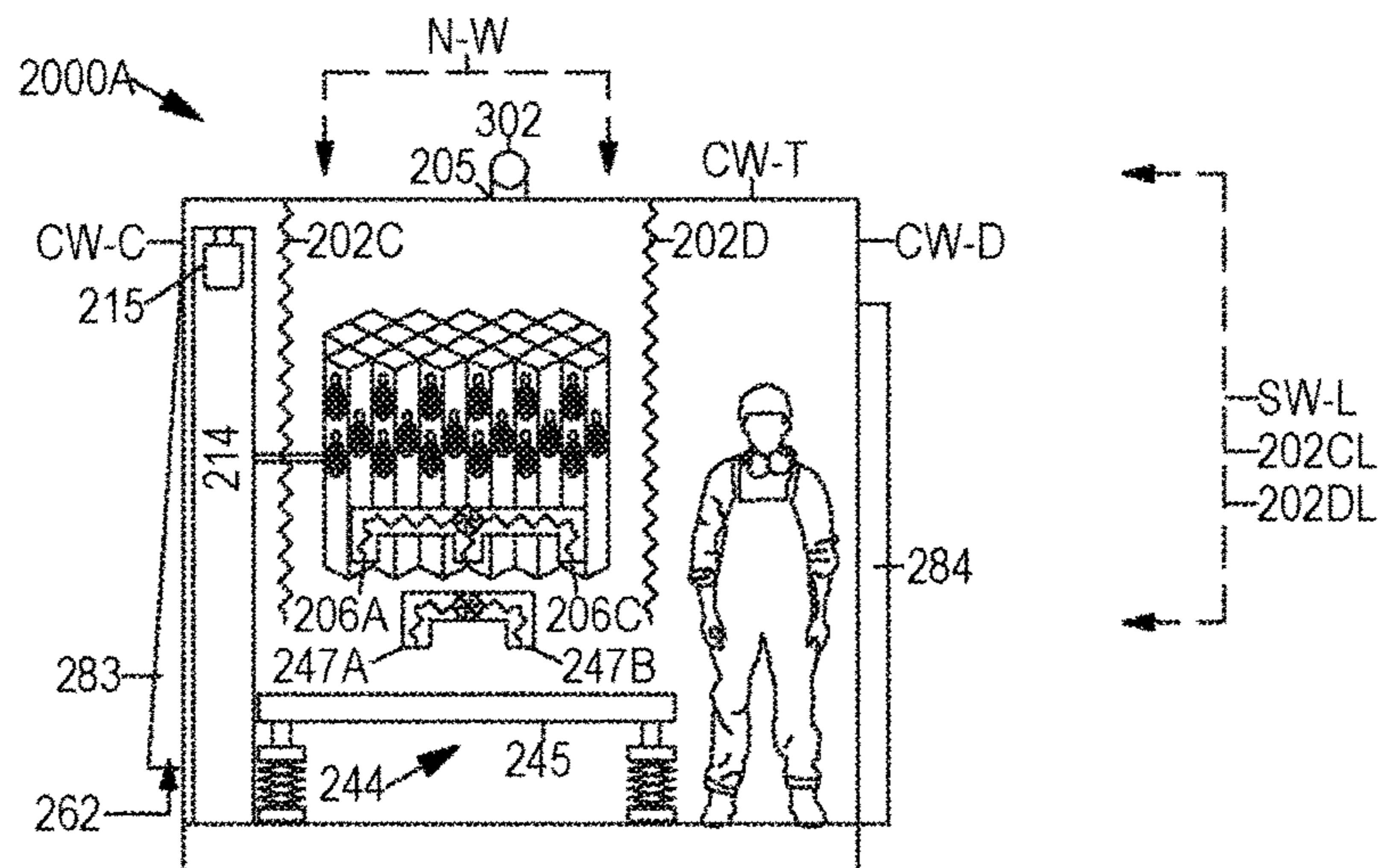
FIGURE 29 INSECT FEEDING MODULE, SIDE VIEW
