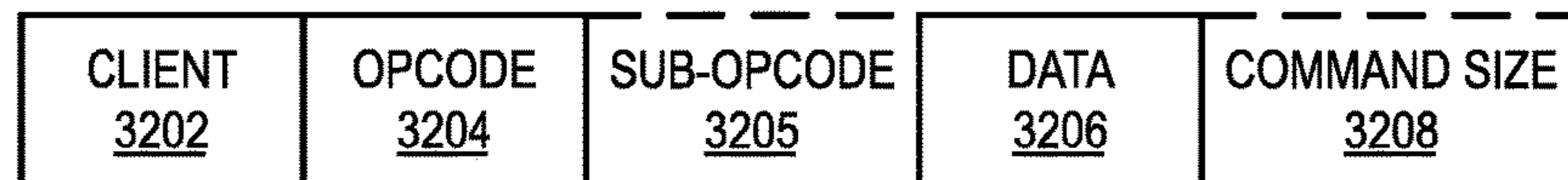
FIG. 32A GRAPHICS PROCESSOR COMMAND FORMAT 3200
