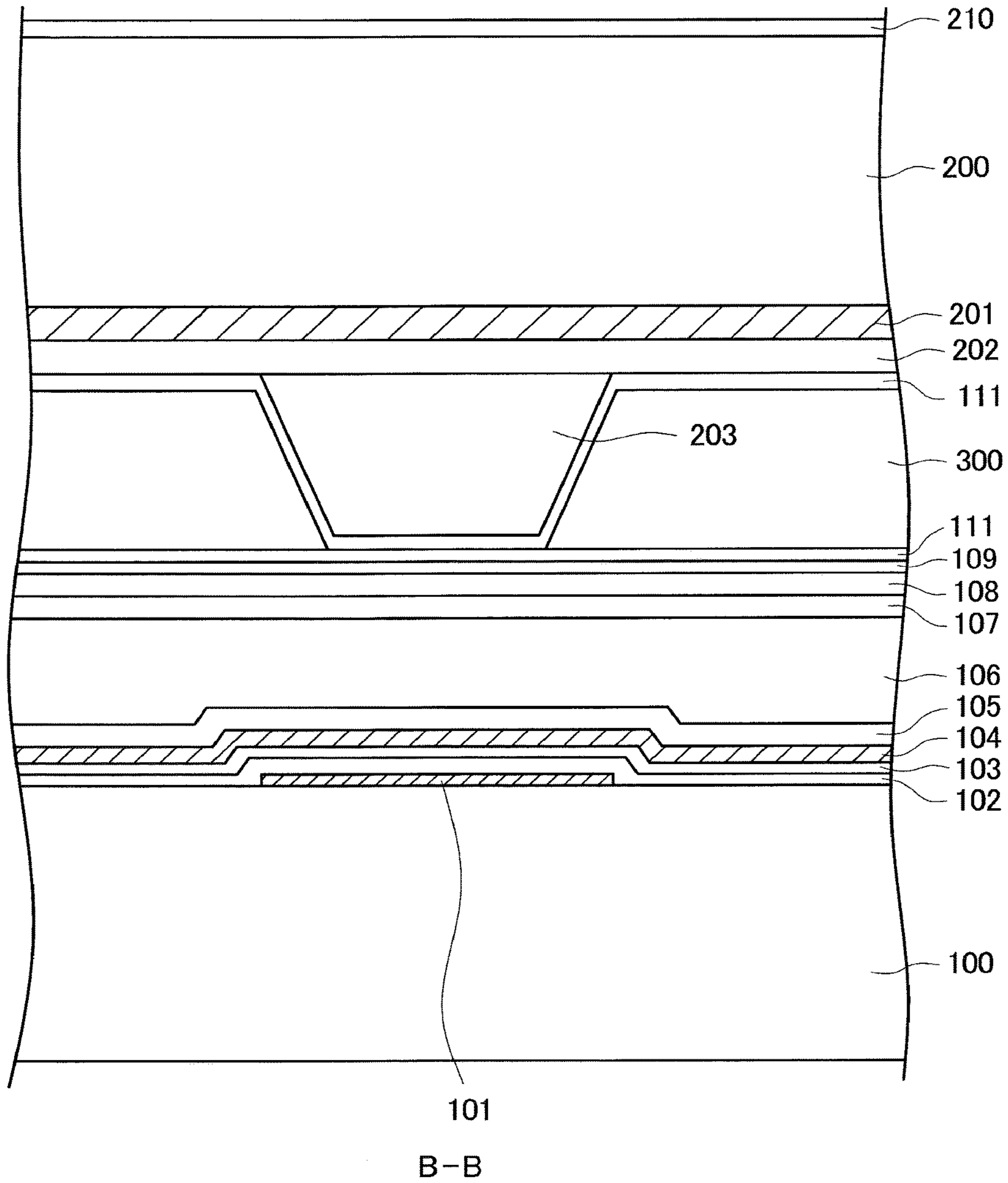
FIG. 7 (Prior Art)
