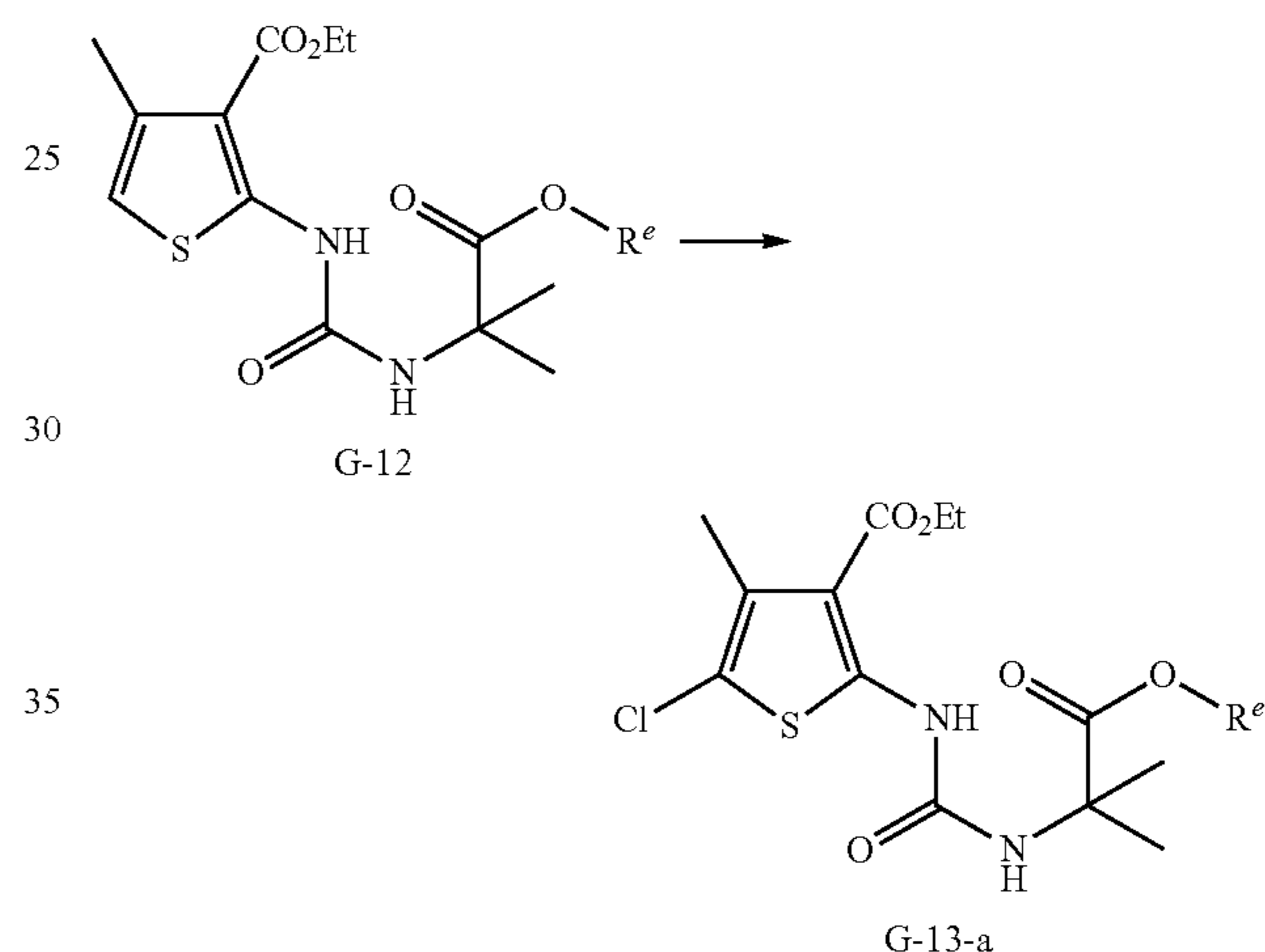
Scheme 6. Synthesis of Intermediate G-13-a
