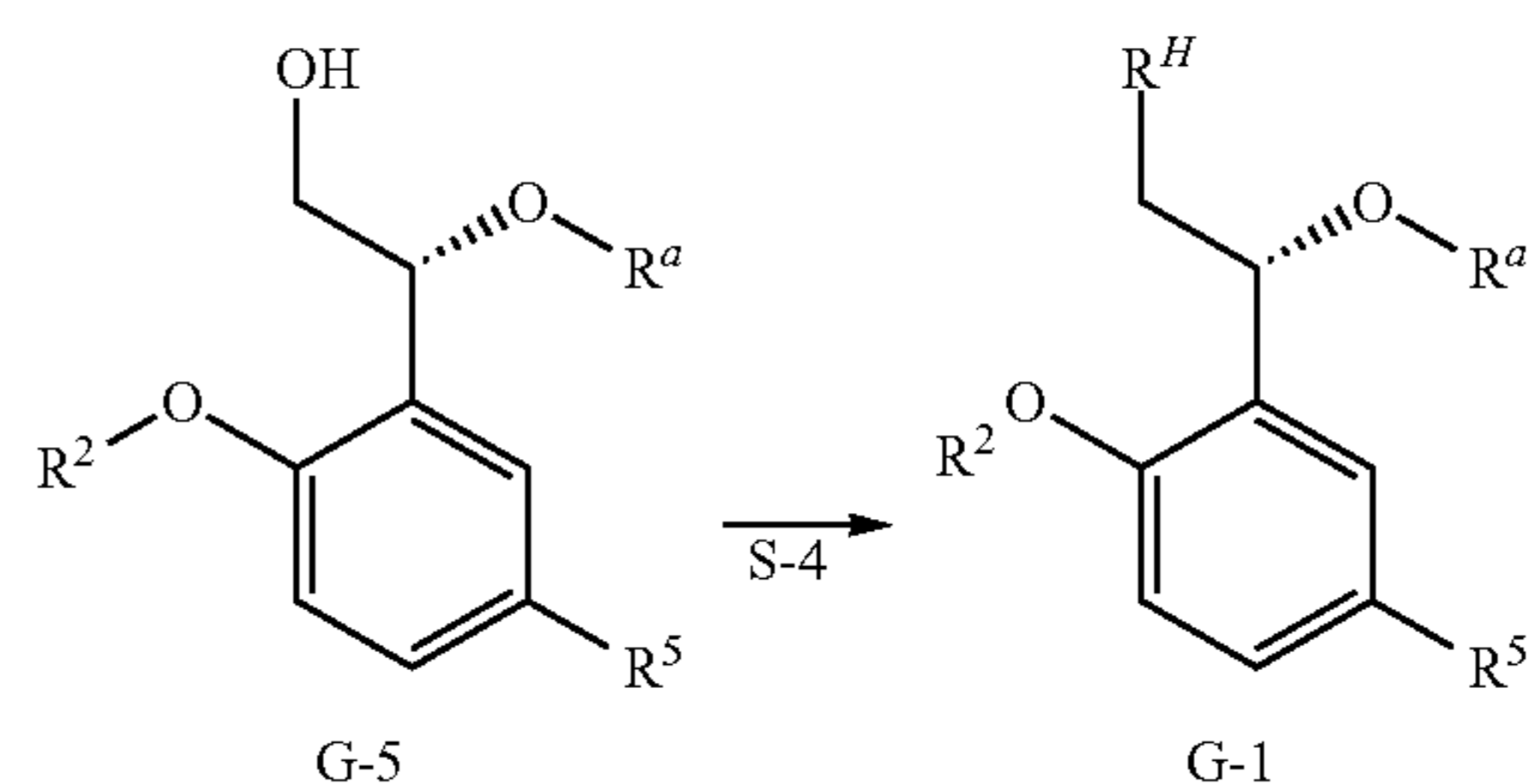
Scheme 2. Synthesis of Intermediates of Formula G-1
