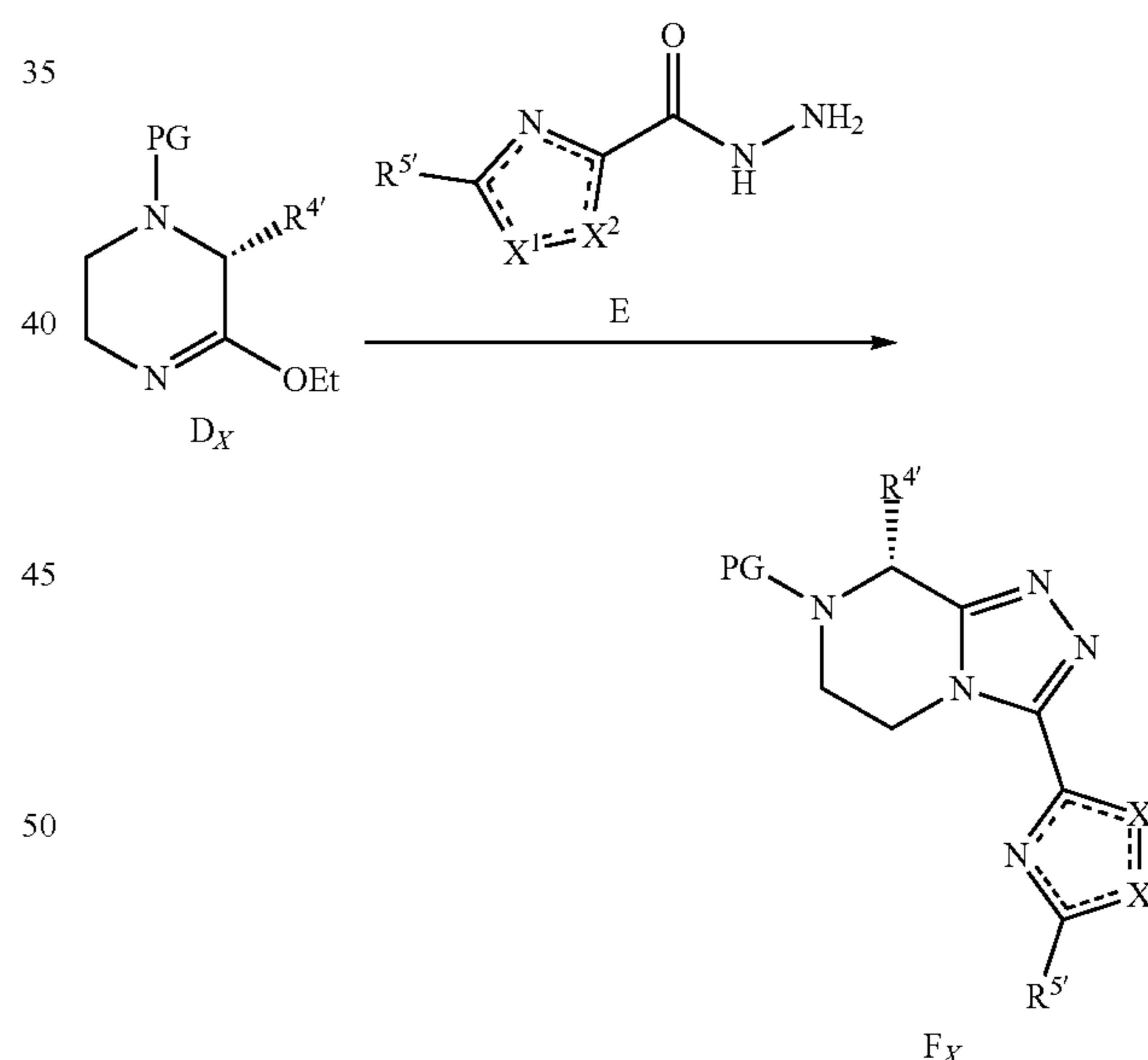
Scheme 13: Formation of acylhydrazide F.
