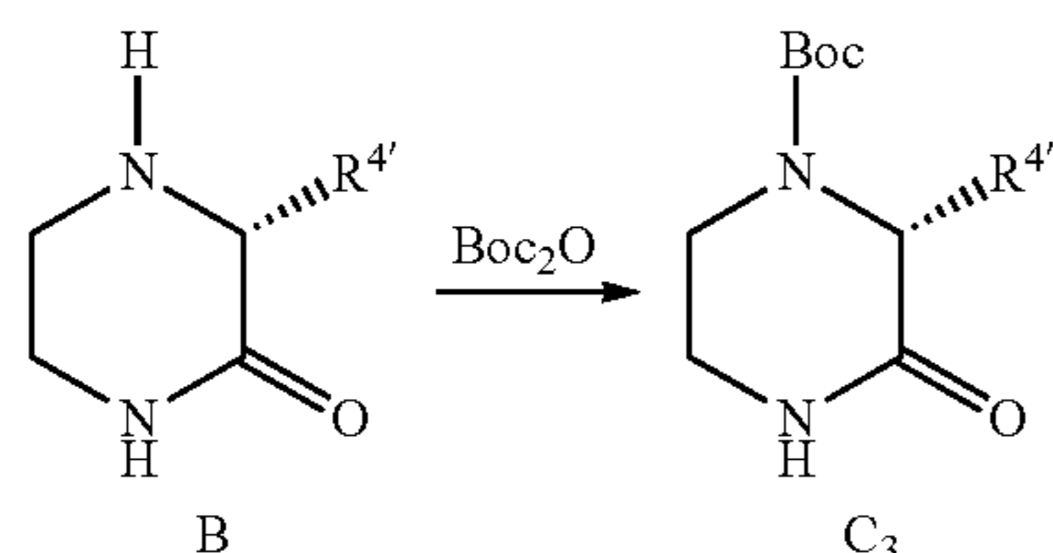
Scheme 10: Boc protection of B.
