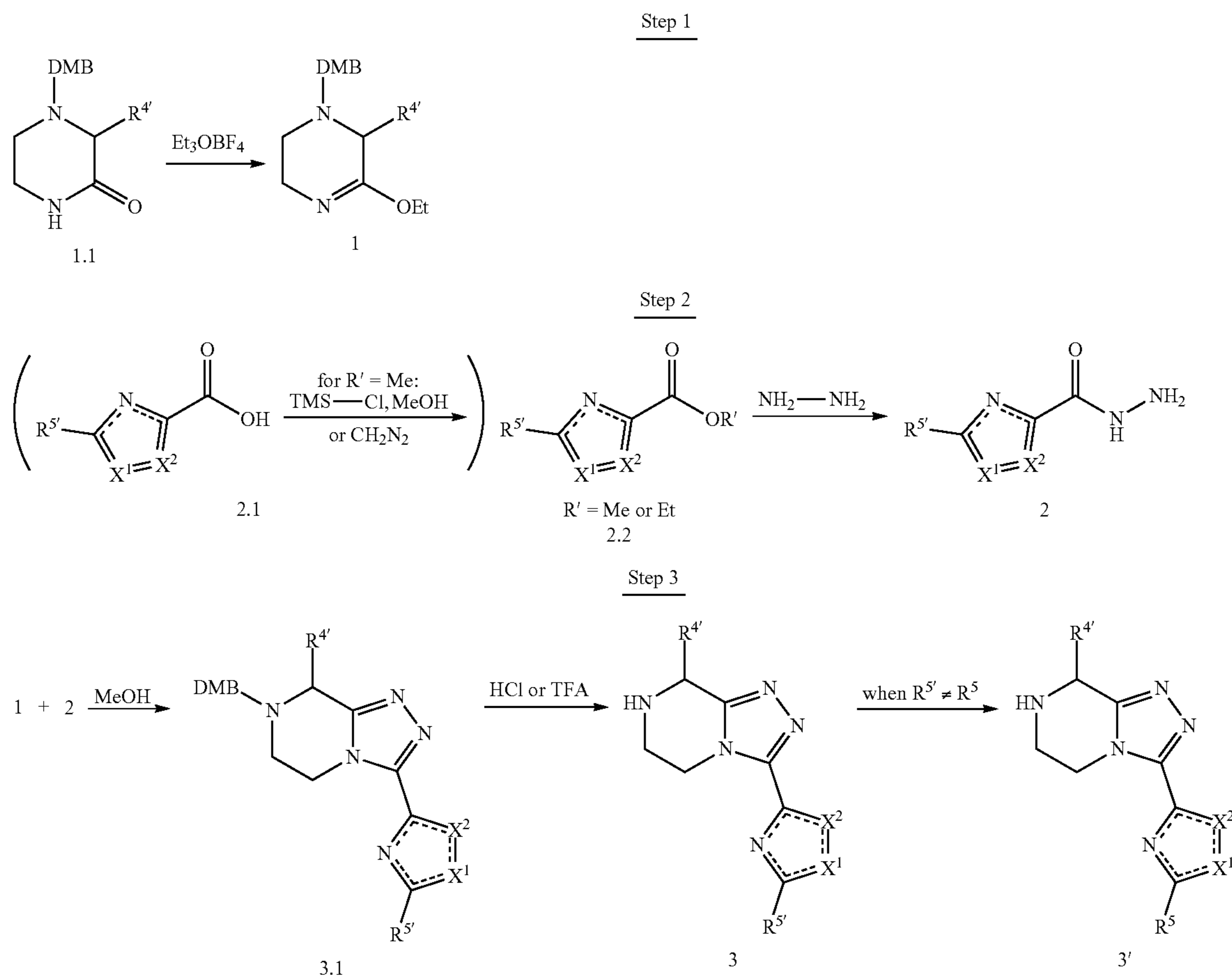
Scheme 1: General racemic synthetic scheme for the preparation of the compounds of the invention.
