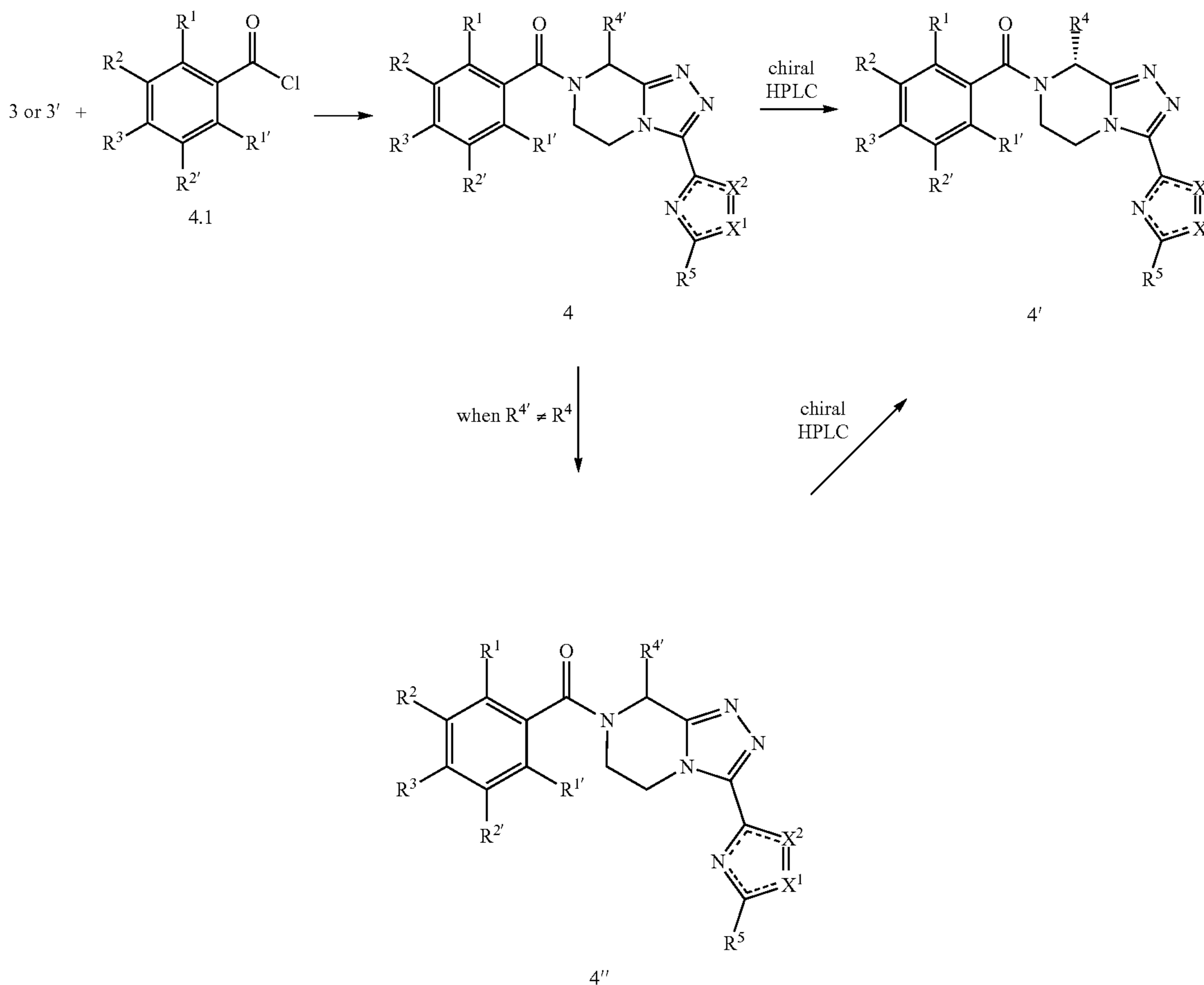
Scheme 6: Acylation and chiral HPLC purification.
