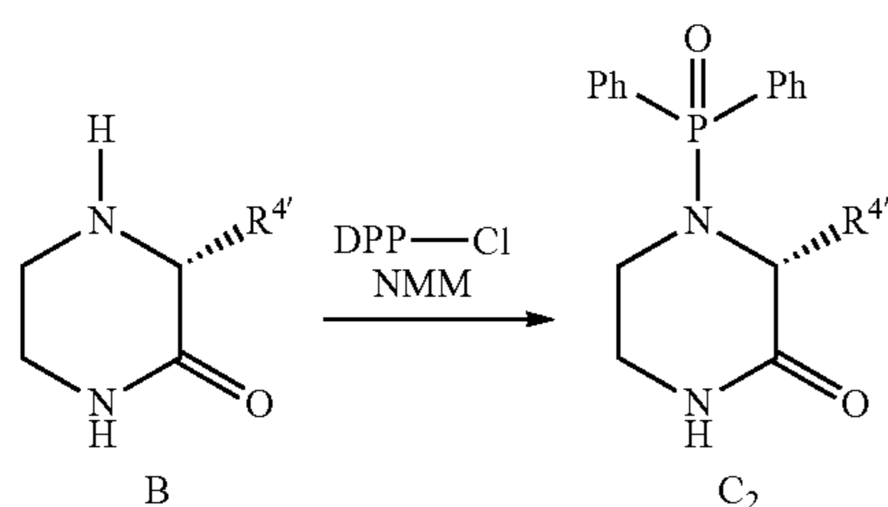
Scheme 9: DPP protection of B.
