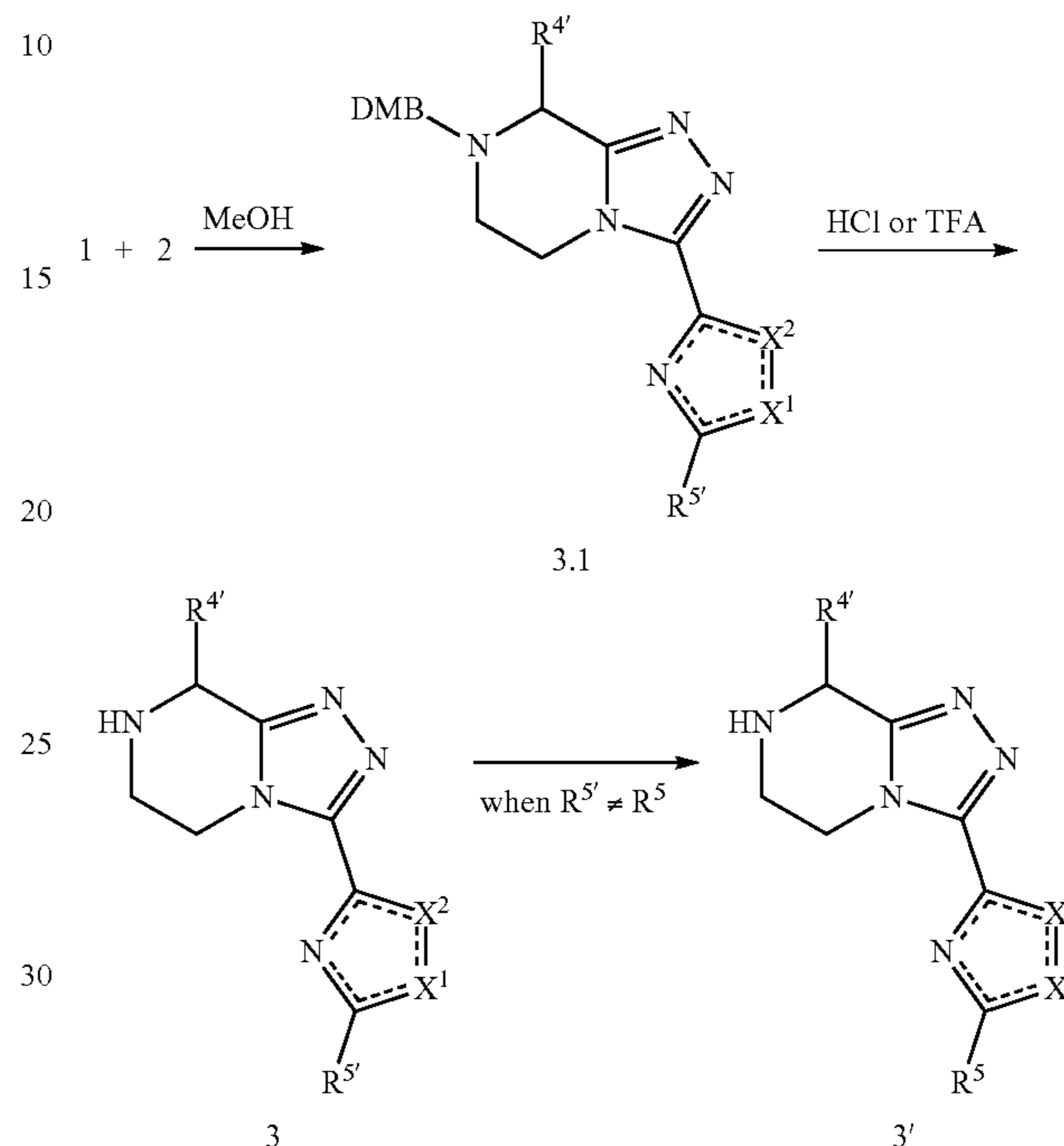
Scheme 5: Cyclodehydration leading to triazolopiperazine 3.
