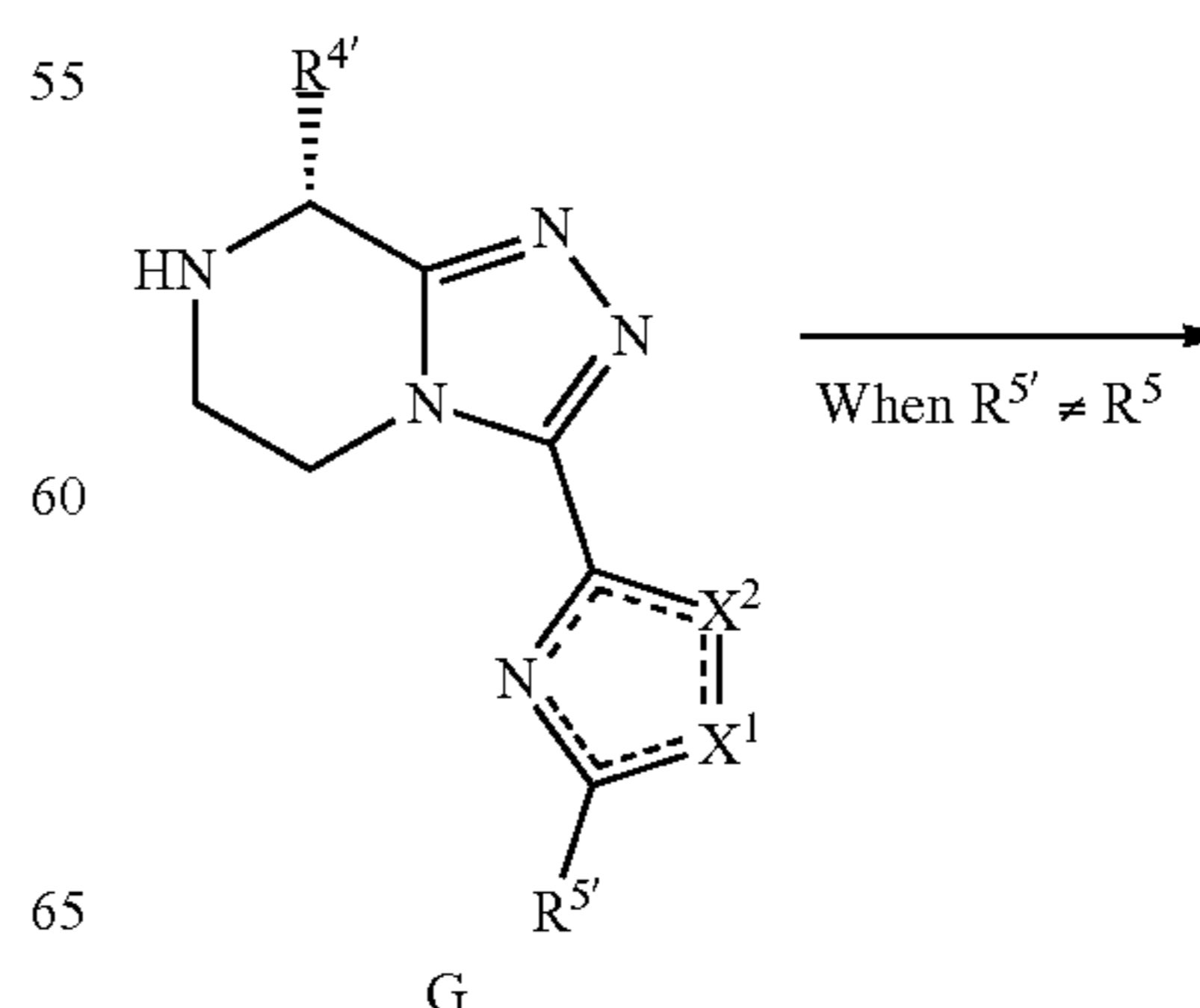
Scheme 15: conversion of R 5' to R 5 in triazolopyrazine G leading to G'.
