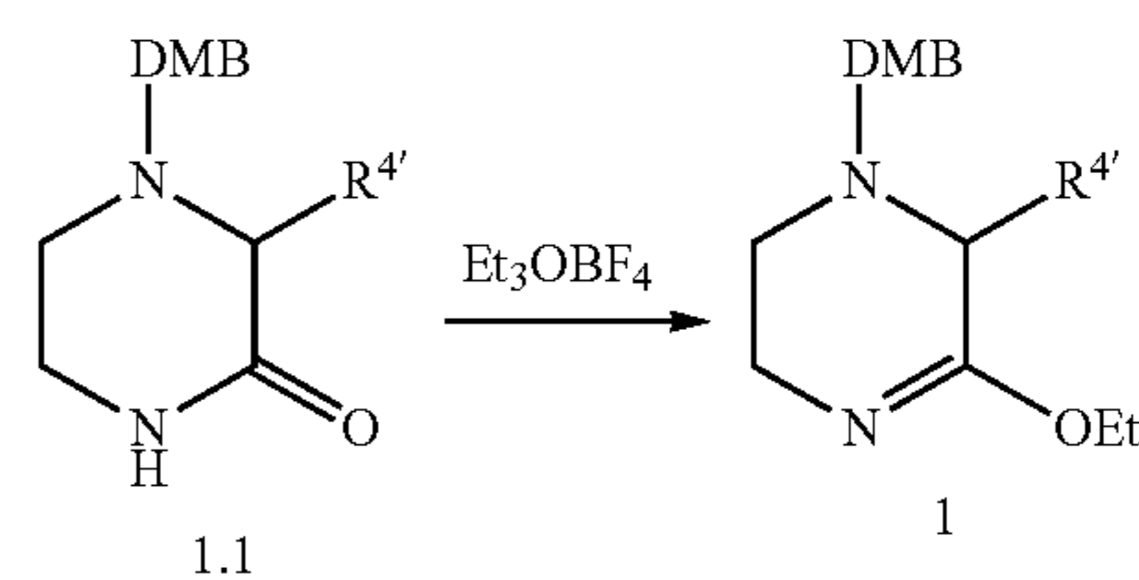
Scheme 2: Conversion to iminoether 1.
