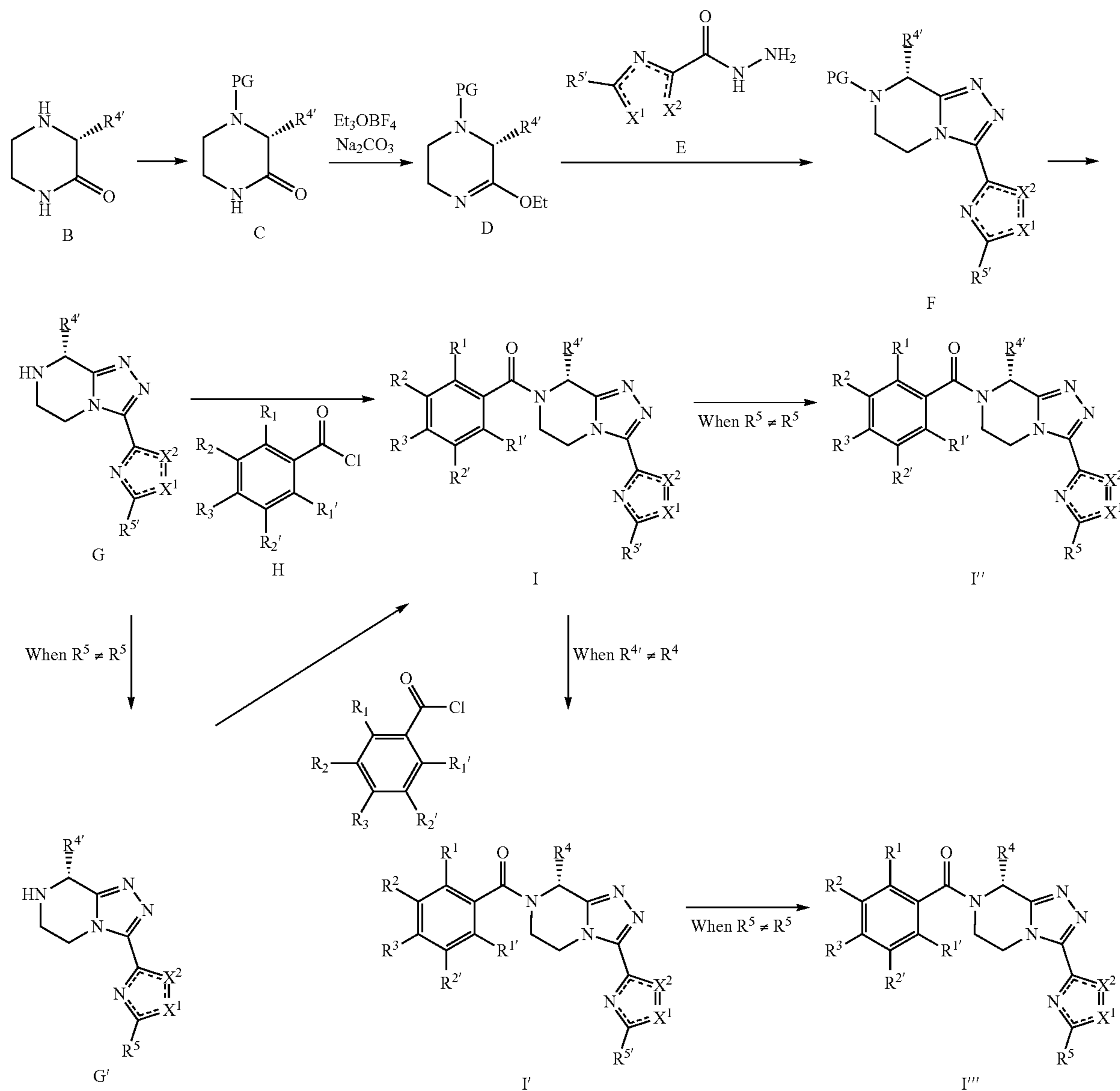
Scheme 7: General synthetic scheme for the preparation of chiral compounds of the invention.
