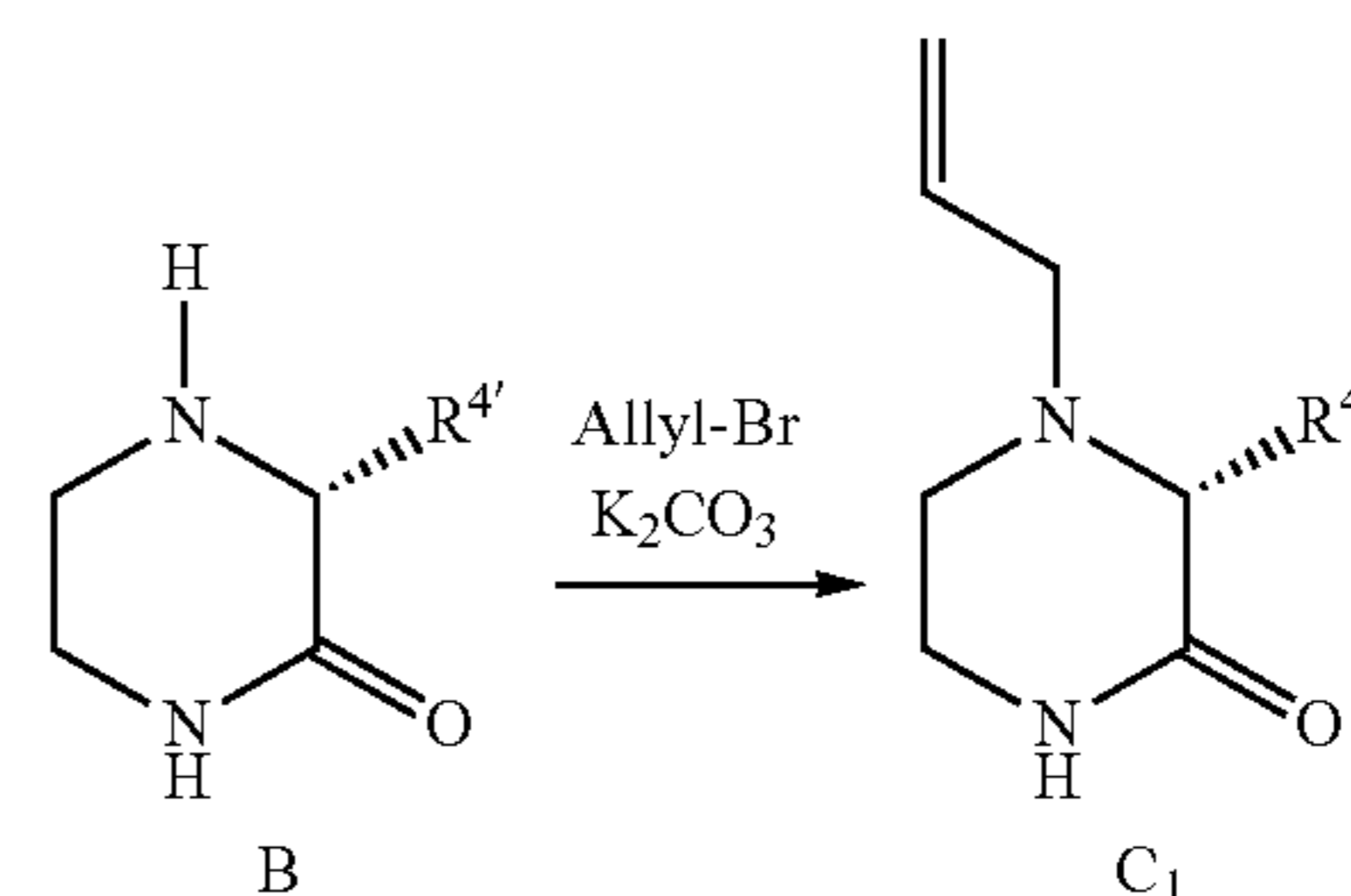
Scheme 8: Allyl protection of B.
