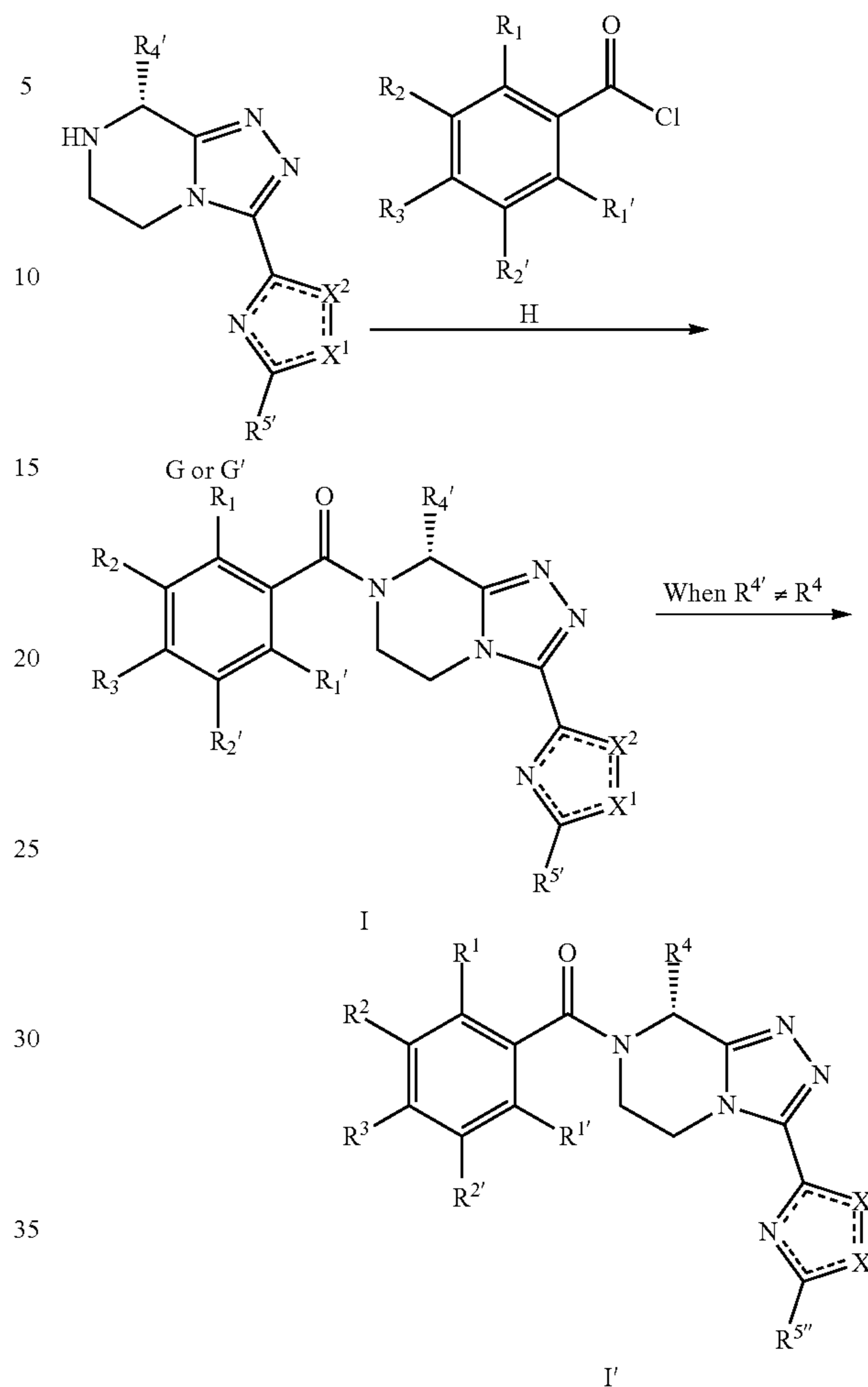
Scheme 16: Acylation.
