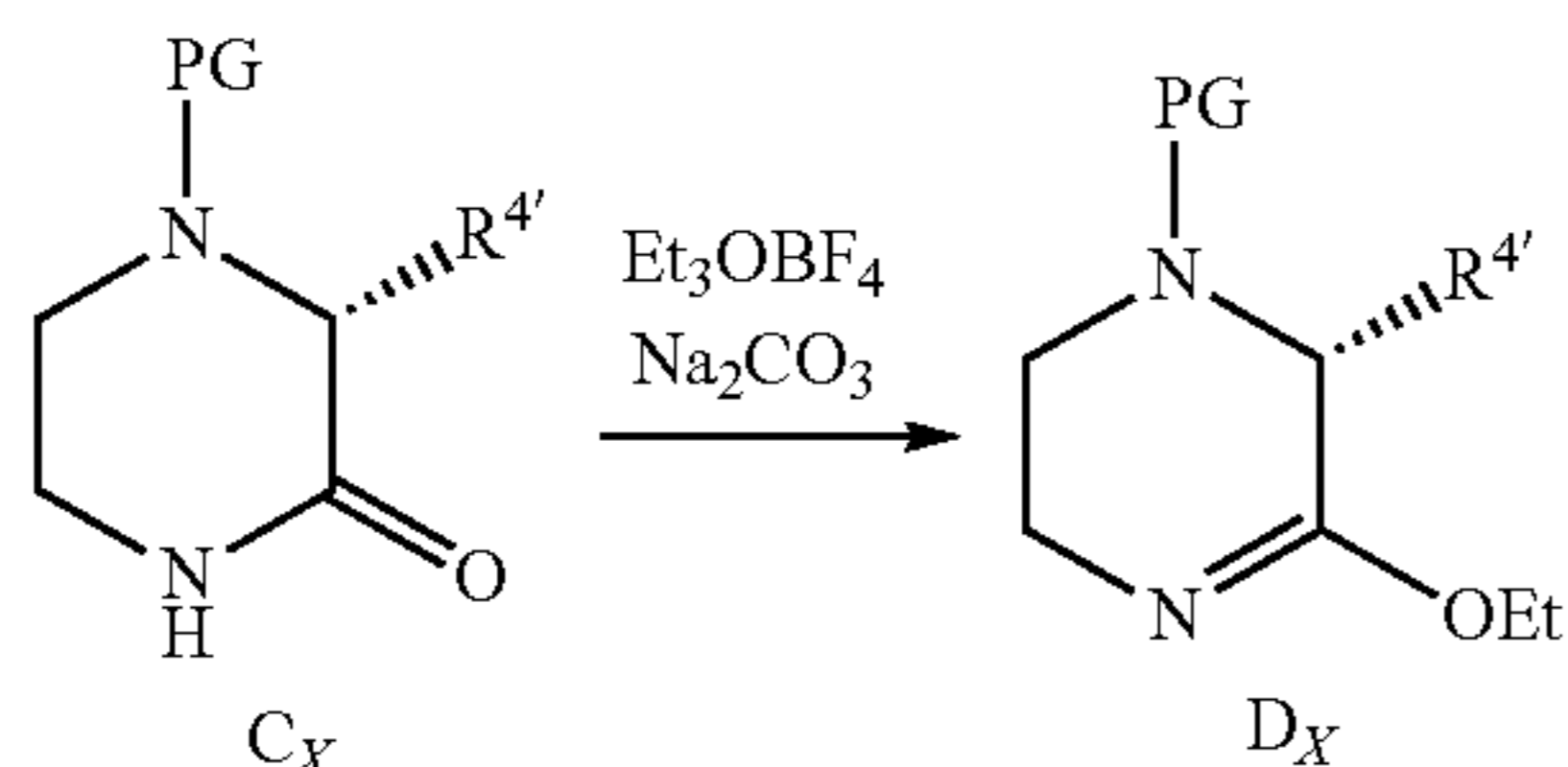
Scheme 12: Conversion to iminoether D.
