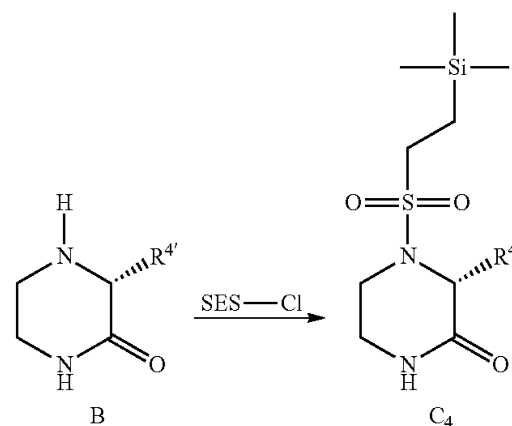
Scheme 11: SES protection of B.
