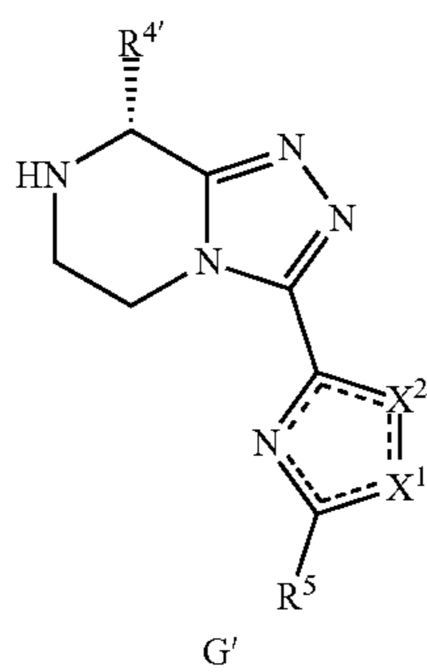
Scheme 16: Acylation.
