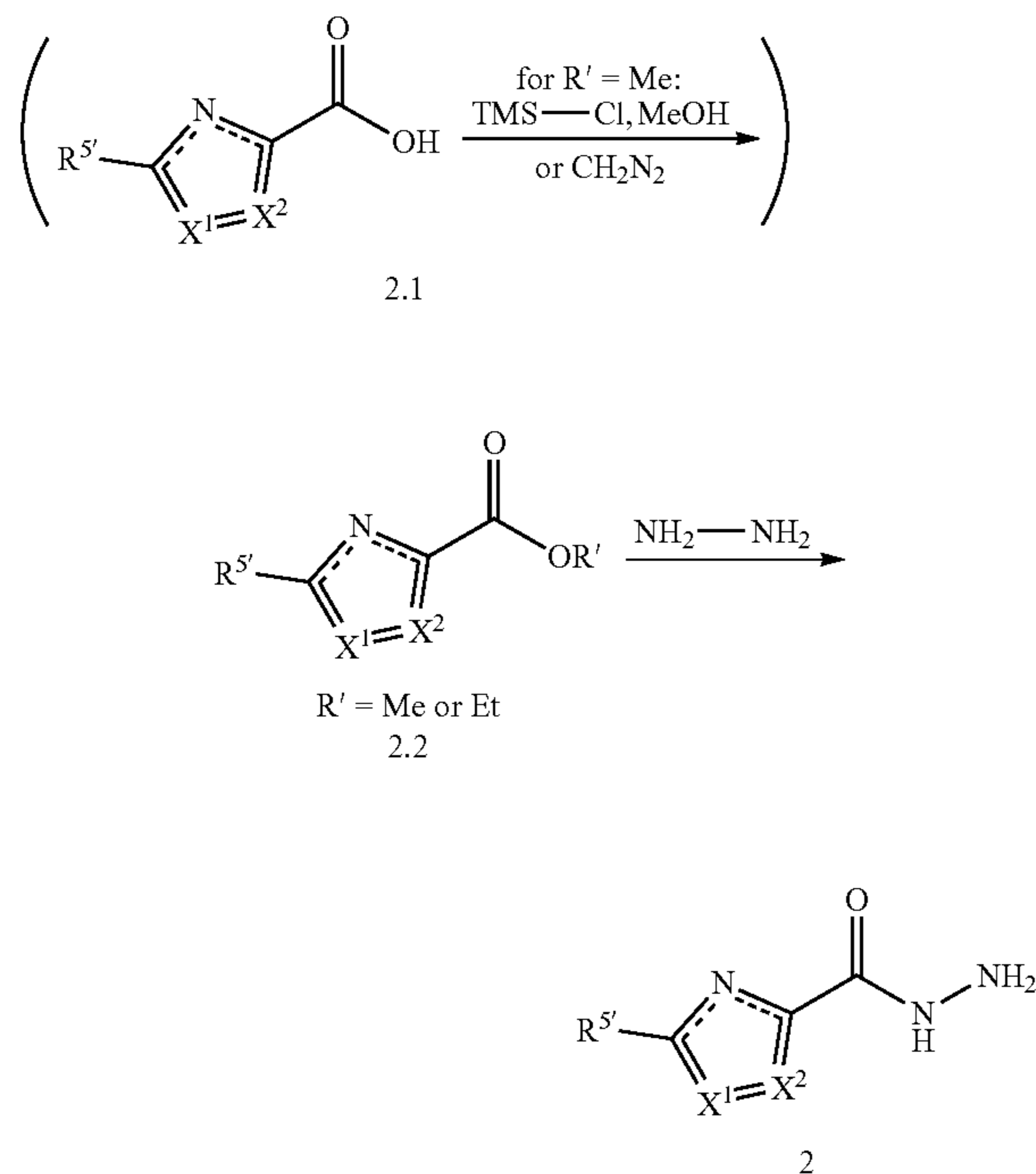
Scheme 4: Formation of acylhydrazide 2.
