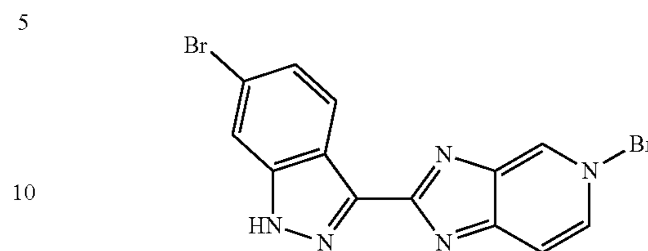
(a) 5-Benzyl-2-(6-bromo-1H-indazol-3-yl)-5H-imidazo[4,5-c]pyridine
