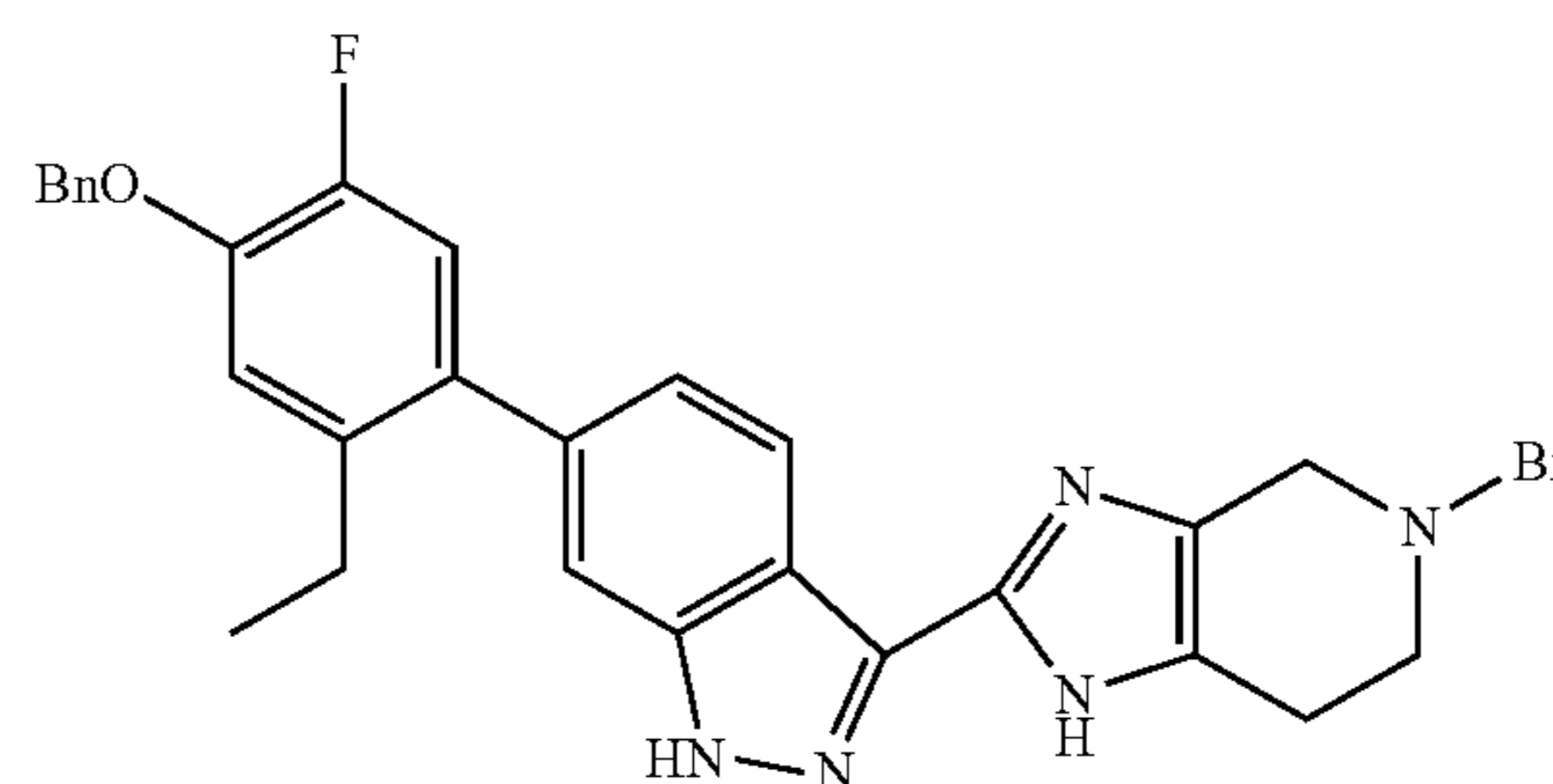
(a) 5-Benzyl-2-(6-(4-(benzyloxy)-2-ethyl-5-fluorophenyl)-1H-indazol-3-yl)-4,5,6,7-tetrahydro-1H-imidazo[4,5-c]pyridine
