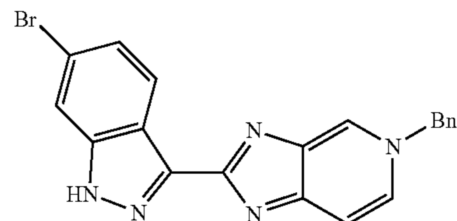
(a) 6-Bromo-1H-indazol-3-yl-carbaldehyde
