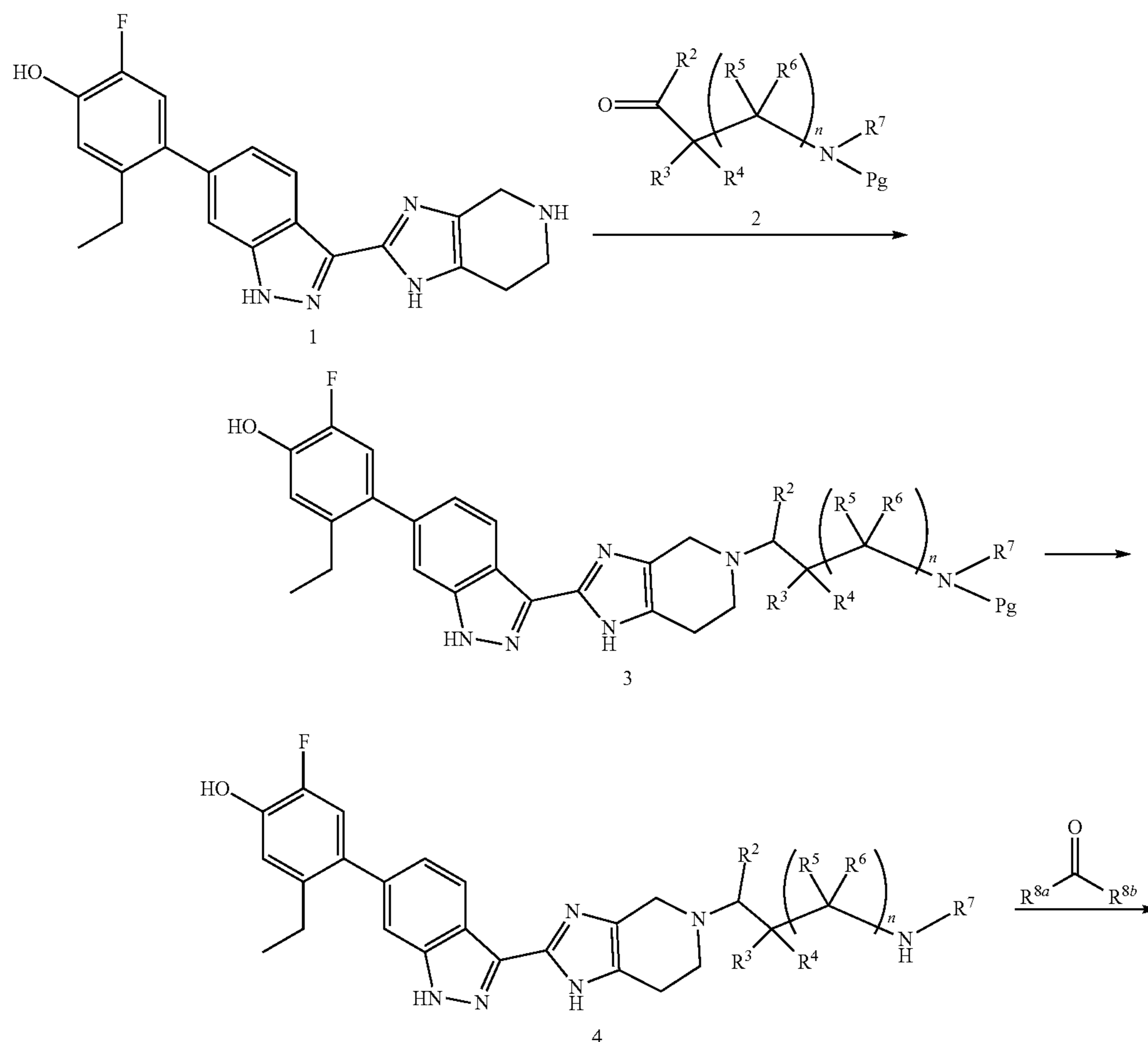
Scheme 1
