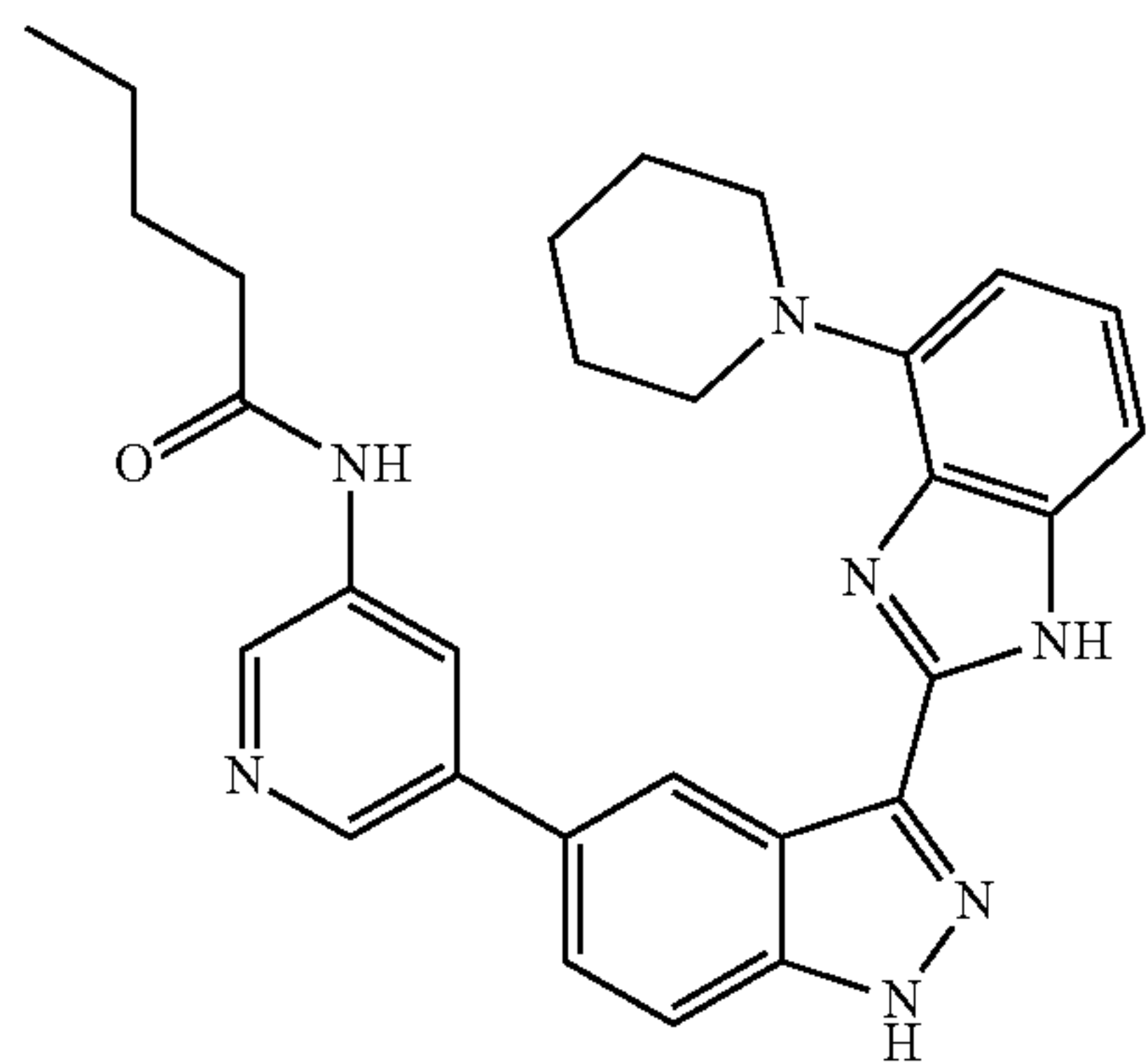
N-(5-(3-(4-(Piperidin-1-yl)-1H-benzo[d]imidazol-2-yl)-1H-indazol-5-yl)pyridin-3-yl)pentanamide 162
