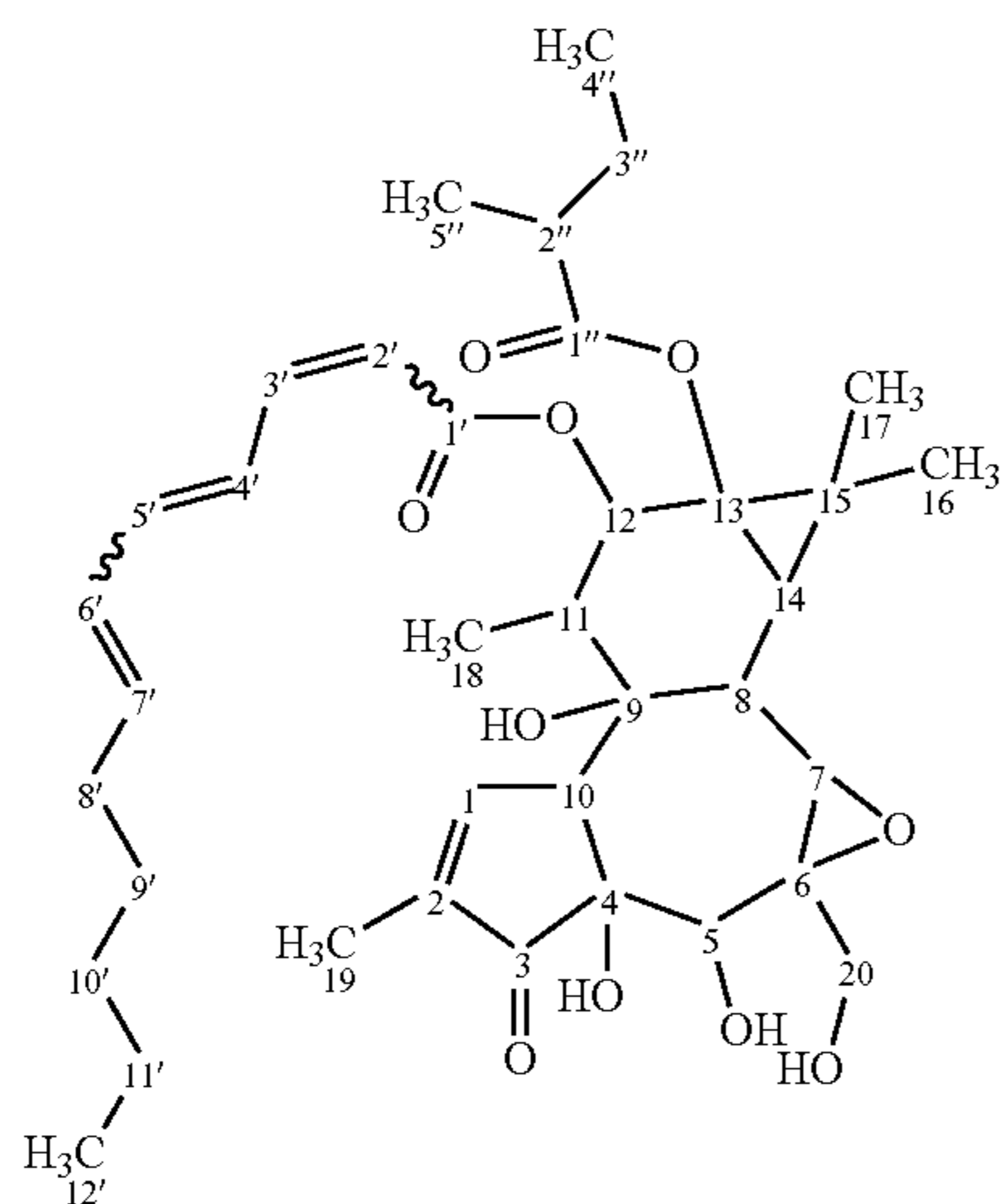
Compound 3: 12-[(2E,4E,6E)-dodeca-2,4,6-trienoyl]-13-(2-methylbutanoyl)-6,7-epoxy-4,5,9,12,13,20-hexahydroxy-1-tigliaen-3-one
