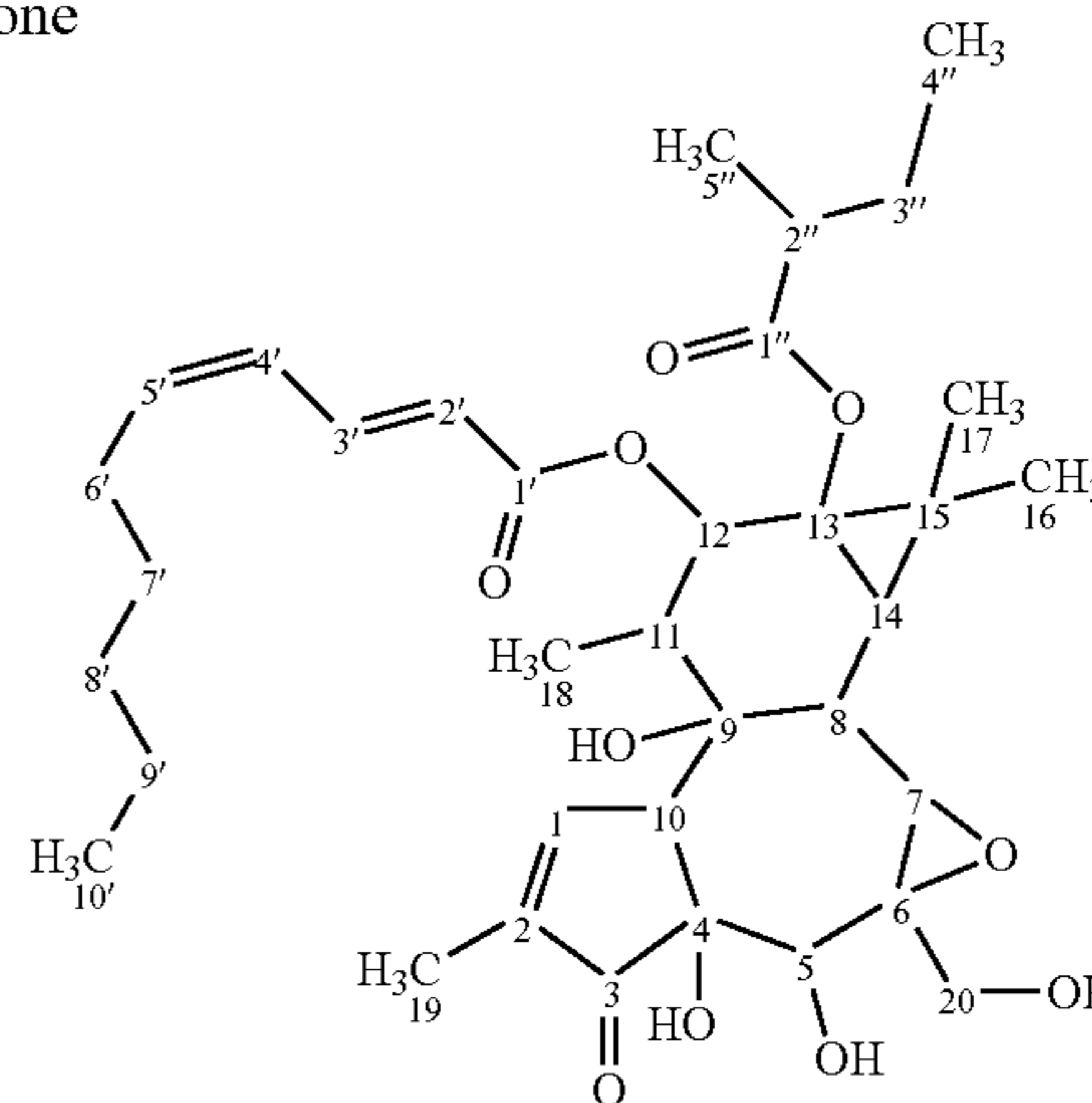
Compound 4: 12-[(2E,4Z)-deca-2,4-dienoyl]-13-(2-methylbutanoyl)-6,7-epoxy-4,5,9,12,13,20-hexahydroxy-1-tigliaen-3-one
