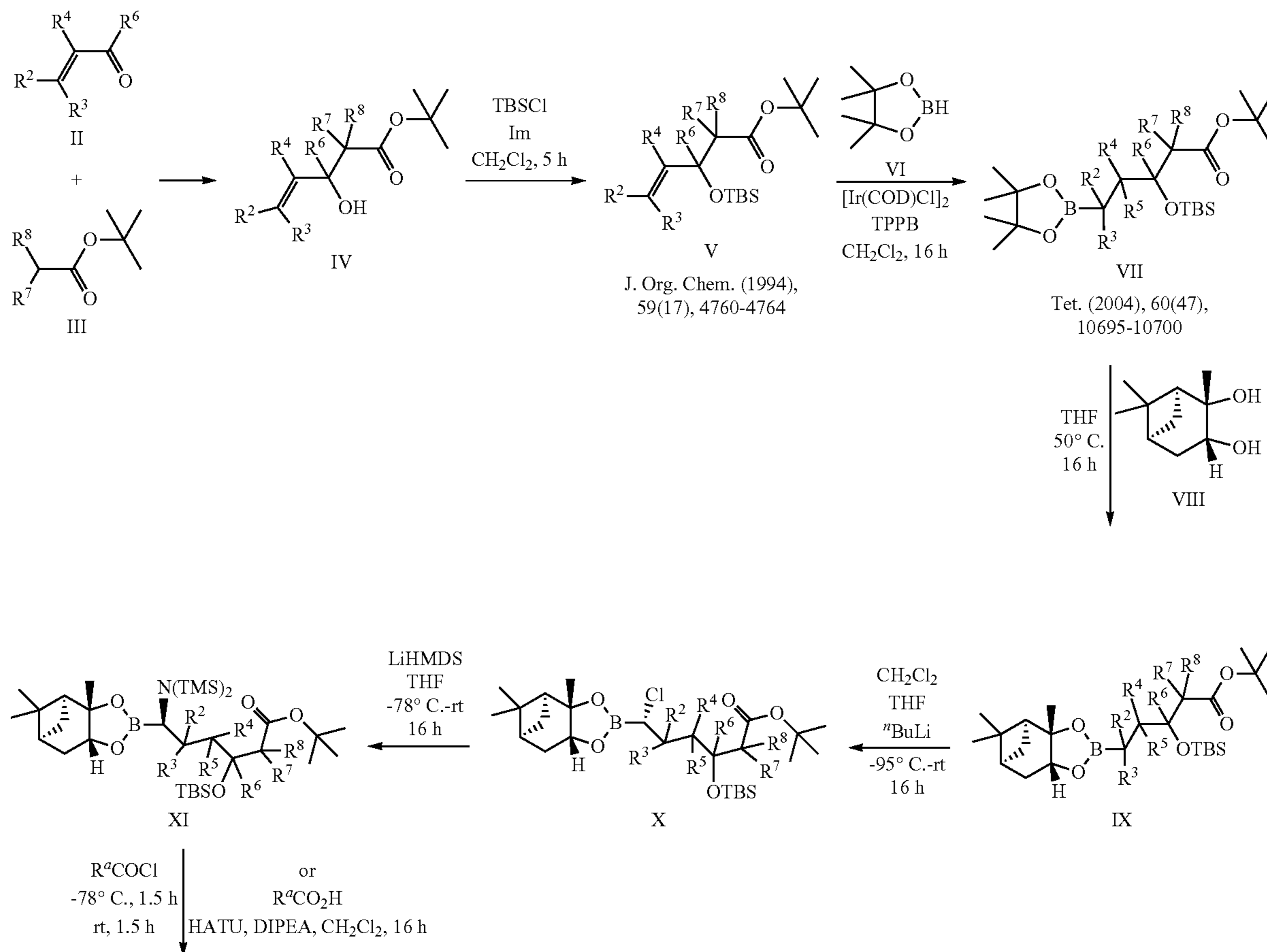
Scheme 1
