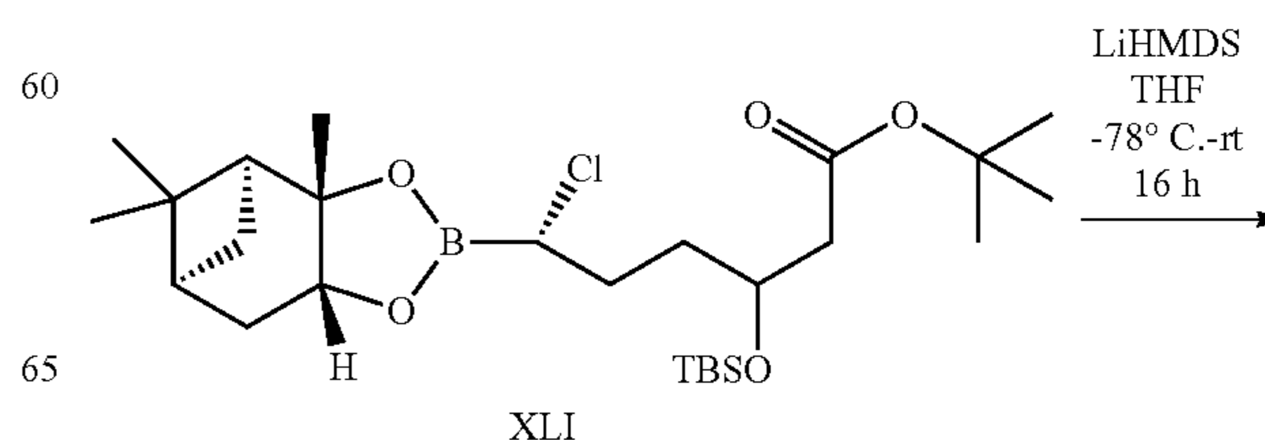
Scheme 10
