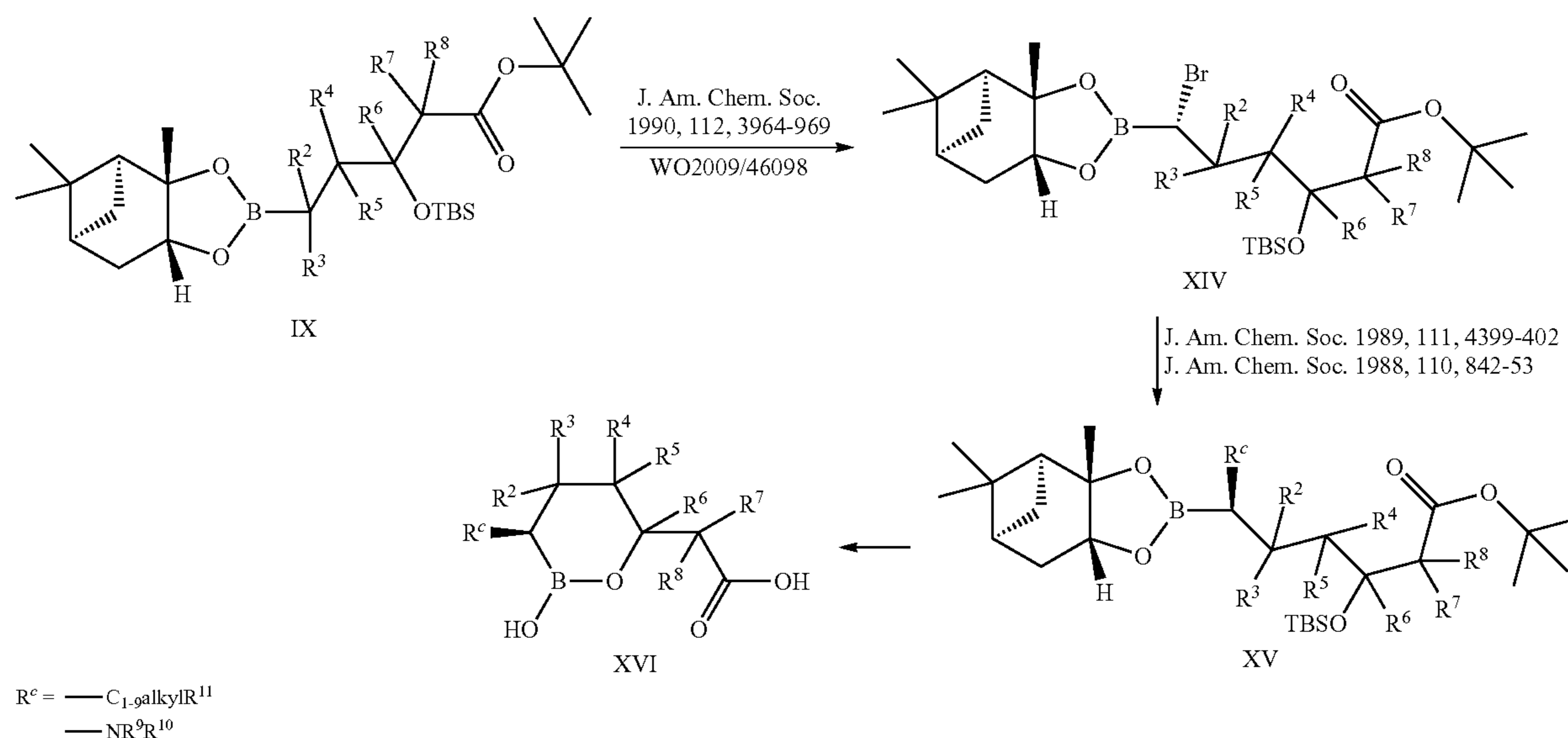
Scheme 2
