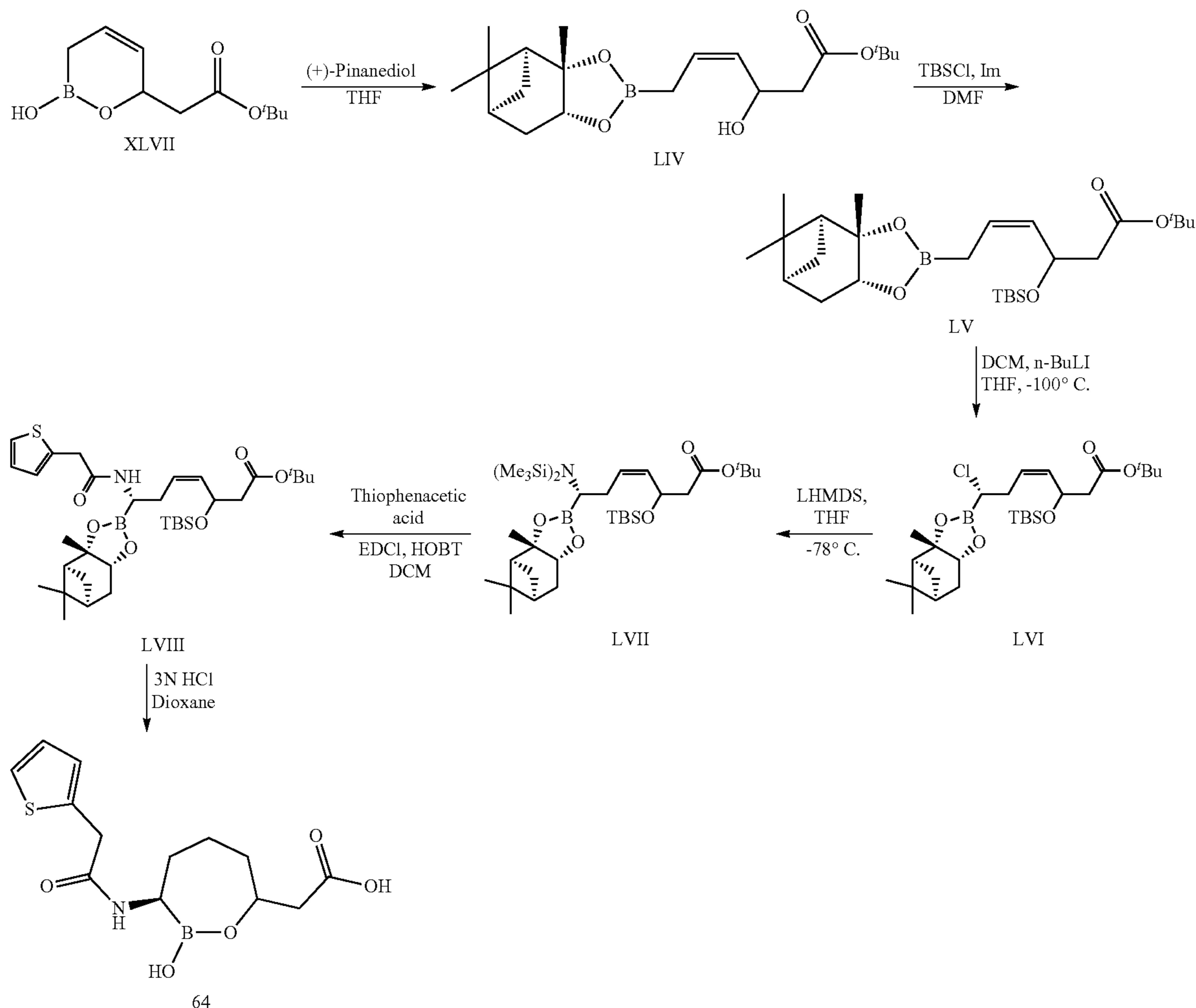
Scheme 12
