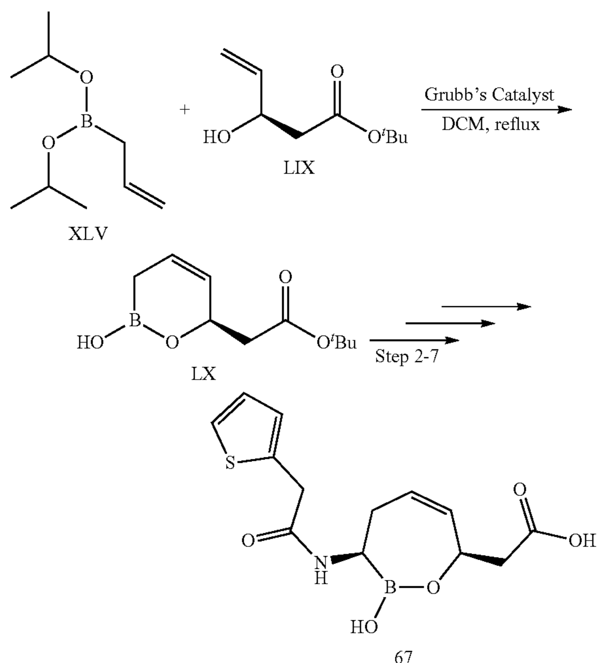
Scheme 14
