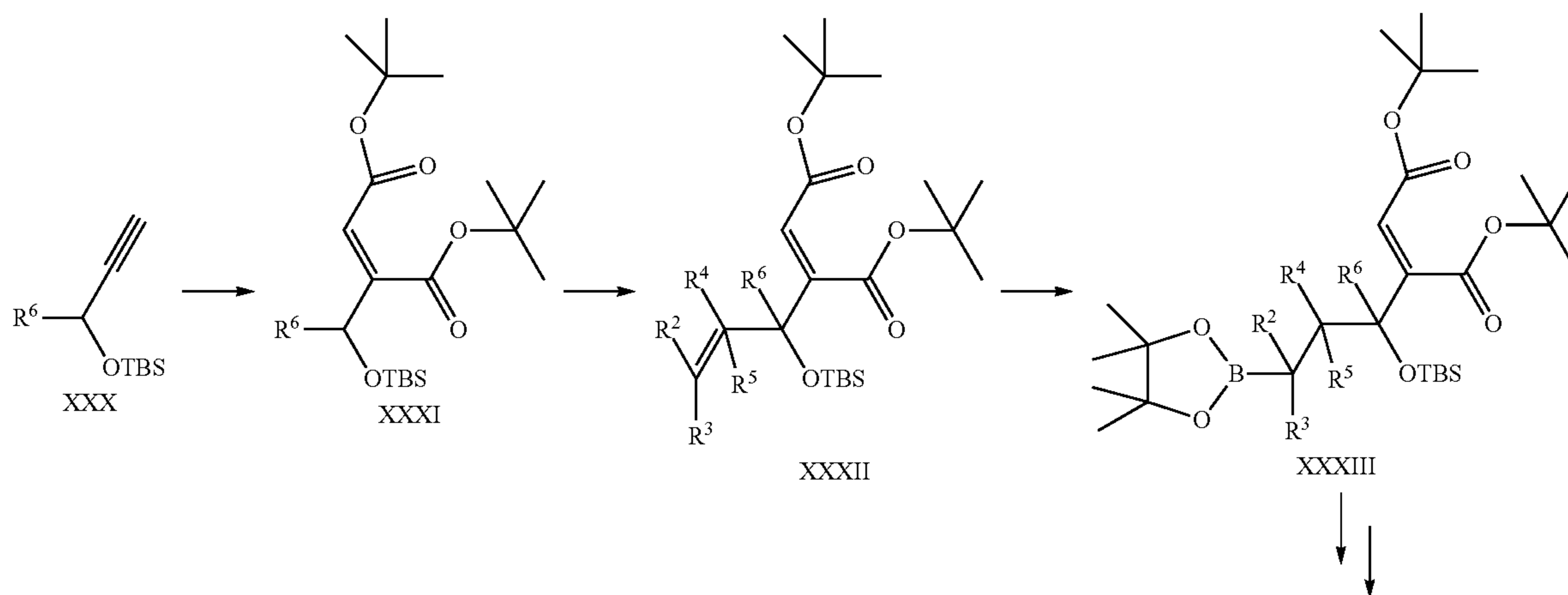
Scheme 7
