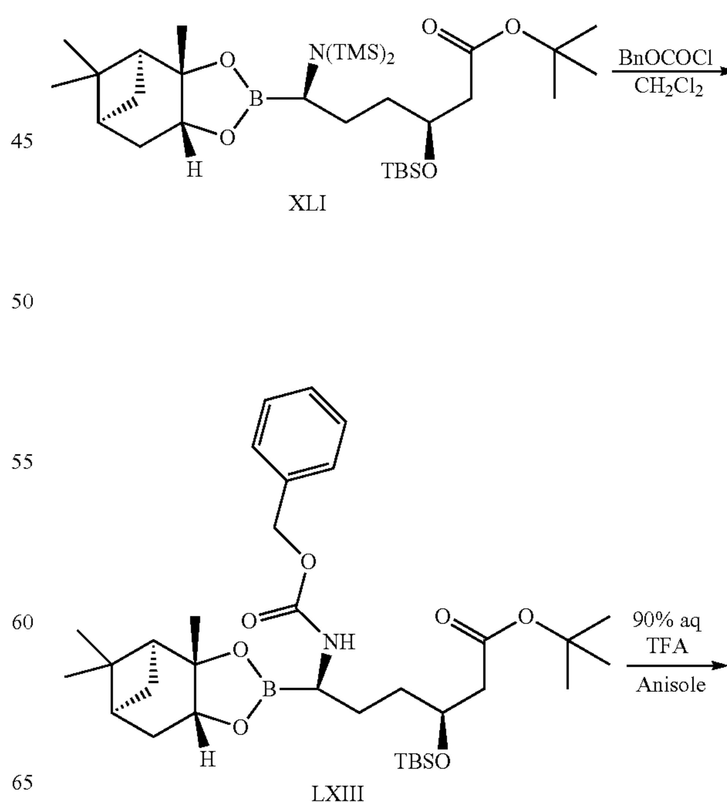
Scheme 16
