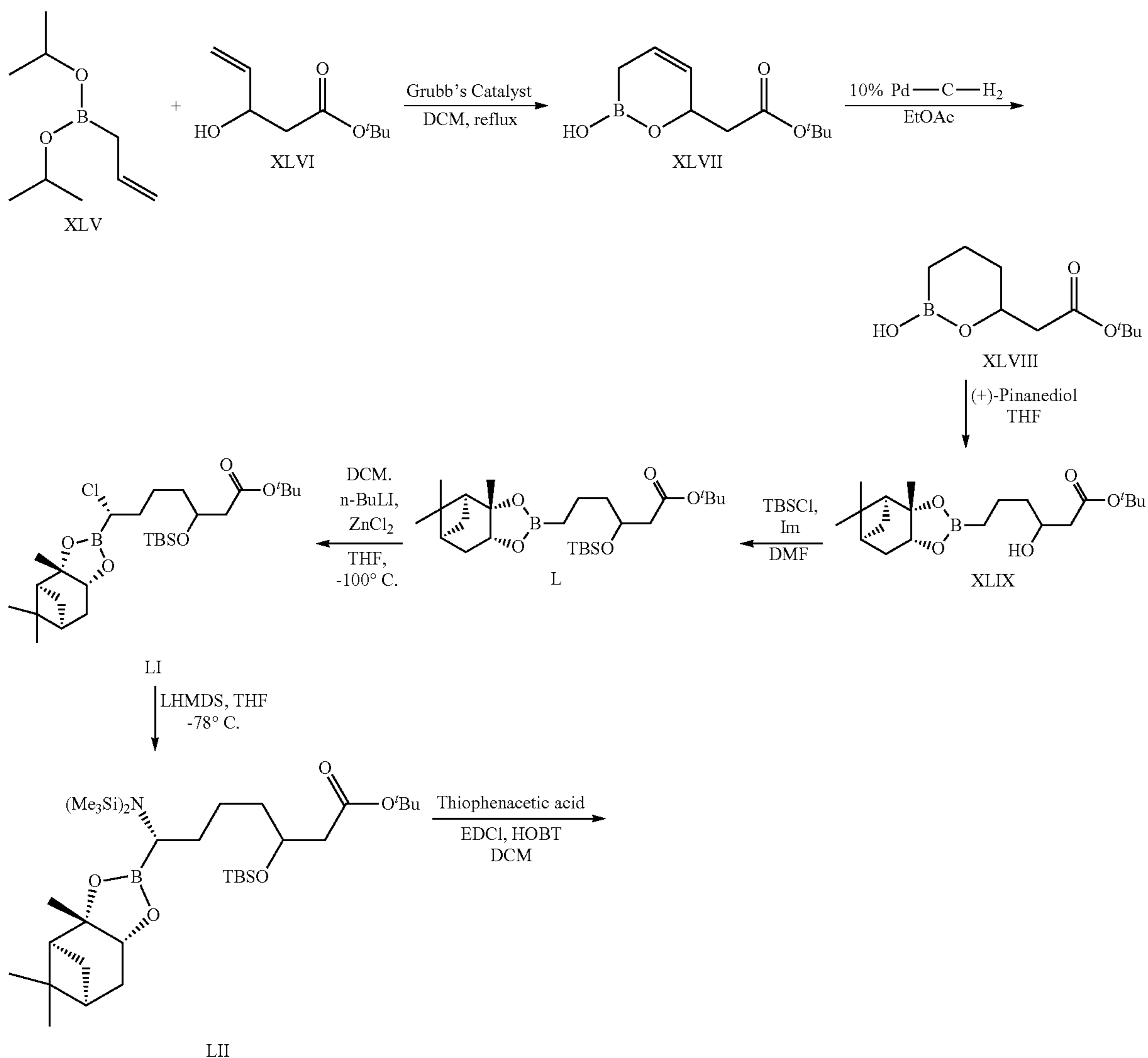
Scheme 11
