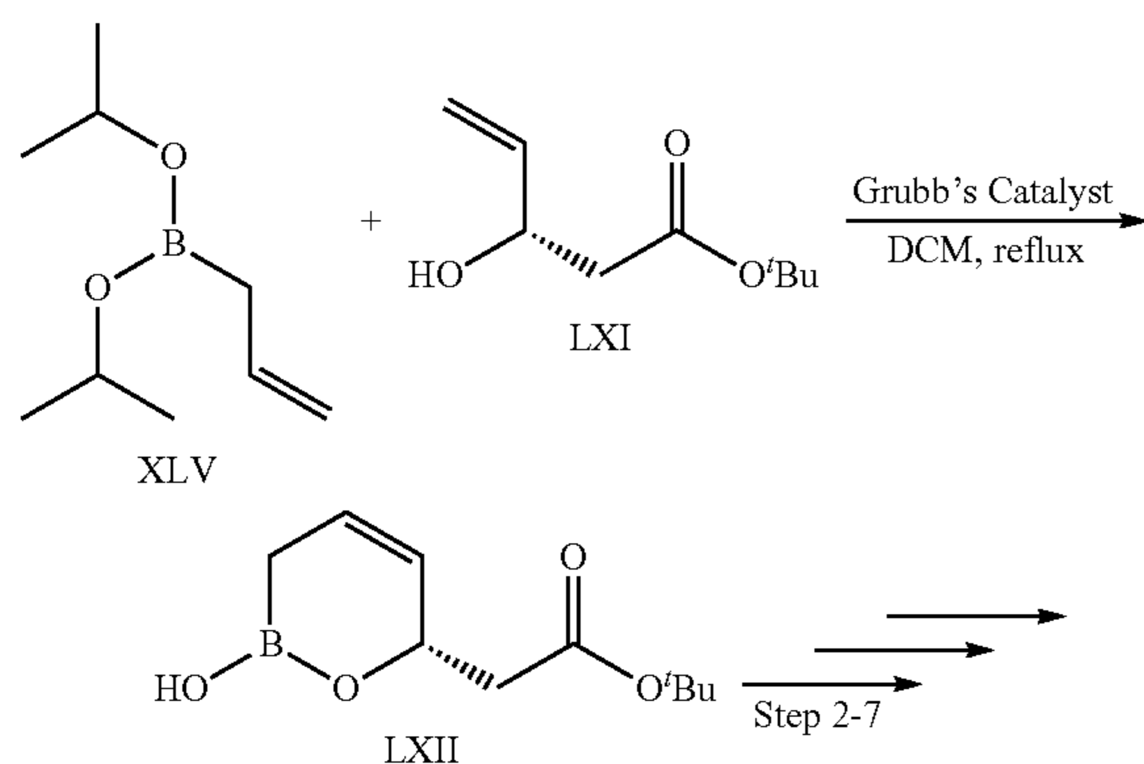
Scheme 15
