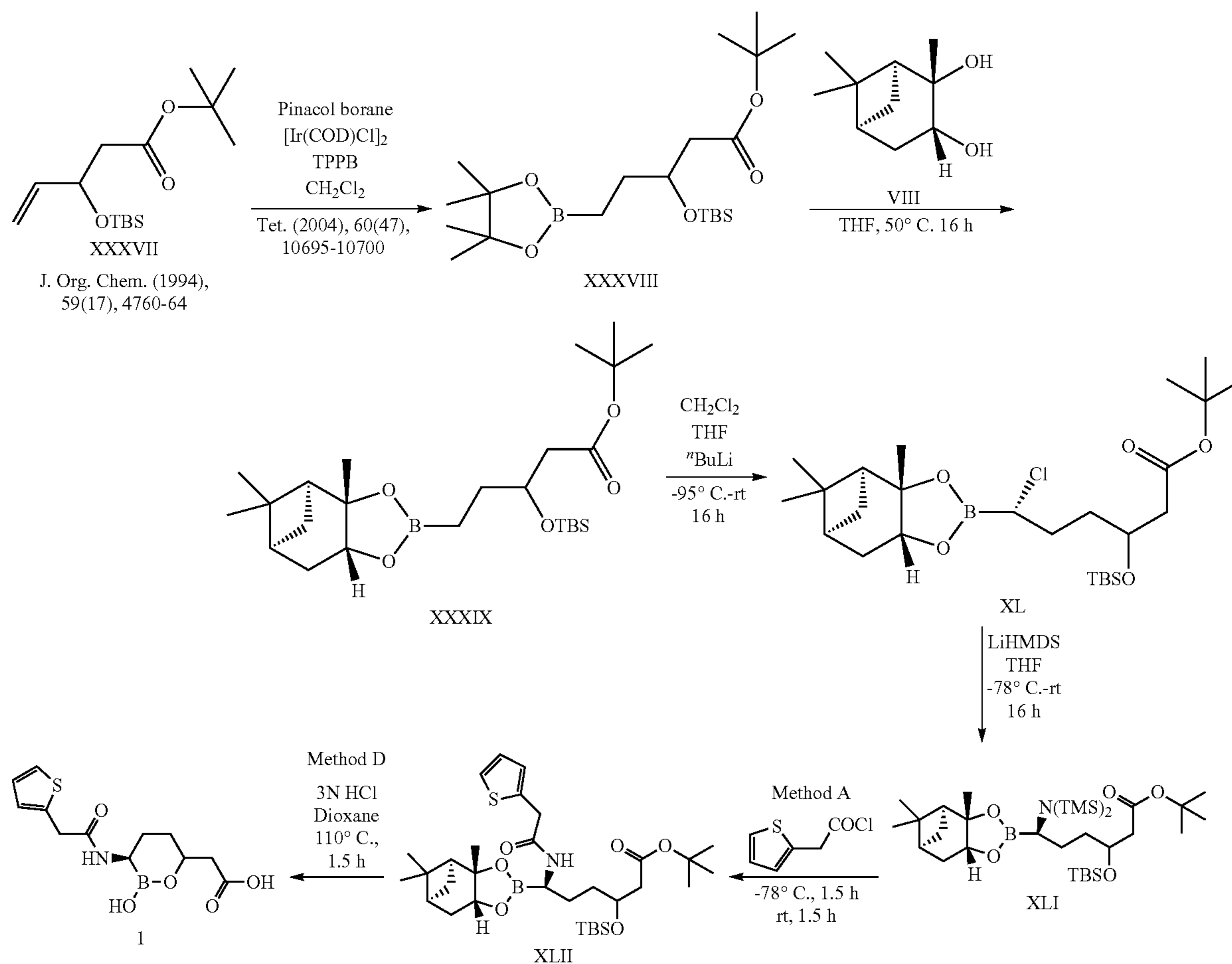
Scheme 8
