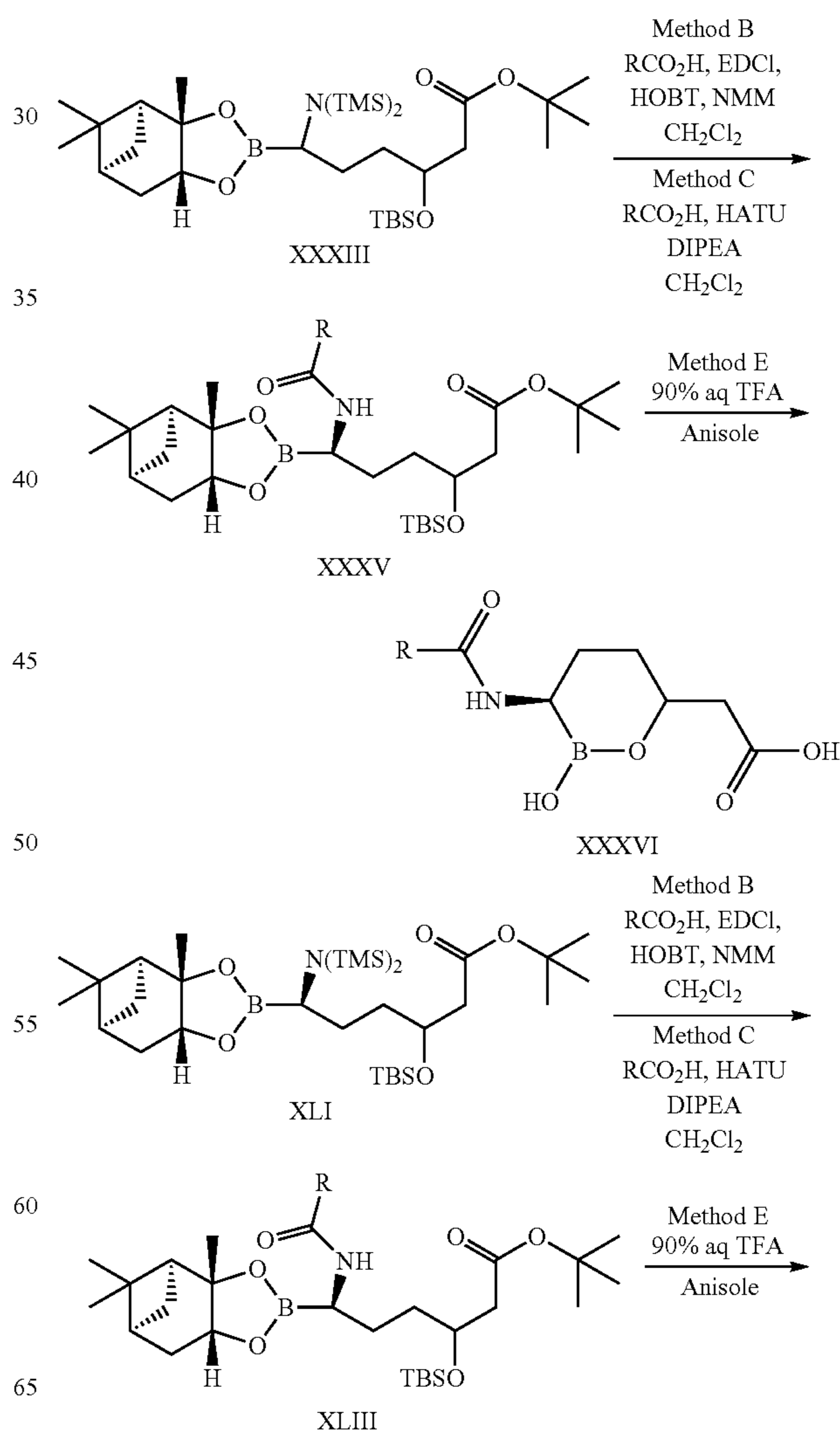
Scheme 9
