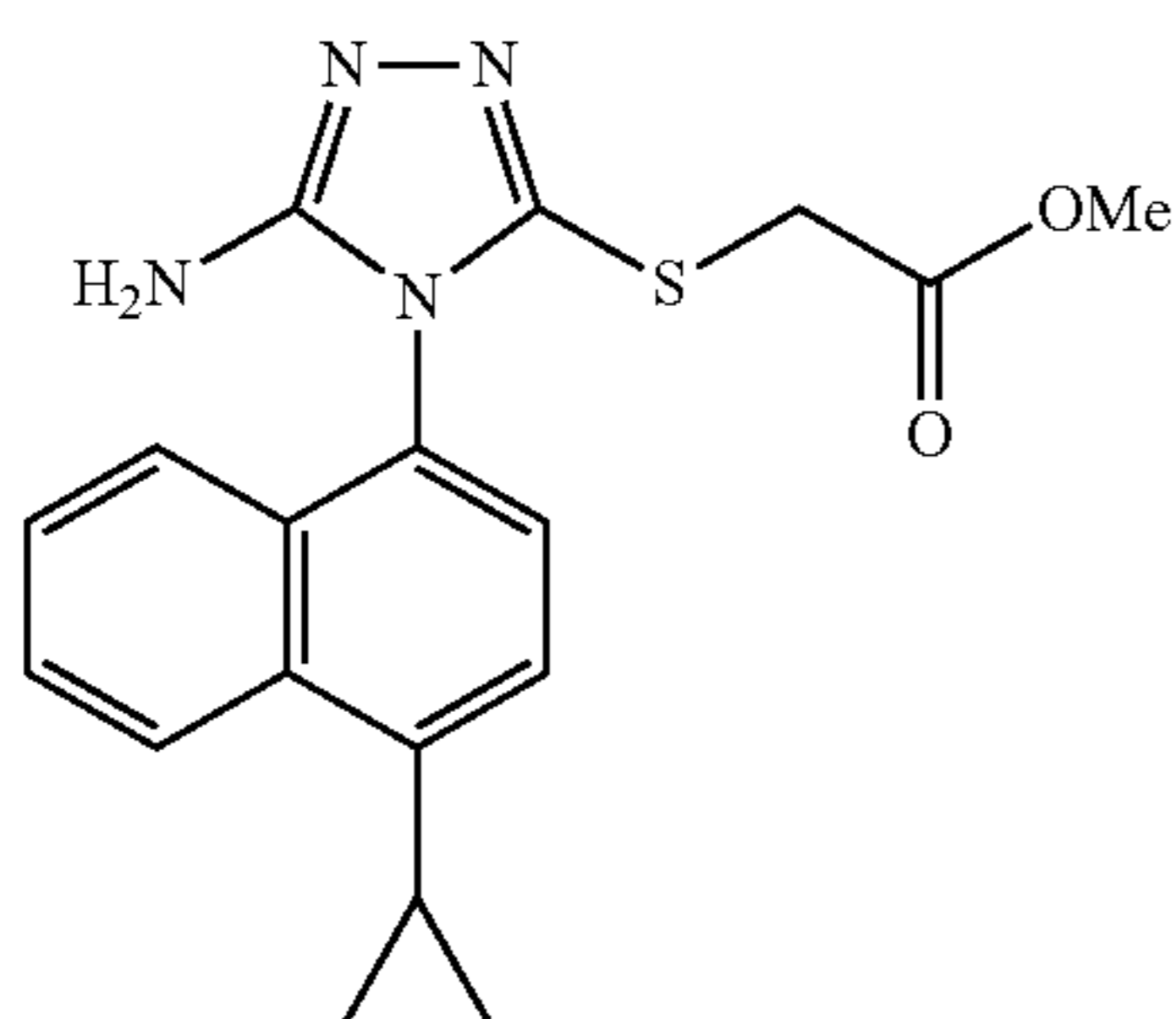
Methyl 2-(5-amino-4-(1-cyclopropylnaphthalen-4-yl)-4H-1,2,4-triazol-3-ylthio)acetate
