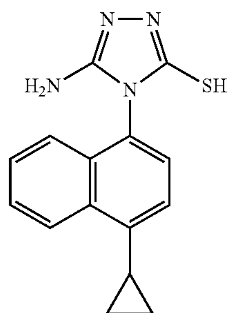
5-Amino-4-(1-cyclopropylnaphthalen-4-yl)-4H-1,2,4-triazole-3-thiol
