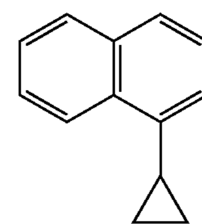
1-Cyclopropyl-naphthalene
