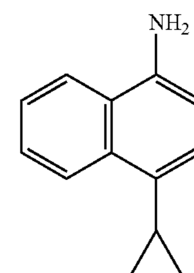
1-Amino-4-cyclopropyl-naphthalene
