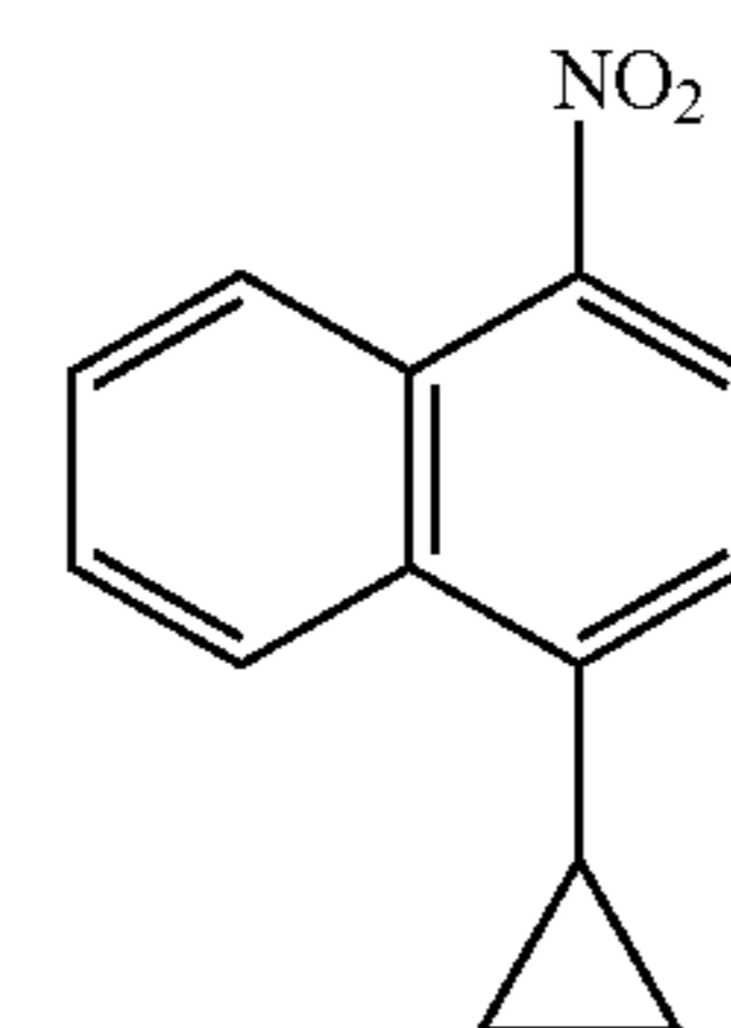
1-Cyclopropyl-4-nitronaphthalene
