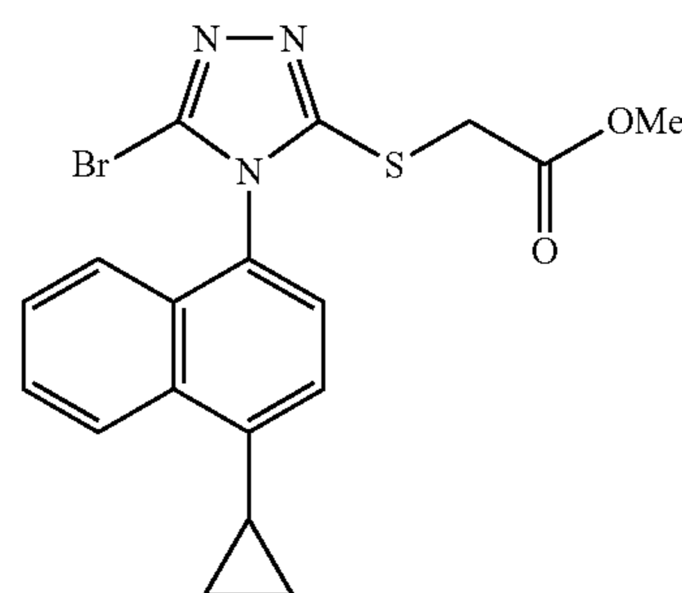
Methyl 2-(5-bromo-4-(1-cyclopropylnaphthalen-4-yl)-4H-1,2,4-triazol-3-ylthio)acetate
