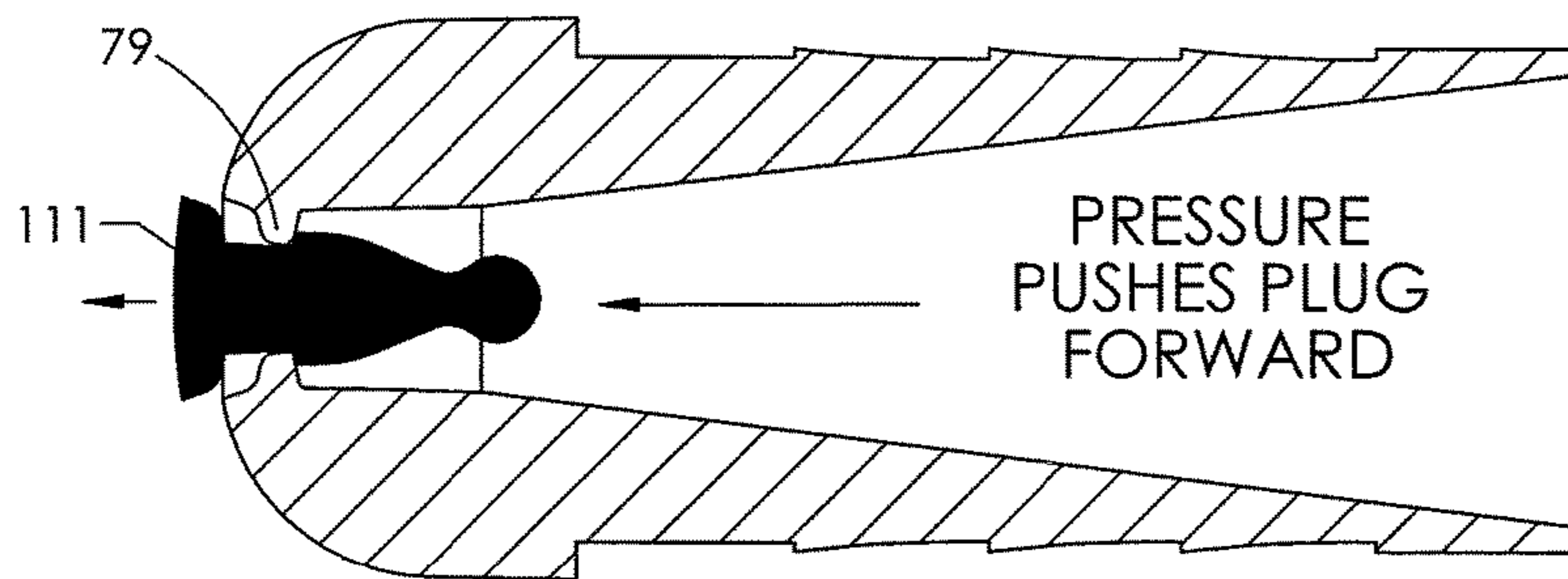
DURING INJECTION TOP VIEW CROSS-SECTION
