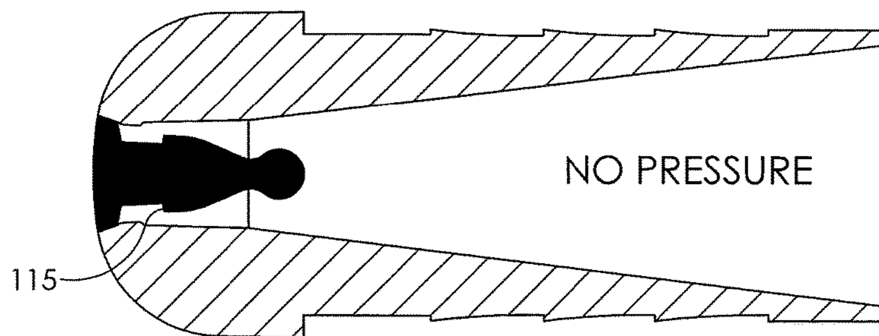
PRIOR TO USE FRONT VIEW CROSS-SECTION
