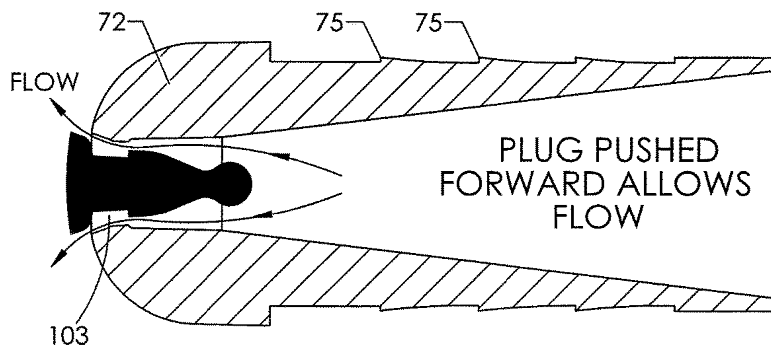
DURING INJECTION FRONT VIEW CROSS-SECTION
