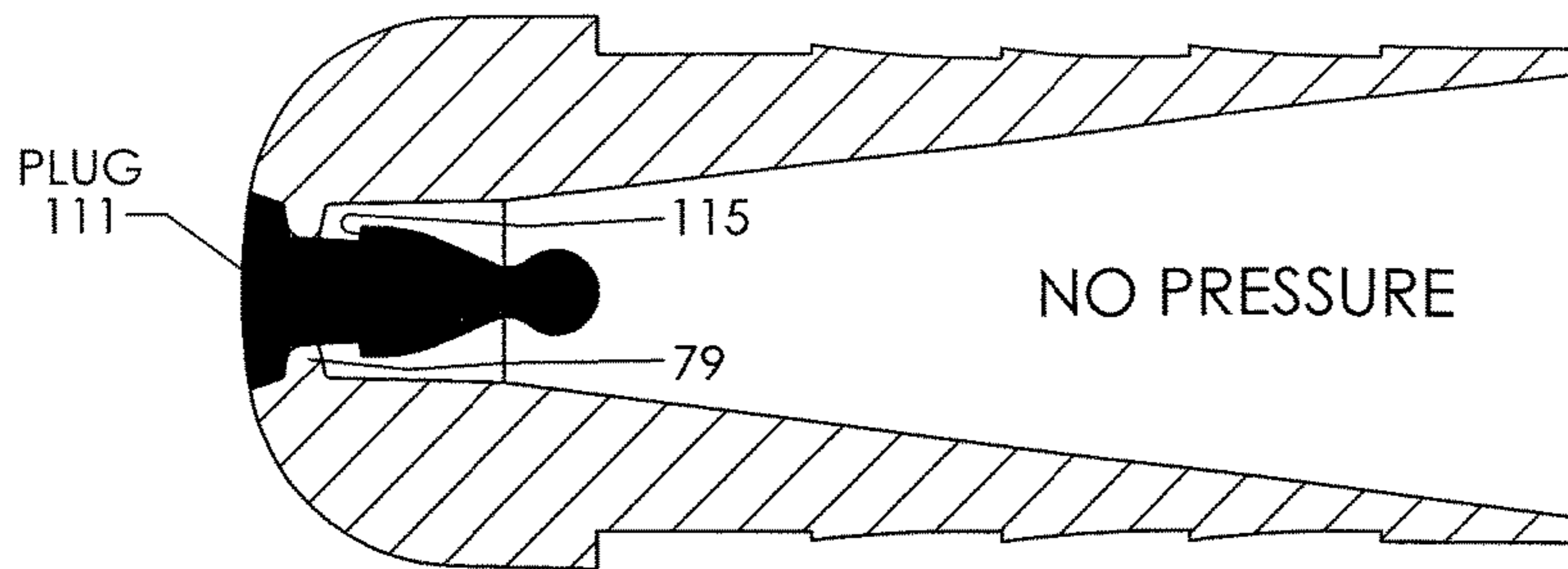
PRIOR TO USE TOP VIEW CROSS-SECTION
