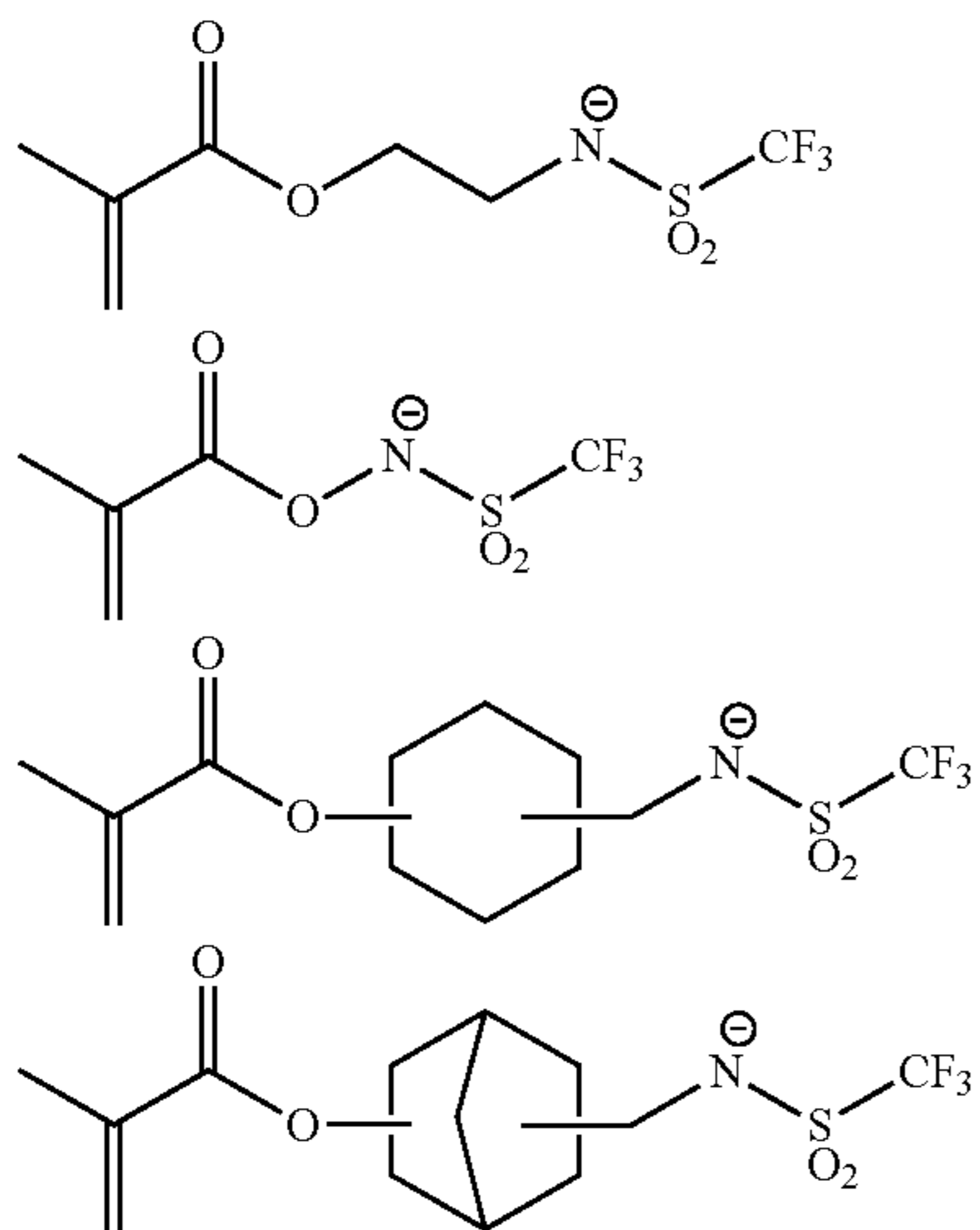
Chemical Formula 53
