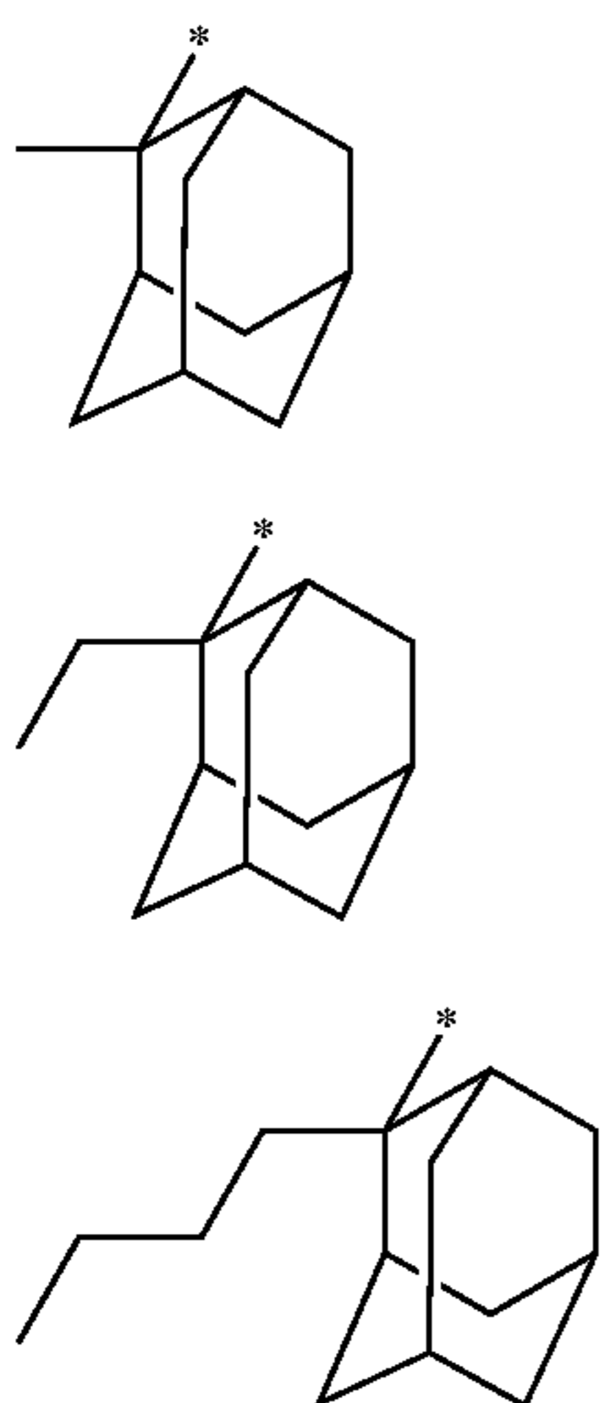
Chemical Formula 6
