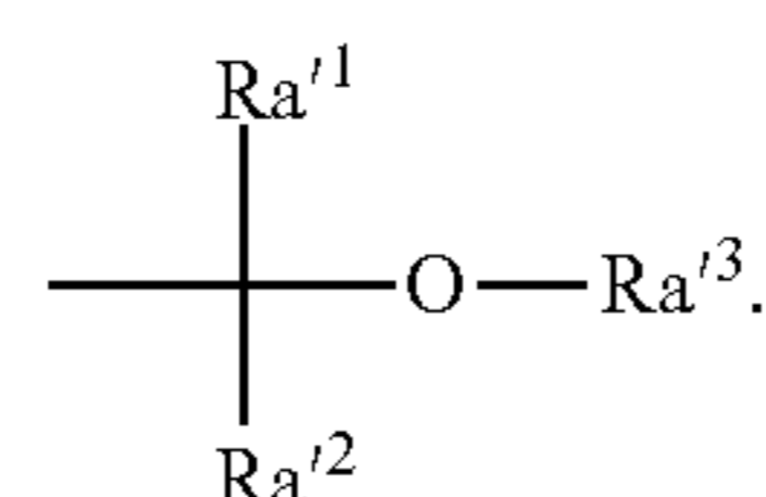
Chemical Formula 3
