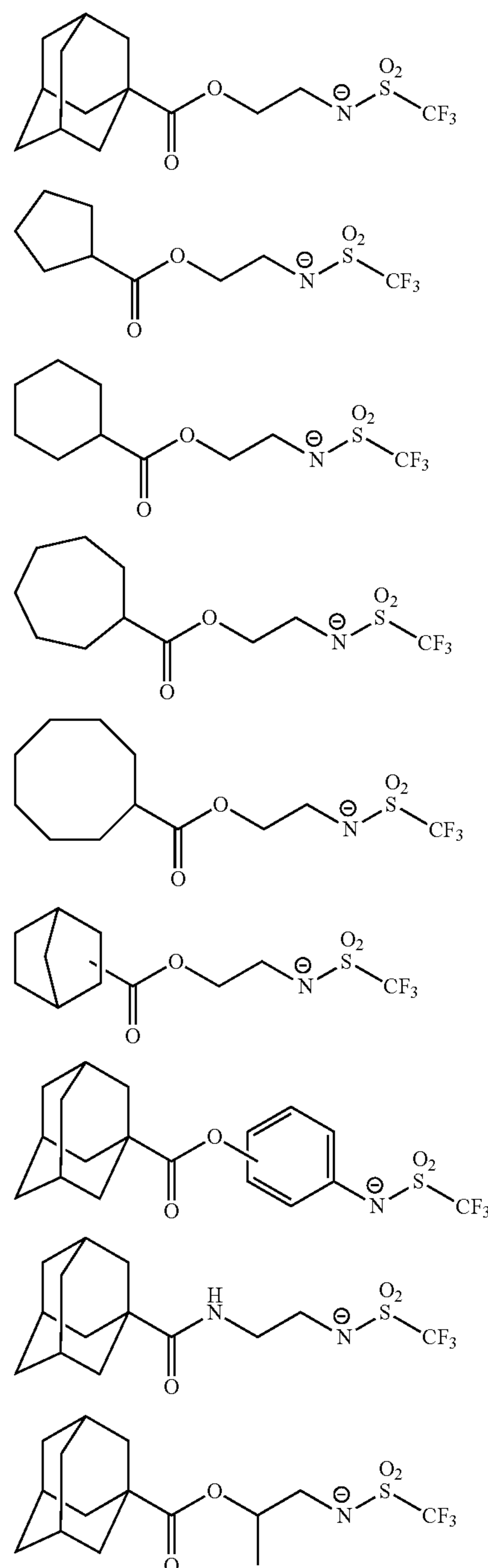
Chemical Formula 52
