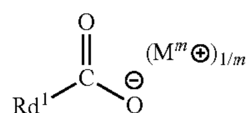
Chemical Formula 49
