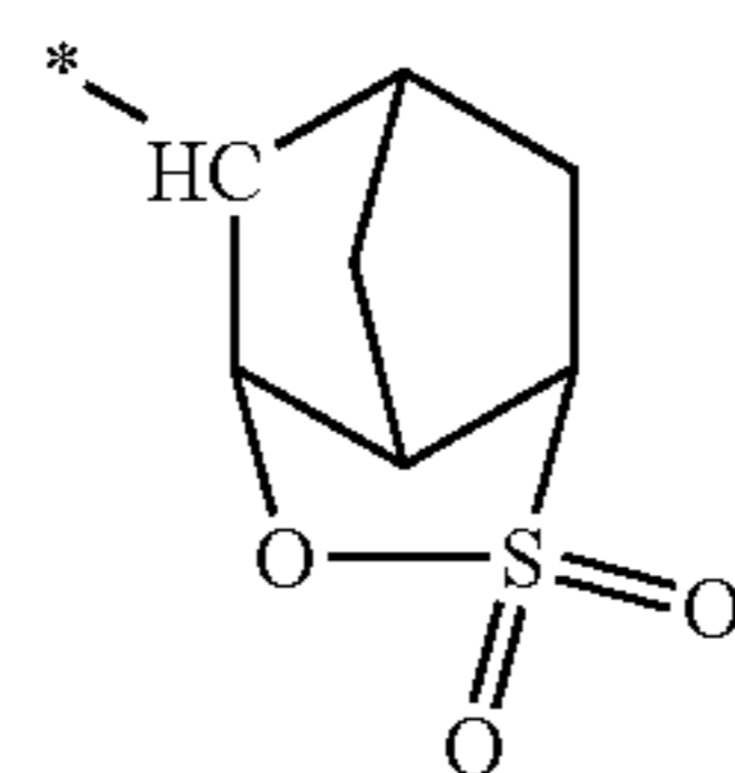
Chemical Formula 21
