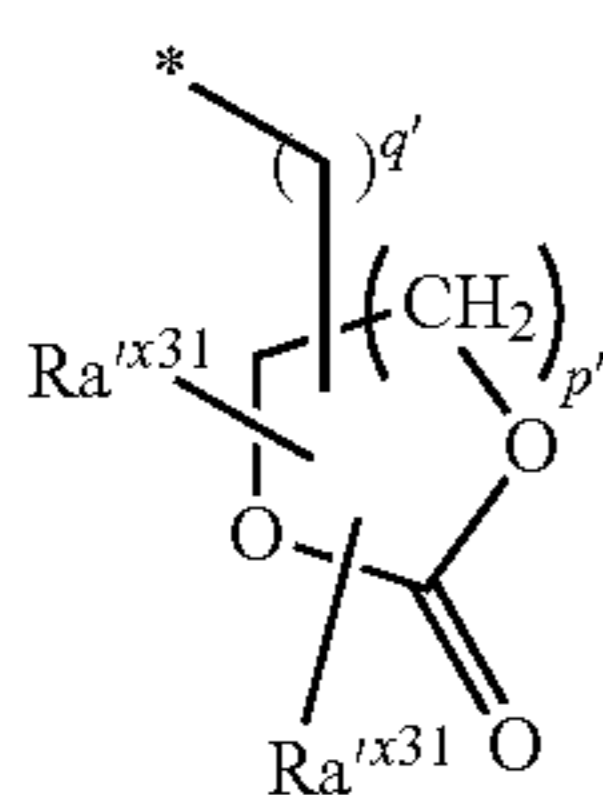
Chemical Formula 24
