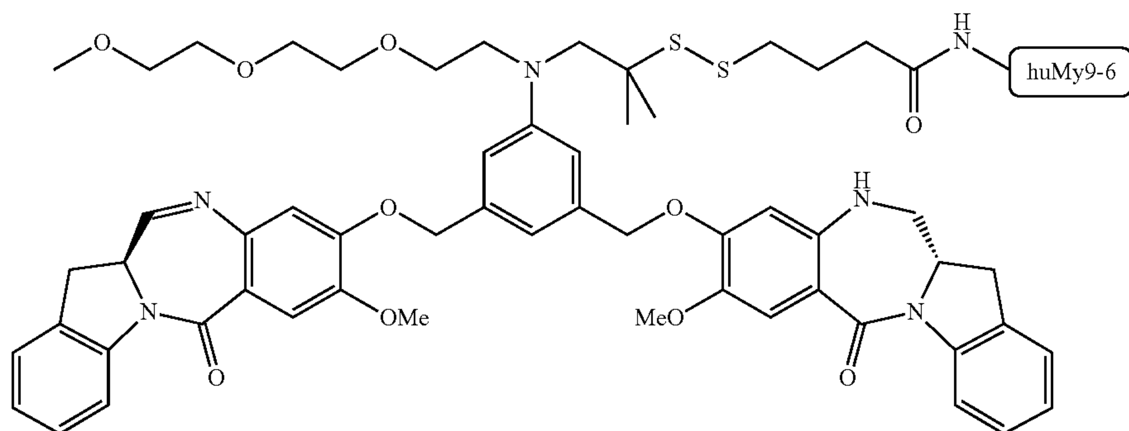
huMy9-6-SPDB-1f
