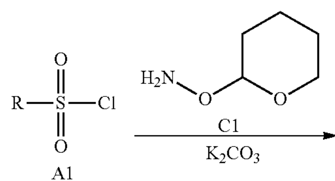
Scheme C. General Synthesis of Intermediate N-(tetrahydro-pyran-2-yloxy)sulfonamides.
