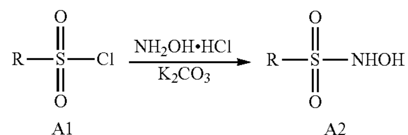
Scheme A. General Synthesis of N-Hydroxysulfonamides.
