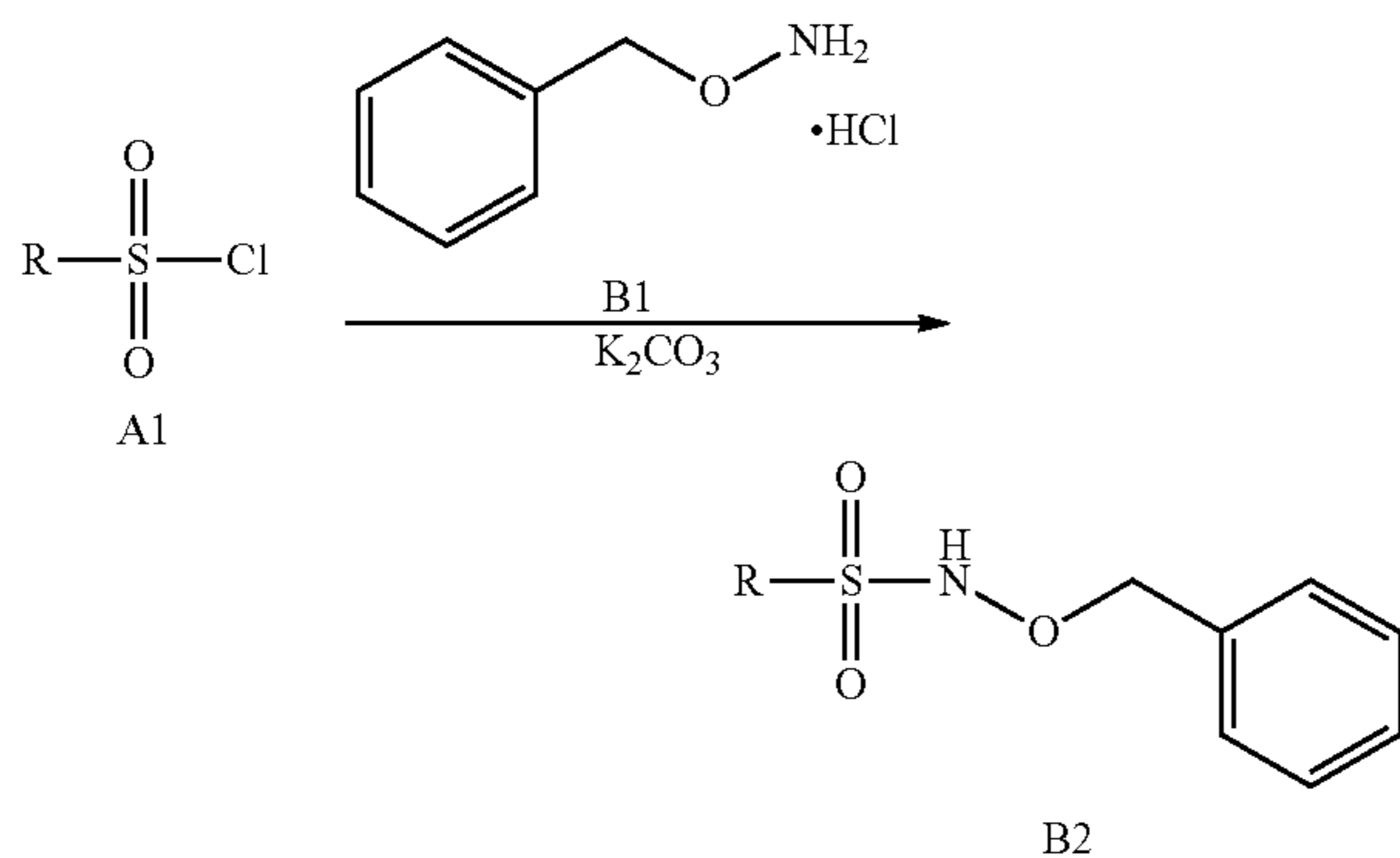
Scheme B. General Synthesis of Intermediate N-Benzyloxysulfonamides.
