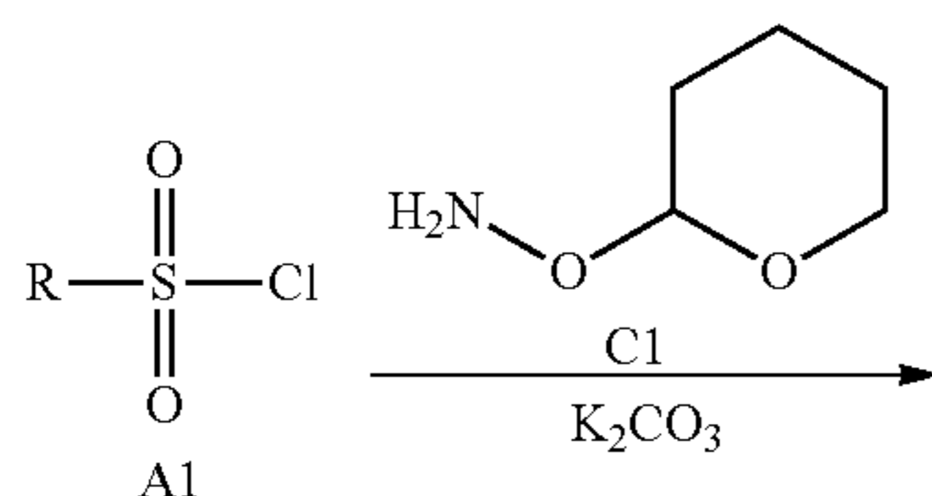
Scheme C. General Synthesis of Intermediate N-(tetrahydro-pyran-2-yloxy)sulfonamides.
